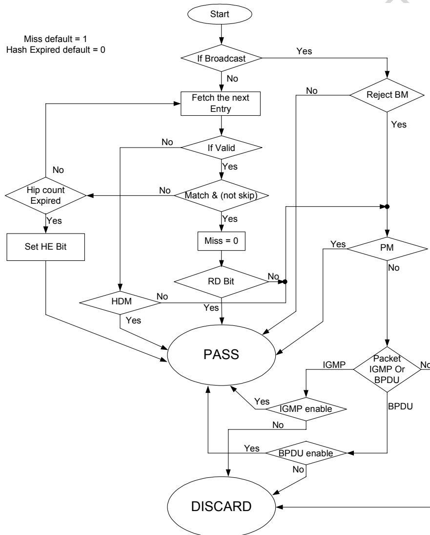
Figure 49: Address Filtering Process
