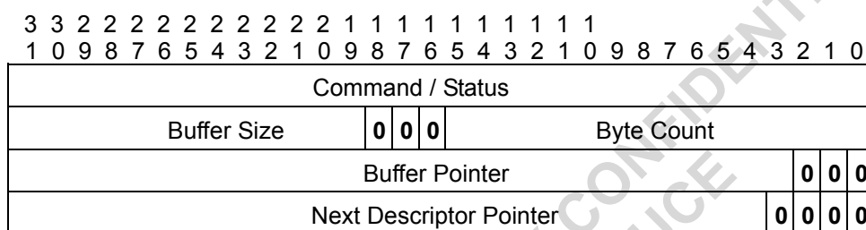
Figure 44: Ethernet Rx DMA Descriptor
