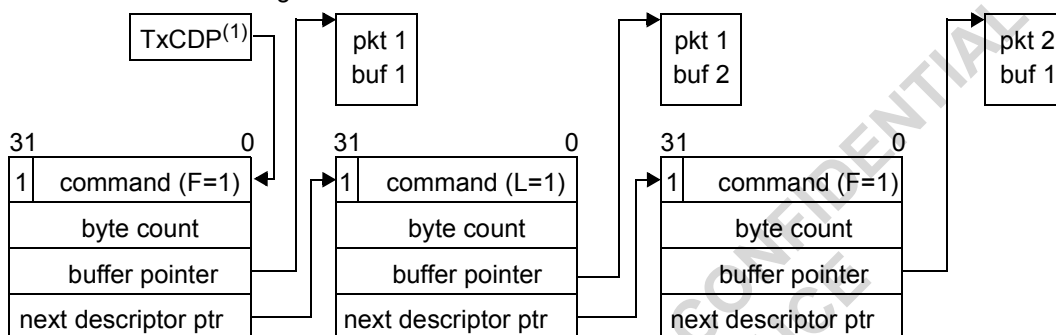
Figure 40: Ethernet Packet Transmission Example
