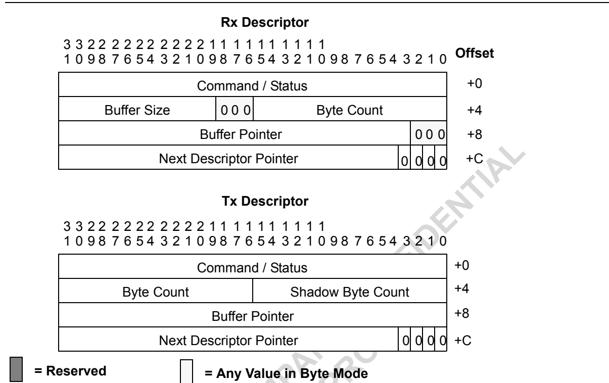
Figure 70: SDMA Descriptor Format
