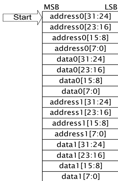
Figure 81: Serial ROM Data Structure
