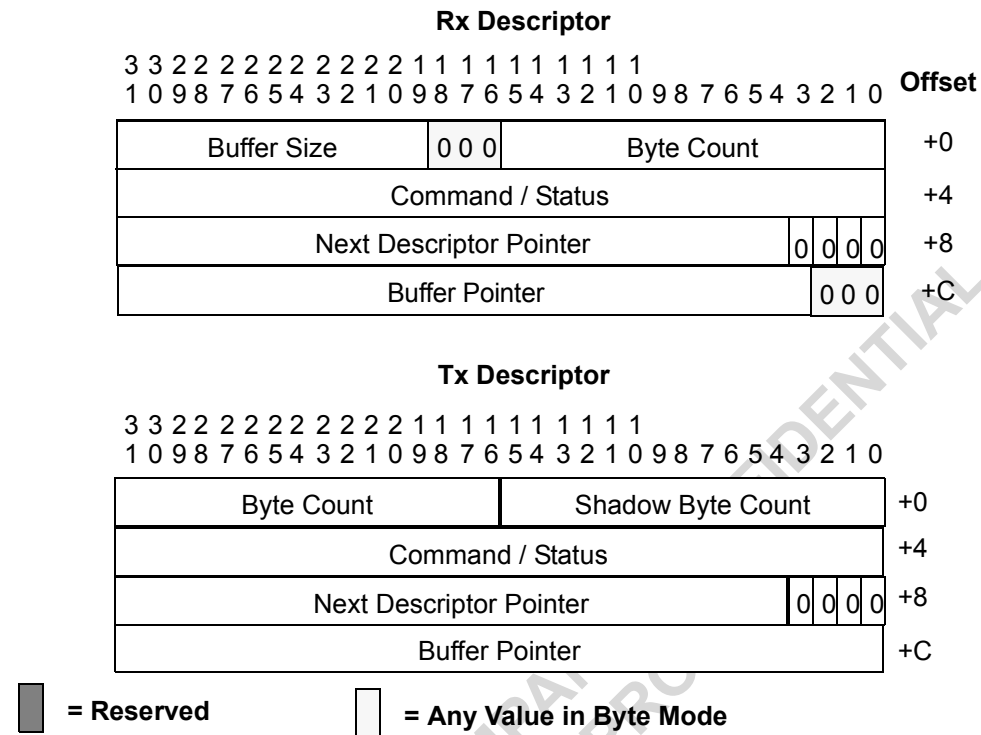
Figure 71: SDMA Descriptor Word Swapped Format
