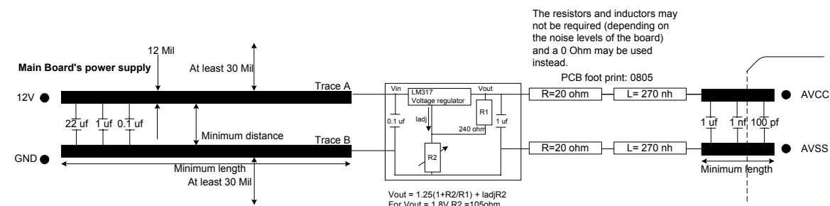
Figure 86: PLL Layout Guideline for Backplane Layout
