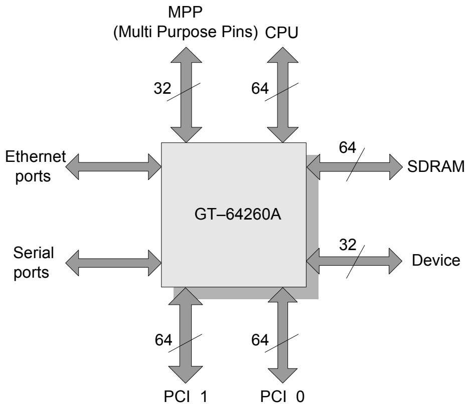
Figure 1: GT-64260 Interfaces
