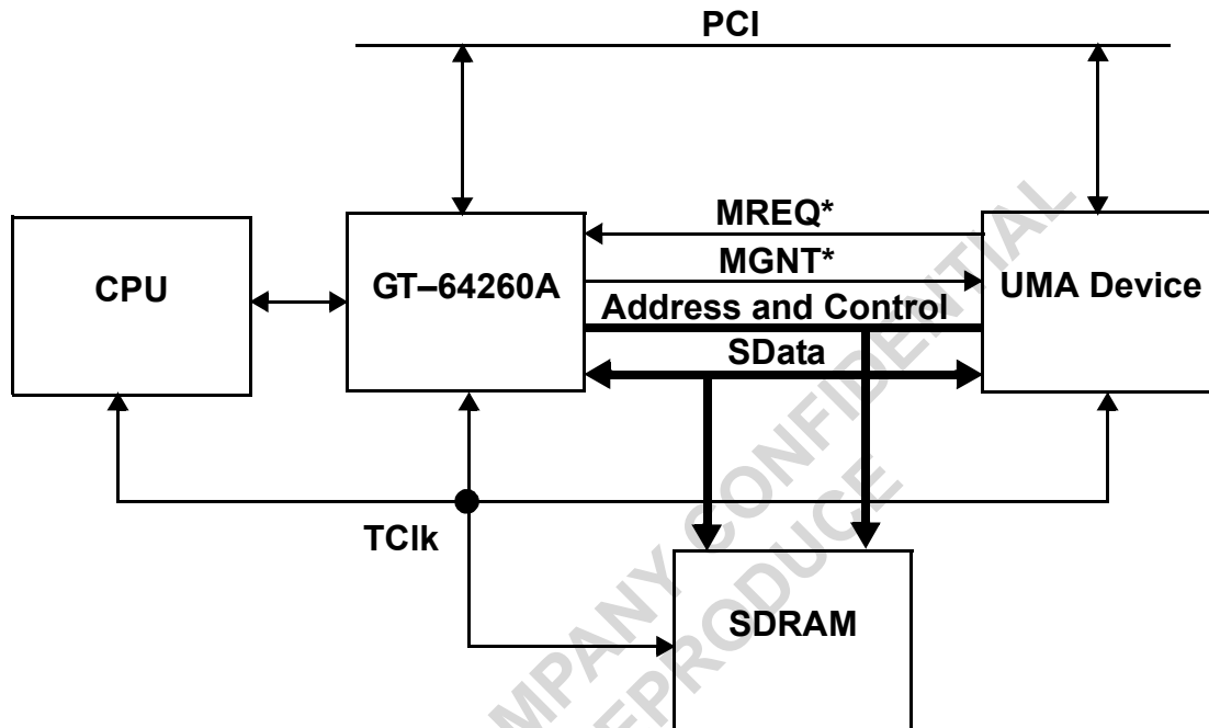
Figure 20: UMA Device and GT-64260A Sharing SDRAM
