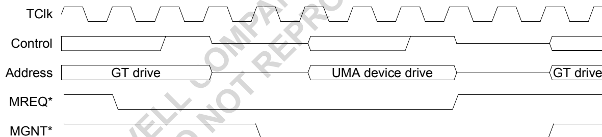
Figure 22: Handing the Bus Over
