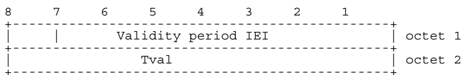
Figure 10.5/GSM 04.xx: Validity period information element
