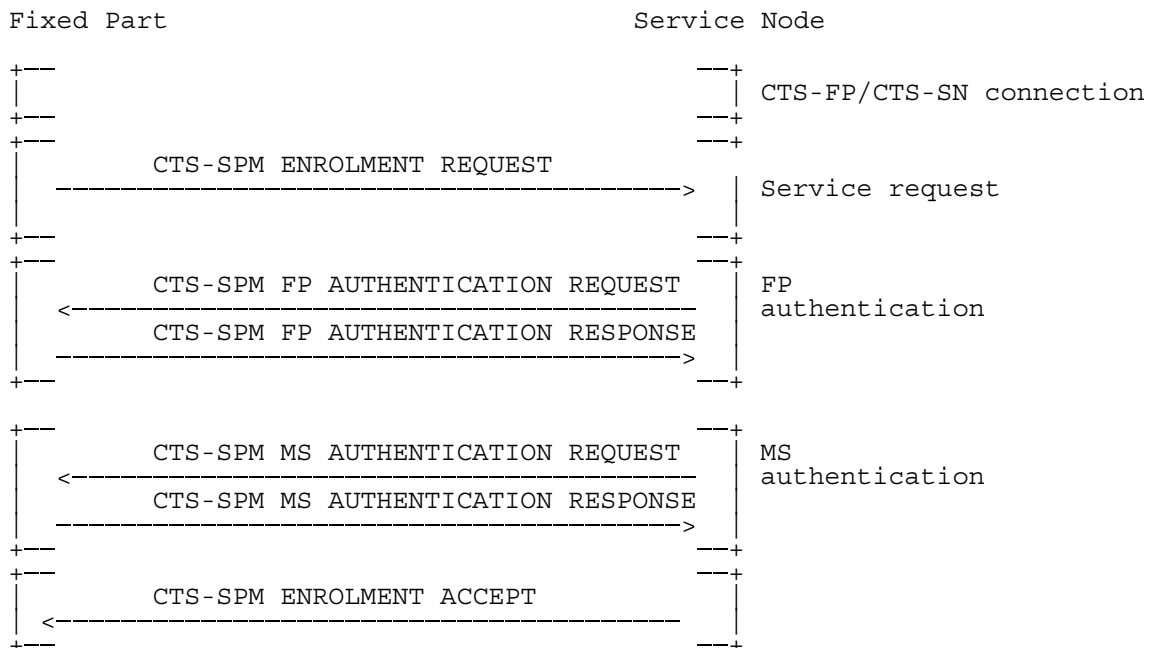
Figure 5.2/GSM 04.xx: CTS-SPM Enrolment
