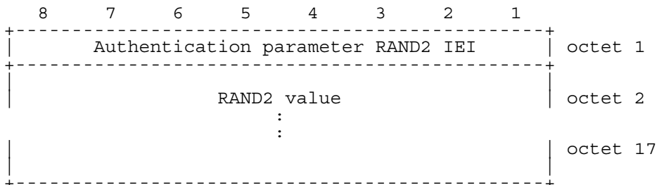
Figure 10.x/GSM 04.xx: Authentication Parameter RAND2 information element
