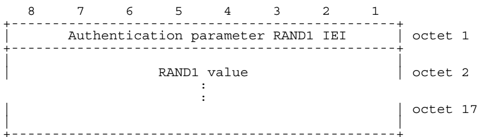
Figure 10.x/GSM 04.xx: Authentication Parameter RAND1 information element
