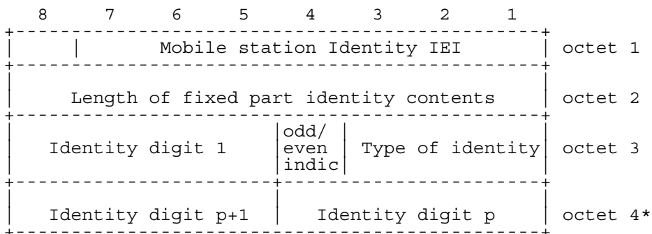
Figure 10.5/GSM 04.xx: Mobile station Identity information element
