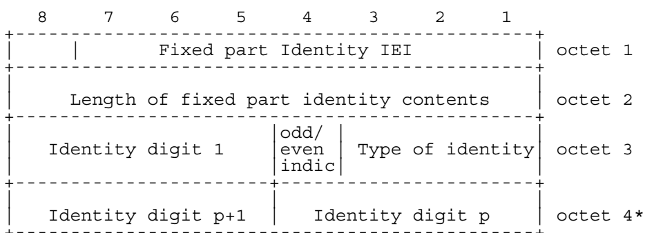
Figure 10.5/GSM 04.xx Fixed part Identity information element
