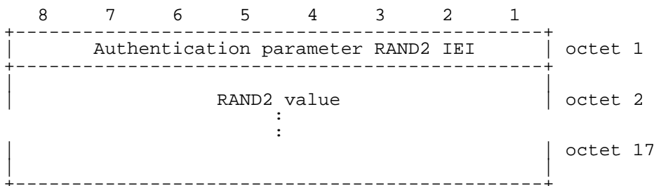
Figure 10.x/GSM 04.xx: Authentication Parameter RAND2 information element
