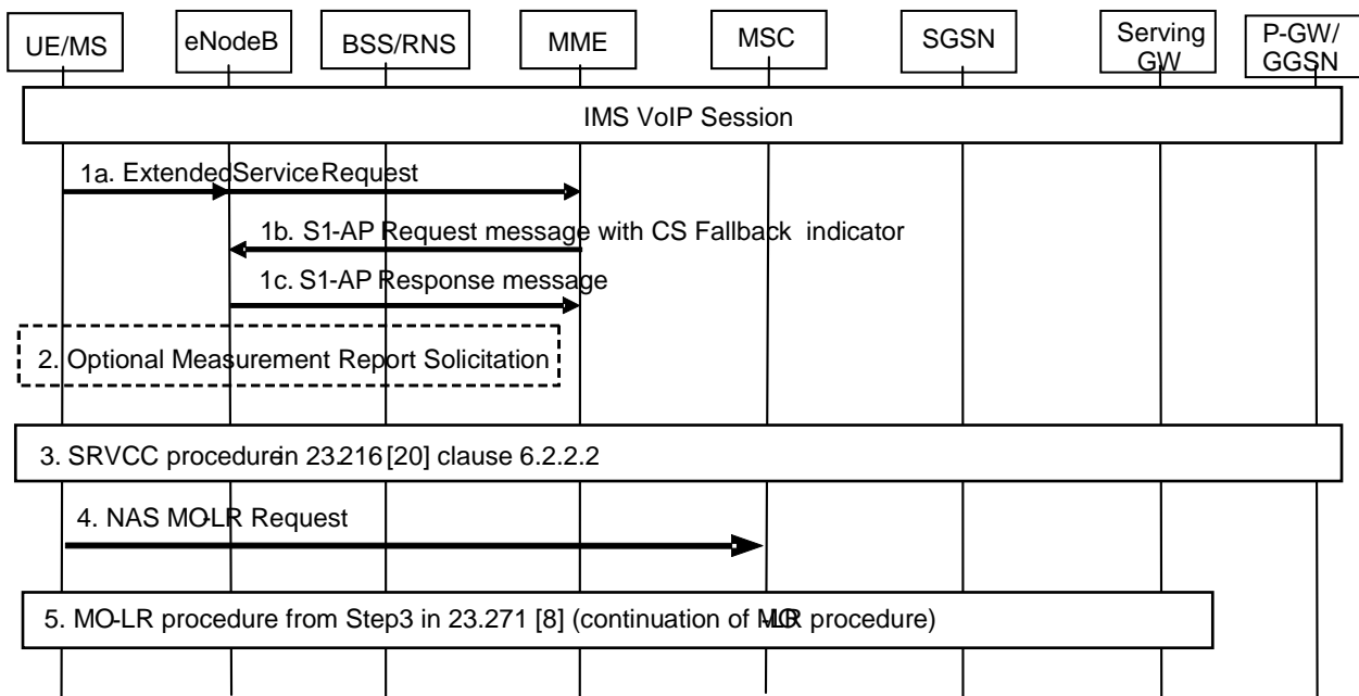
Figure 8.3.1.2-1: MO-LR Request in E-UTRAN while UE is in IMS VoIP session
