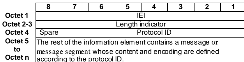
Figure 10.3.1: APDU IE
