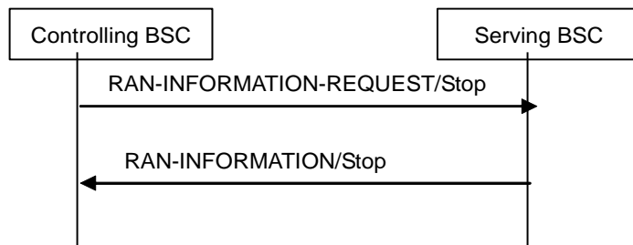
Figure 8c.2.2.3: RAN Information Request/Stop Procedure
