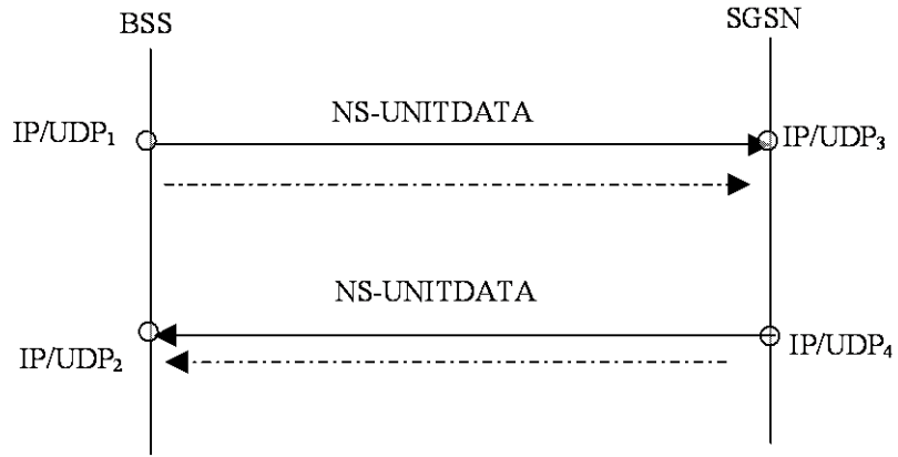
Figure B.4: Example 4 of NS entity not requesting change flow
