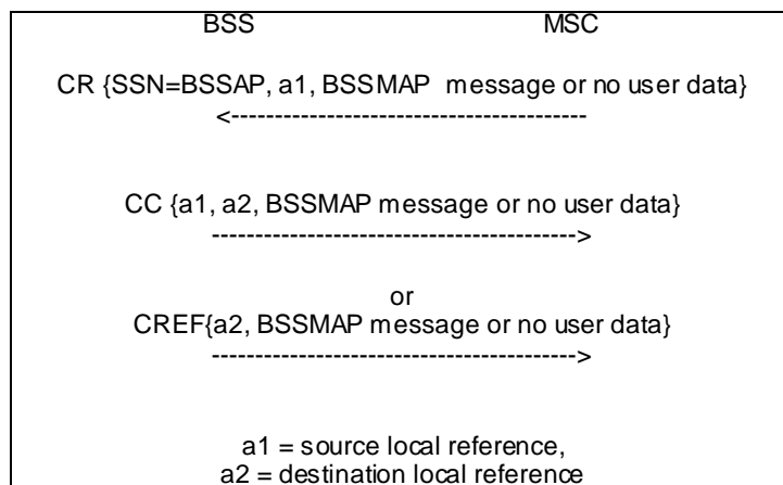
Figure 1: Set-up of SCCP connections on the first BSS/MSC interface
