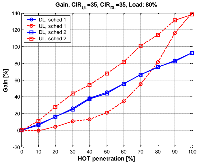
Figure 232i: CIR 35 dB, load factor: 80.0%, DL: 754.7 kbps/cell, UL: 754.7 kbps/cell.
