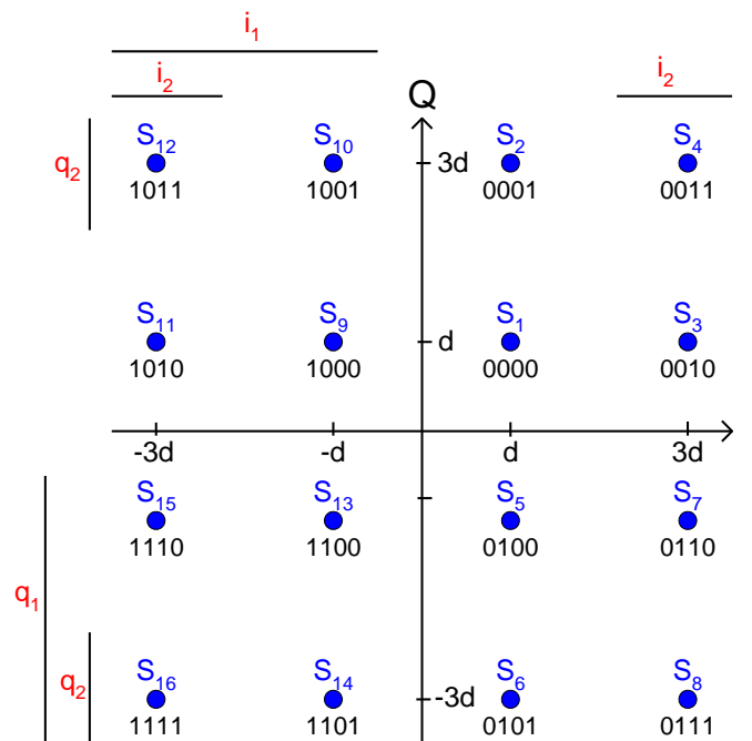
Figure 217: Signal constellation of 16-QAM modulation
