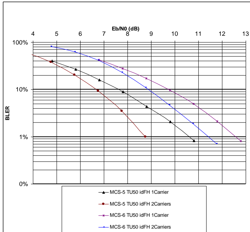
Figure 92: Receiver sensitivity simulation results for various MCS schemes for TU50 channel with Frequency Hopping
