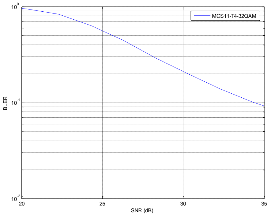
Figure 201: TU3iFH Sensitivity Performance (MCS-11)
