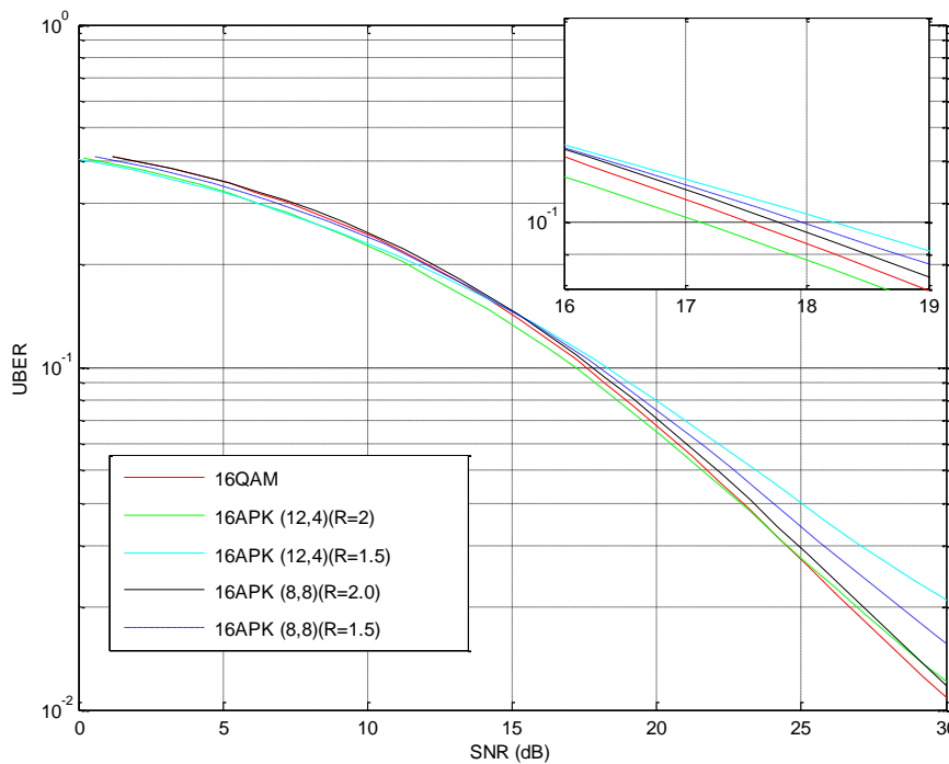
Figure 226: Uncoded BER of 16QAM, 16APK (12,4) & (8,8) Modulations
