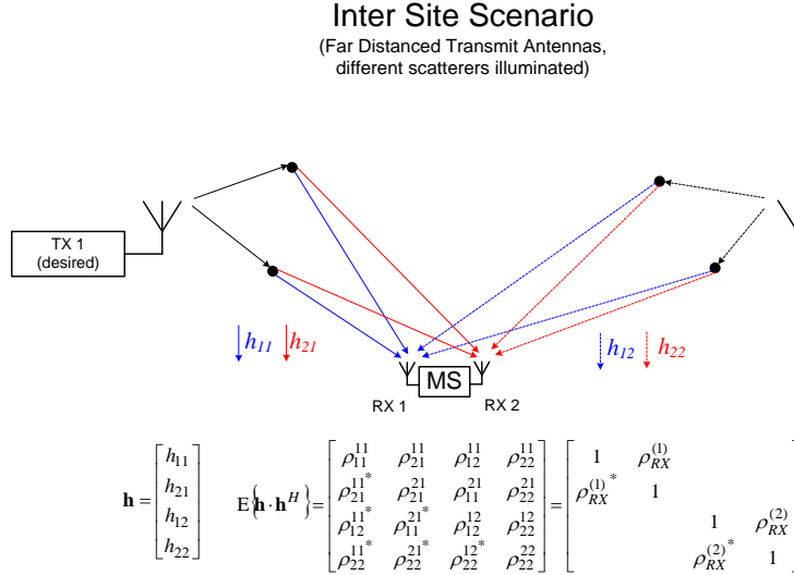
Figure 4: Inter-site interference scenario [13]
