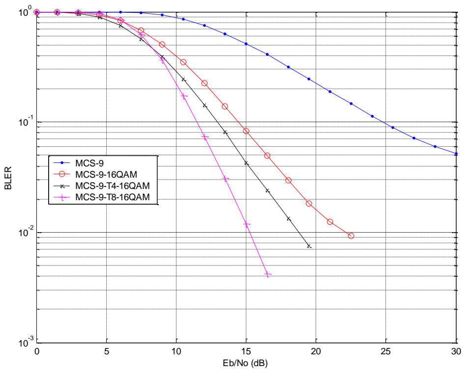
Figure 167: TU3iFH Sensitivity Performance (MCS-9)
