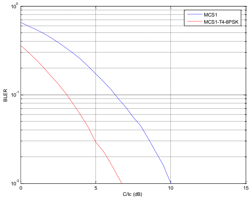
Figure 190: BLER Performance for MCS1 and MCS1-T4-8PSK in TU3iFH Channel
