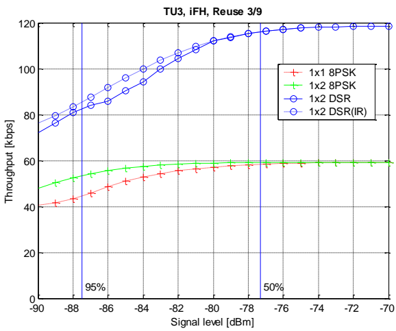
Figure 253: Throughput at Scenario 3 (3/9)
