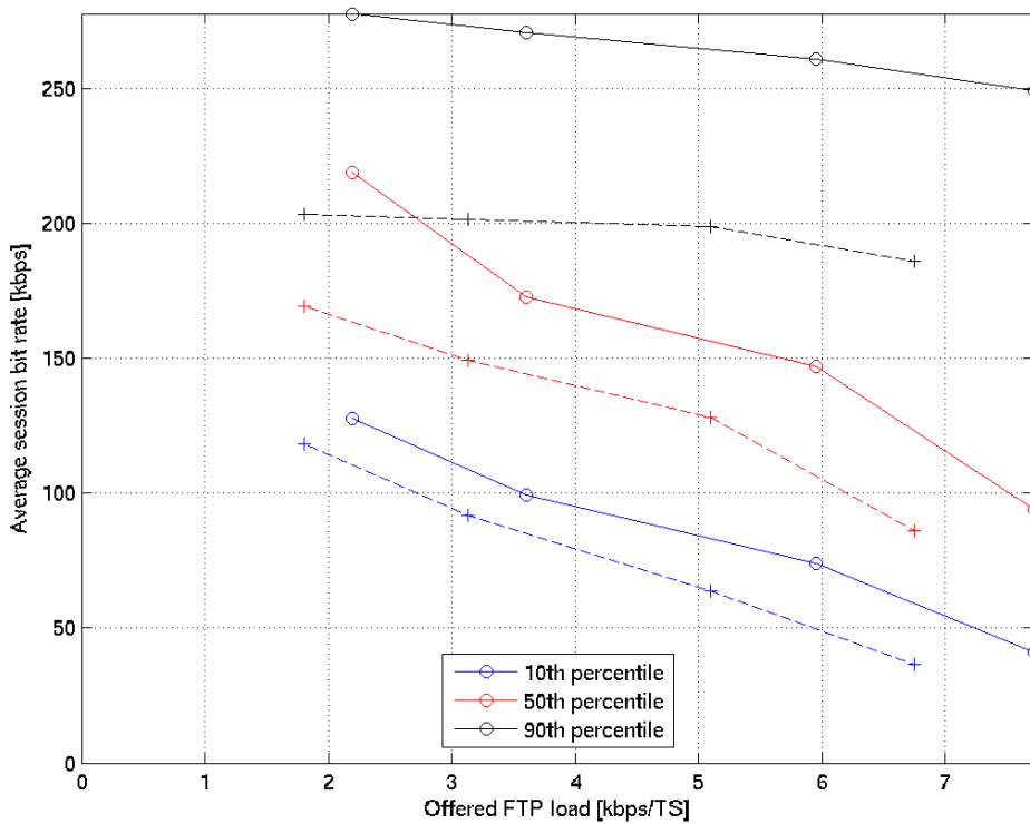
Figure 153a. Average session bit rate percentiles, 10th percentile (blue), 50th percentile (red), 90th percentile (black), as a function of offered FTP load, for EGPRS (dashed) and HOT level 2 (solid), in a 1-reuse.
