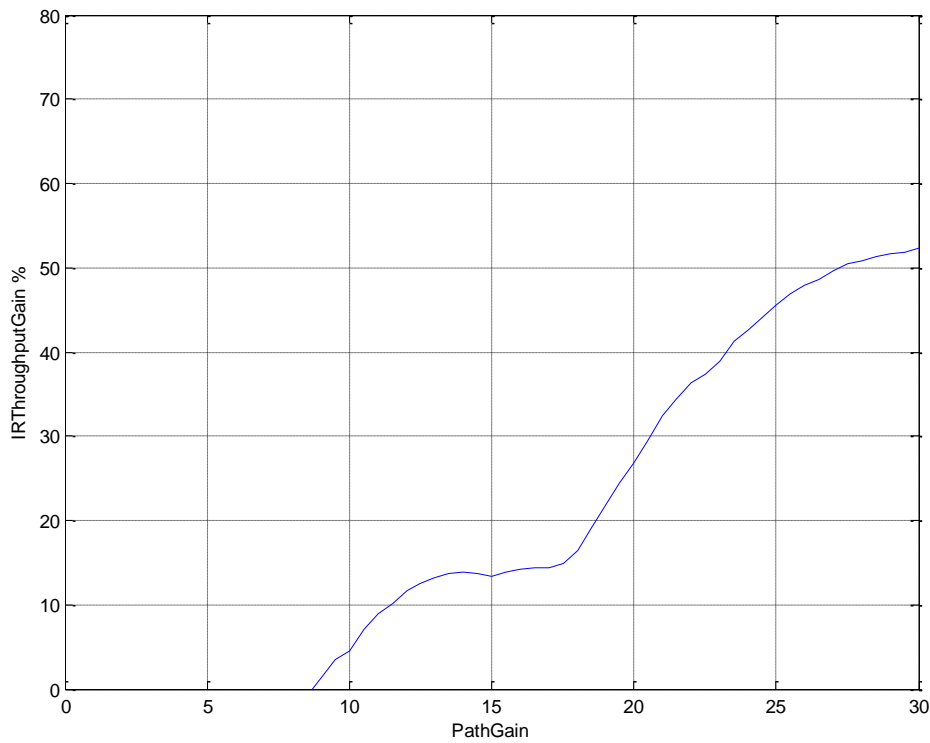
Figure 186: Throughput Performance Gain (%) of MCS9-T4-16QAM v MCS9 with IR for HT100km/h Non Hopping channel
