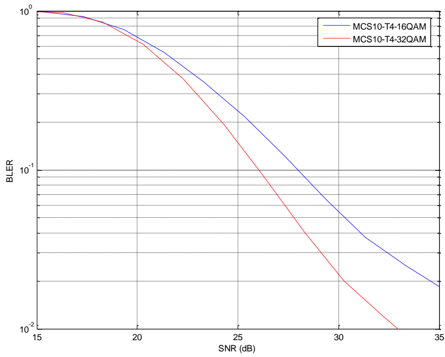
Figure 200: TU3iFH Sensitivity Performance (MCS-10)
