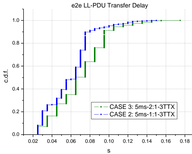
Figure 353: Case 3 ("5 ms TTI", 3 Tx) vs Case 2 ("5 ms TTI", 3 Tx, up to 1 RTTI block per TTI period)
