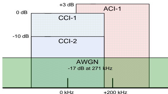
Figure 275: DTS-2 Link scenario for 1.2 times higher symbol rate
