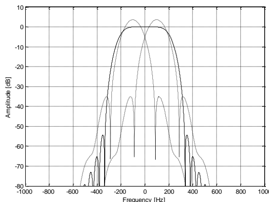
Figure 238: MDSR spectrum
