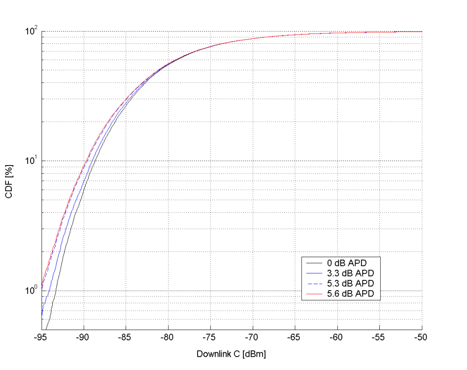
Figure 232a. Downlink distribution of C.
