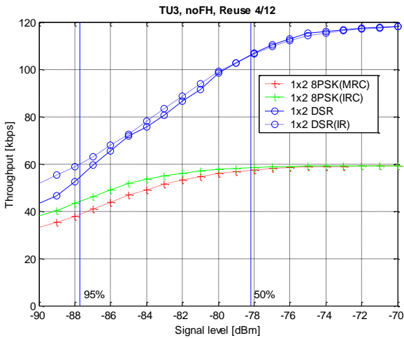
Figure 251: Throughput at scenario 1 (4/12)
