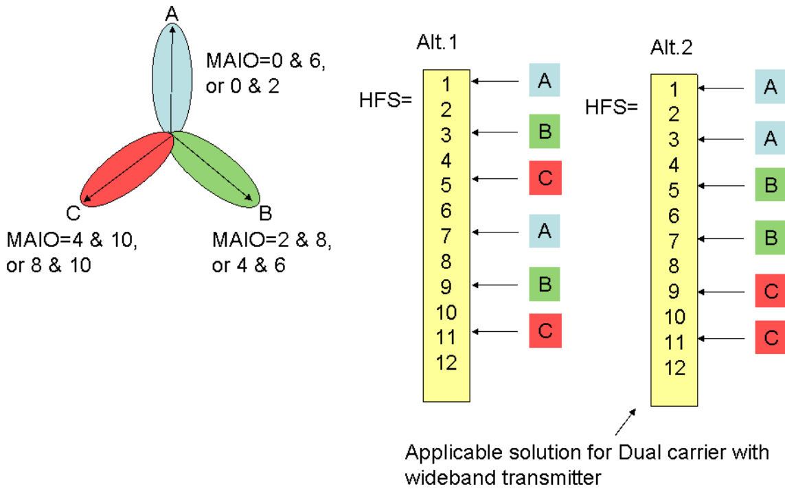
Figure 94: Different Mobile Allocation alternatives in a FLP network
