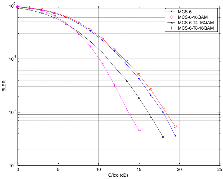
Figure C.2: TU50nH Co-Channel Performance (MCS-6)
