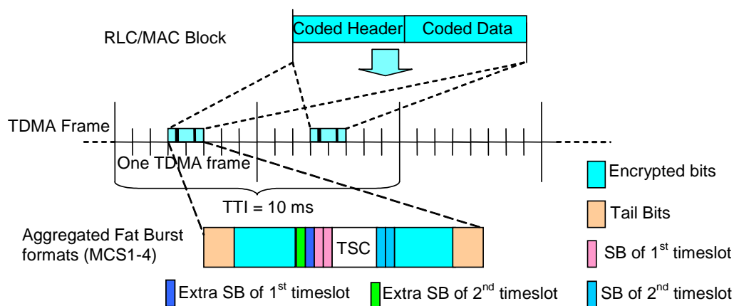
Figure 380: Normal Burst format after two timeslots aggregation for RTTI TBF
