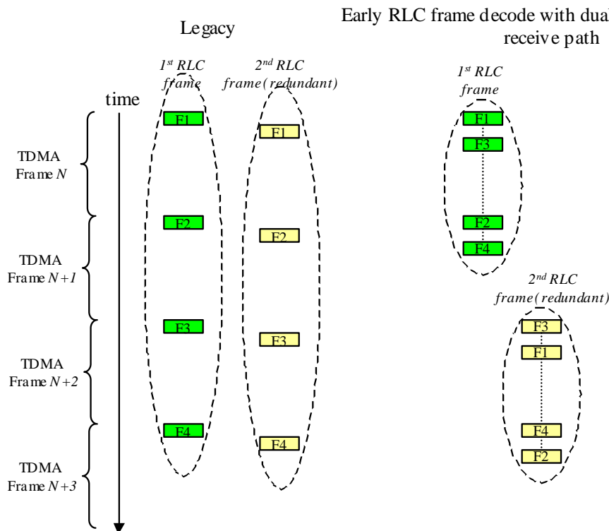
Figure 345: Early RLC frame decode with dual frequency/ single trx
