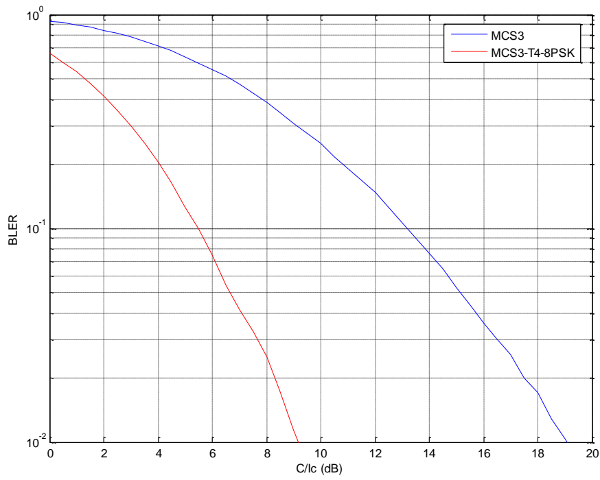
Figure 192: BLER Performance for MCS3 and MCS3-T4-8PSK in TU3iFH Channel
