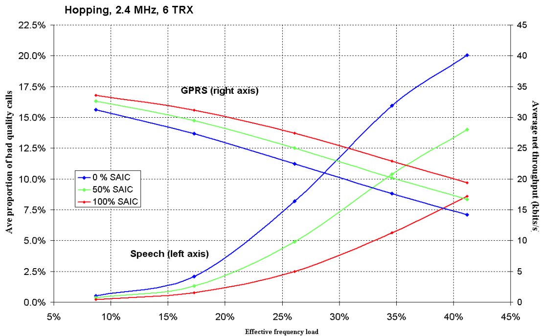
Figure 7.18: Speech and GPRS performance indicators for FTP/MMS data traffic.
