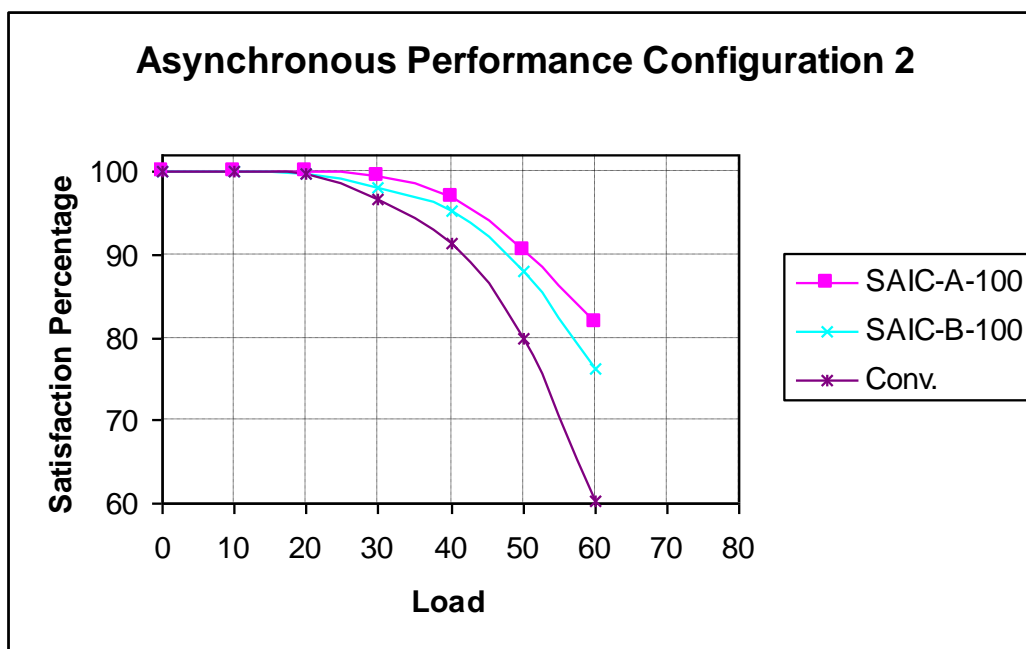
Figure 7.2. System performance for Configuration 2 – Asynchronous [8].
