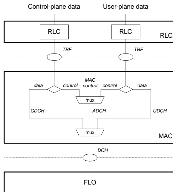
Figure 3: Logical Channels and Transport Channels
