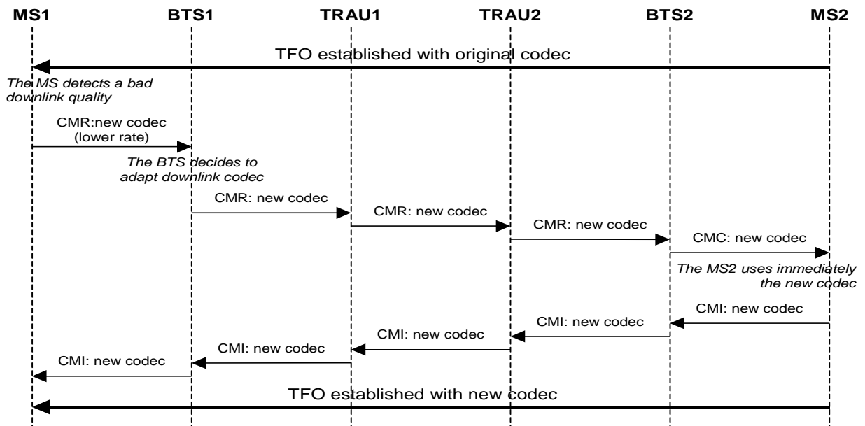
Figure C.1.2: Downlink Downgrading
