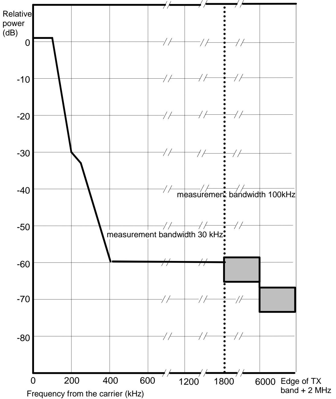
Figure A.3a: DCS 1 800 and PCS 1900 MS spectrum due to GMSK modulation
