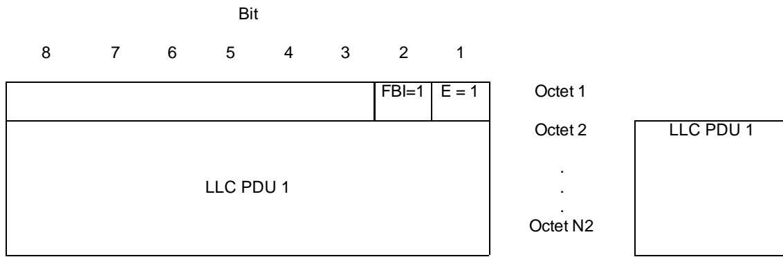
Figure B.10: Example for the case when a LLC PDU fills the RLC data block precisely.
