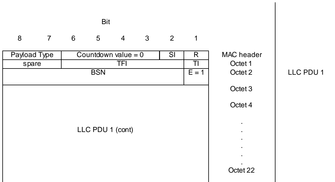
Figure B.6: Example when Length indicator (LI) can be omitted
