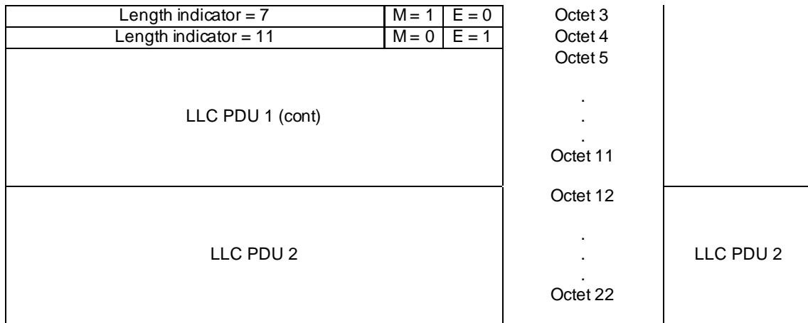
Figure B.3: Length indicator (LI) example
