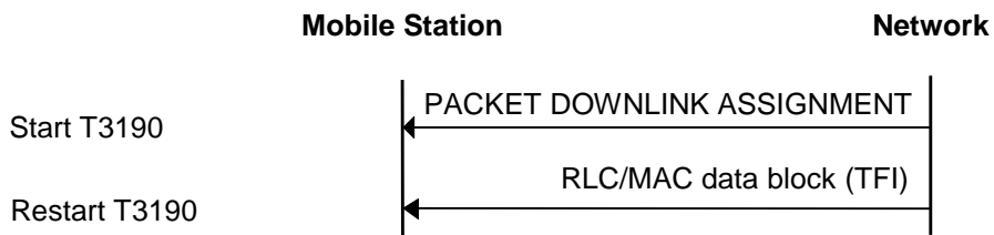
Figure C.1: Message Sequence Diagram for one phase packet access
