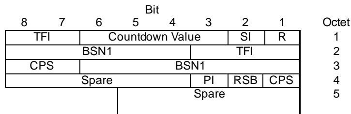
Figure 10.3a.4.2.1: EGPRS uplink RLC data block header (FANR not activated) for MCS-5 and MCS-6
