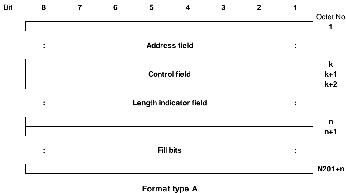
Figure 1 (sheet 1 of 3): General frame formats
