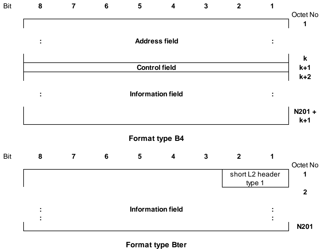
Figure 1 (sheet 3 of 3): General frame formats
