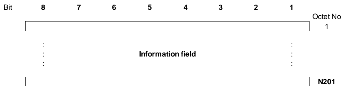
Figure 1 (sheet 2 of 3): General frame formats
