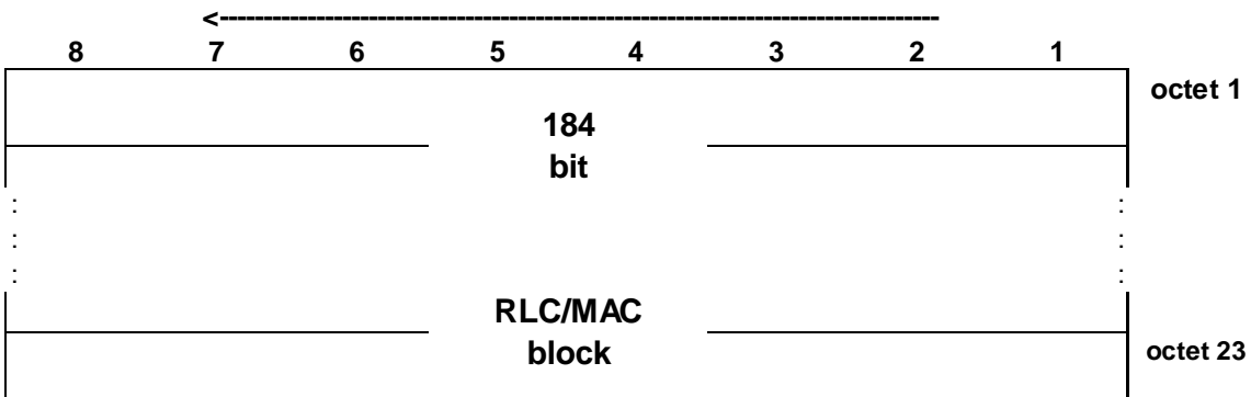
Figure 7.5: PBCCH/PCCCH downlink/PACCH blockformat
