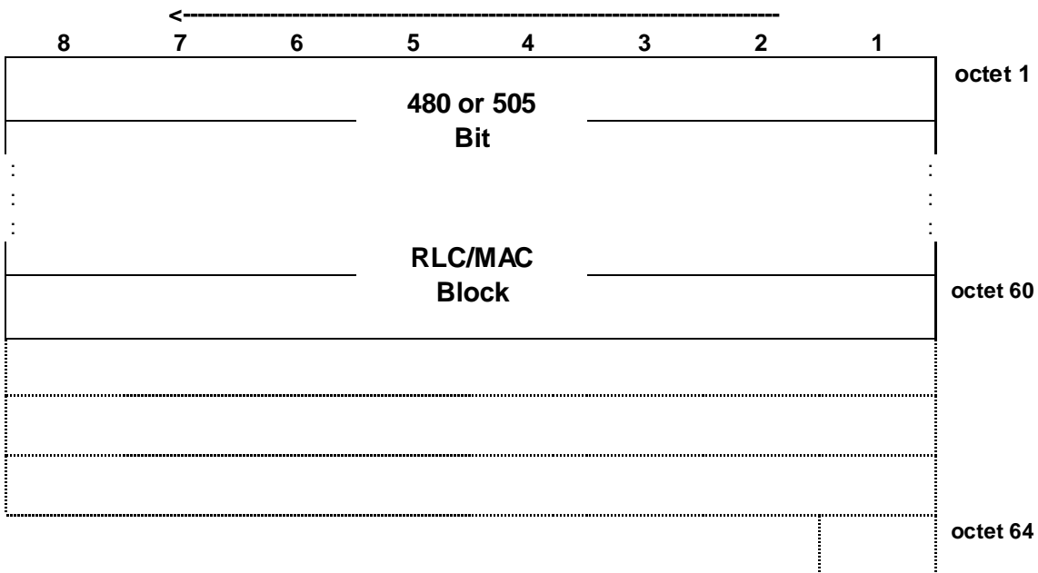
Figure 7.6.35.1: PDTCH block type 35 (DBS-5) format
