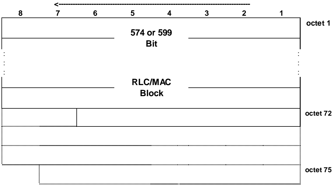
Figure 7.6.28.1: PDTCH block type 28 (DAS-6) format
