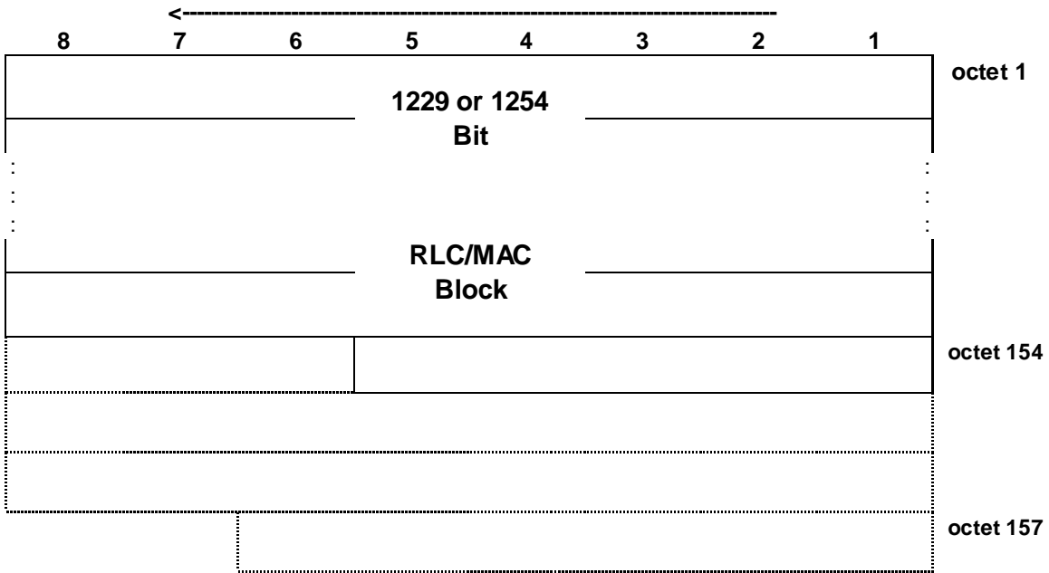
Figure 7.6.38.1: PDTCH block type 38 (DBS-8) format
