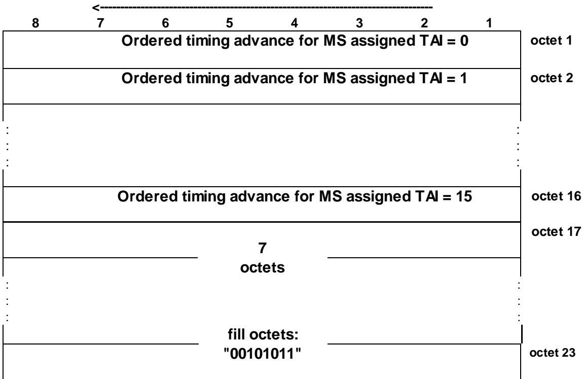
Figure 7.8: PTCCH downlink block format
