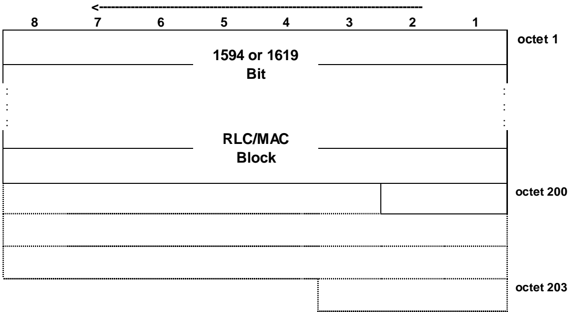
Figure 7.6.18.1: PDTCH block type 18 (UAS-11) format
