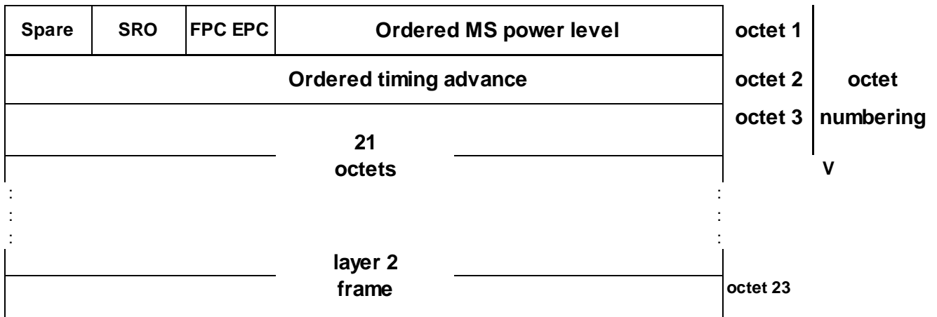
Figure 7.1.1: SACCH downlink block format for MS operating in A/Gb mode
