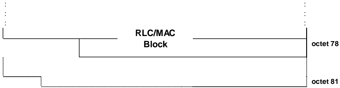
Figure 7.6.10.2: PDTCH block type 10 (MCS-6) downlink format
