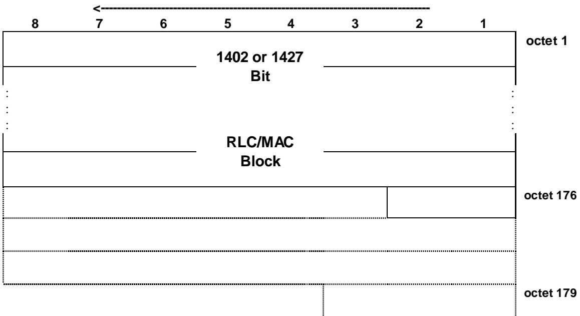
Figure 7.6.17.1: PDTCH block type 17 (UAS-10) format
