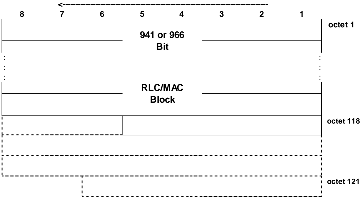
Figure 7.6.14.1: PDTCH block type 14 (UAS-7) format
