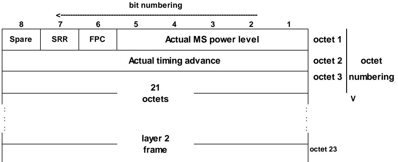
Figure 7.2.1: SACCH uplink block format for MS operating in A/Gb mode
