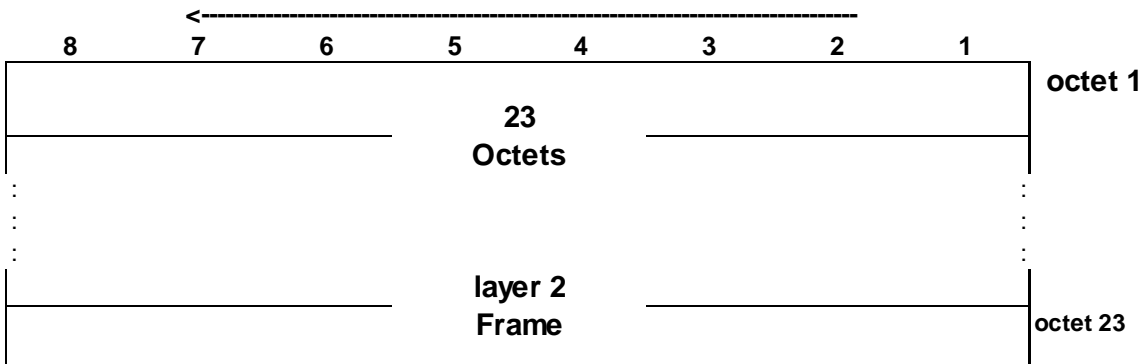
Figure 7.3.2.1: FACCH/SDCCH downlink block format for MS operating in A/Gb mode
