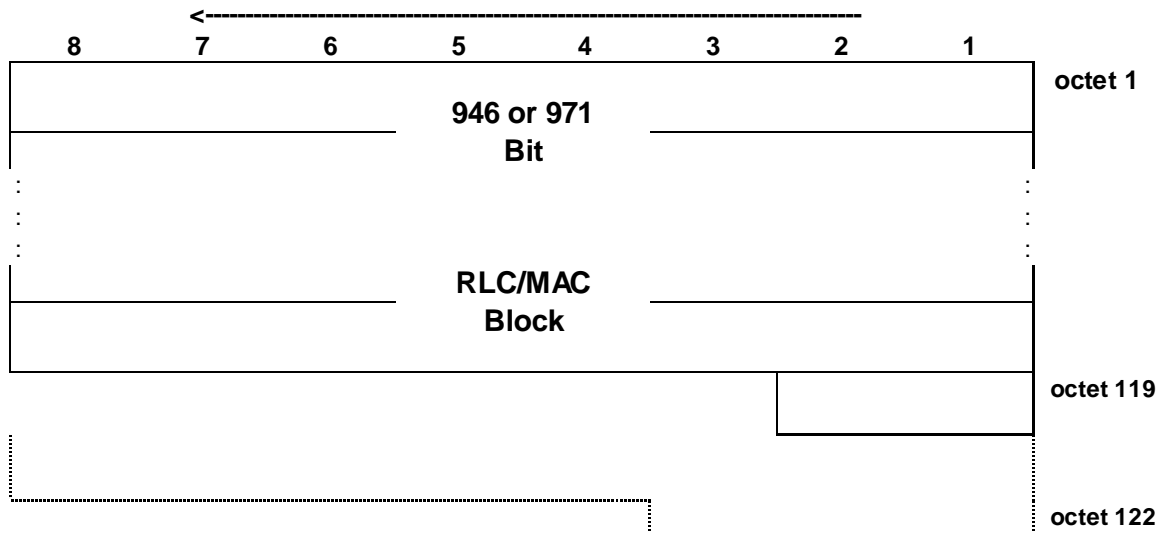
Figure 7.6.11.1: PDTCH block type 11(MCS-7) uplink format
