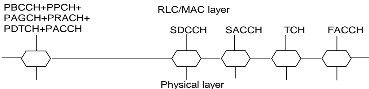
Figure 3.1.d: SAP between the physical layer and the RLC/MAC layer when the MS is operating in lu mode
