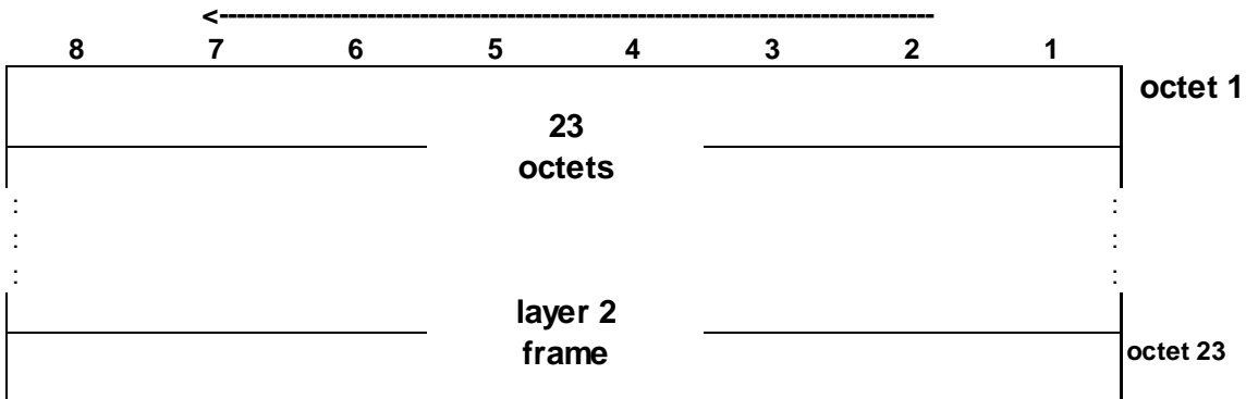
Figure 7.3.1: BCCH/CCCH/CBCH downlink block format
