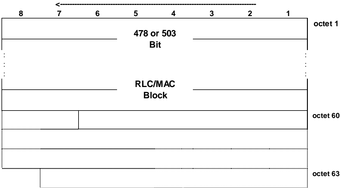
Figure 7.6.27.1: PDTCH block type 27 (DAS-5) format
