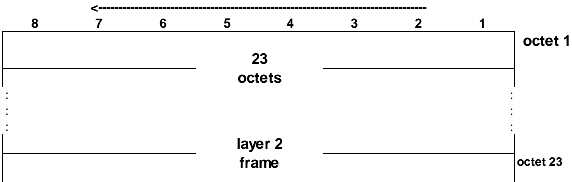
Figure 7.4.1: FACCH/SDCCH uplink block format for MS operating in A/Gb mode
