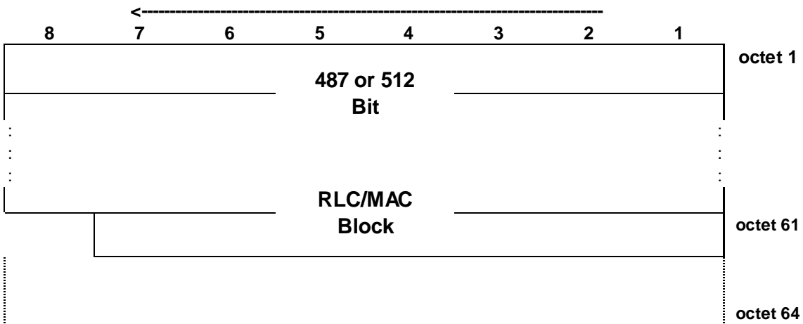
Figure 7.6.9.1: PDTCH block type 9 (MCS-5) uplink format
