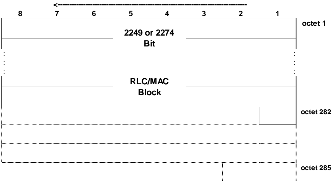
Figure 7.6.41.1: PDTCH block type 41 (DBS-11) format
