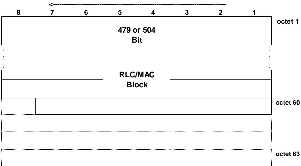
Figure 7.6.19.1: PDTCH block type 19 (UBS-5) format
