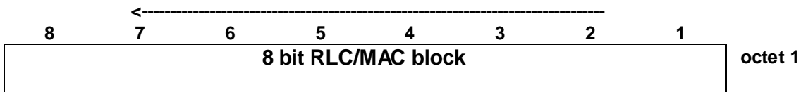
Figure 7.7.a: PRACH uplink/PACCH uplink short acknowledgement block format
