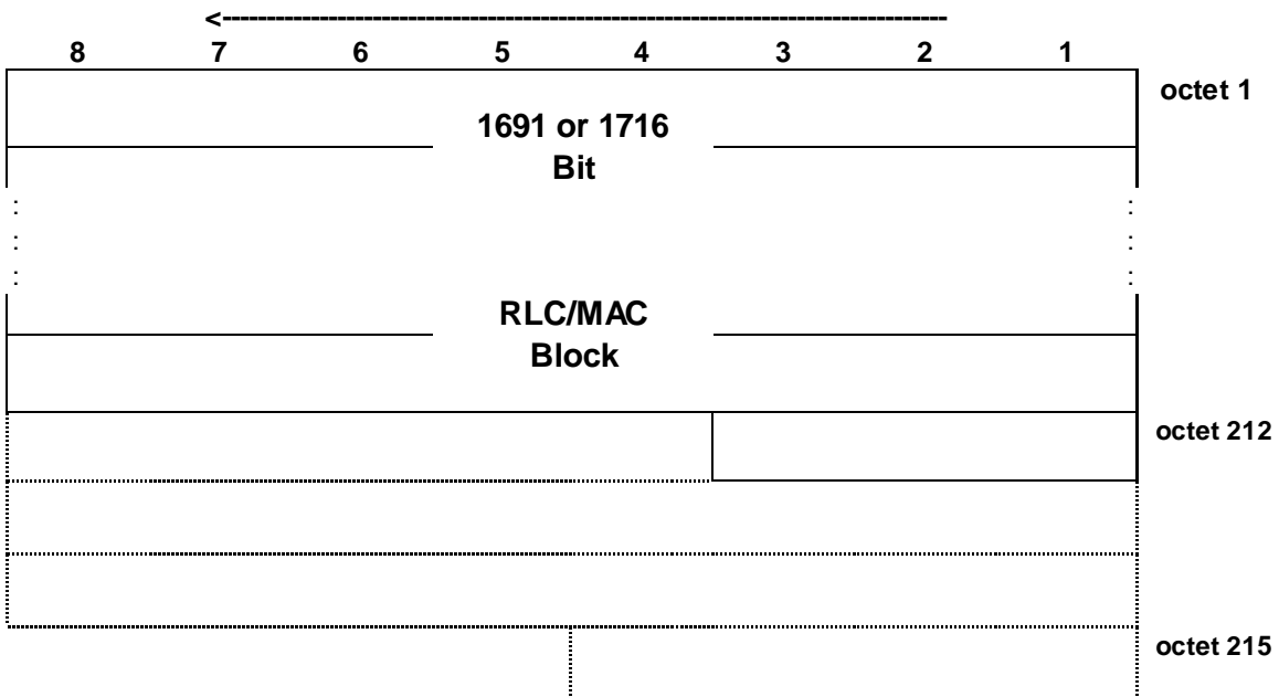
Figure 7.6.33.1: PDTCH block type 33 (DAS-11) format
