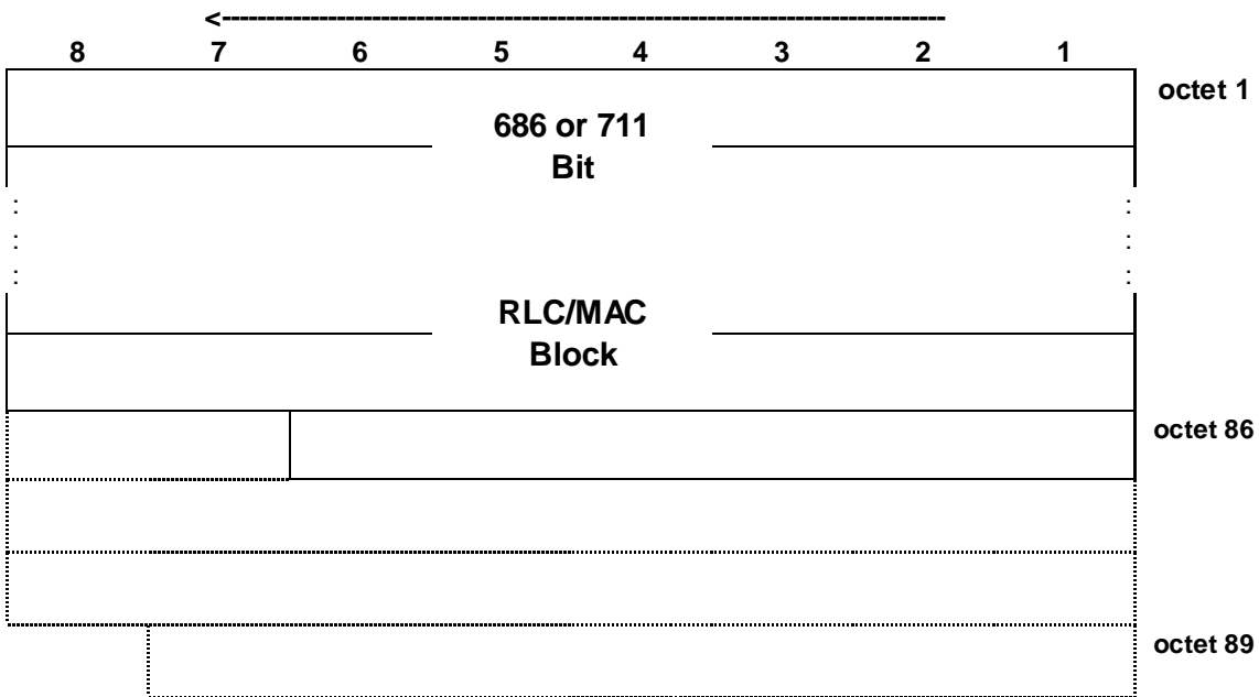
Figure 7.6.29.1: PDTCH block type 29 (DAS-7) format
