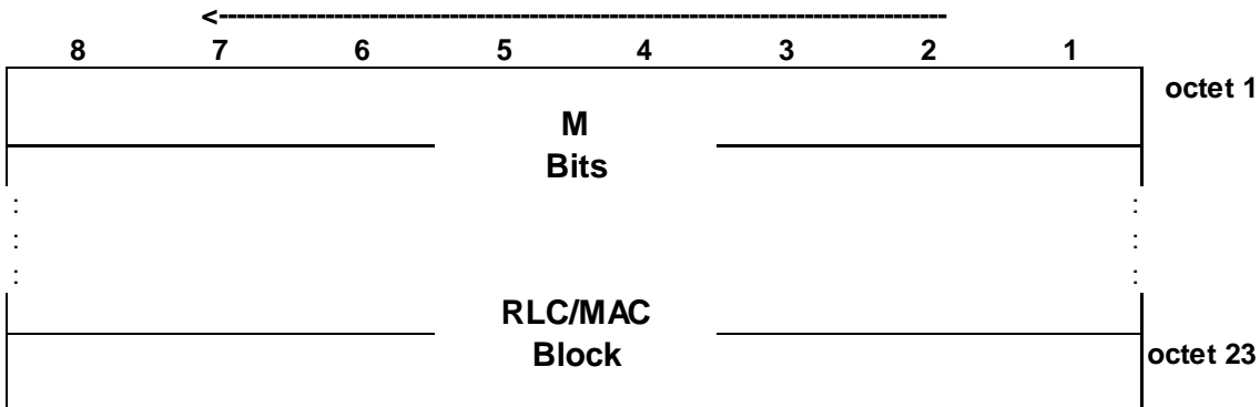
Figure 7.9a.2 Transport block format for TFC for signalling
