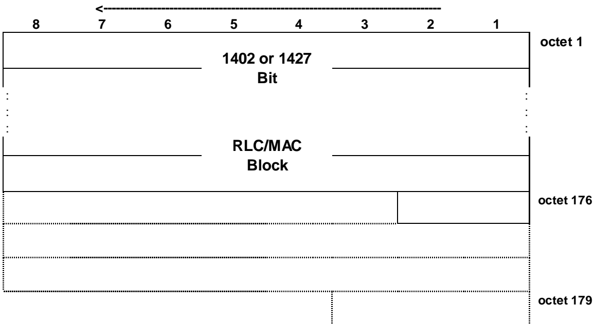
Figure 7.6.23.1: PDTCH block type 23 (UBS-9) format
