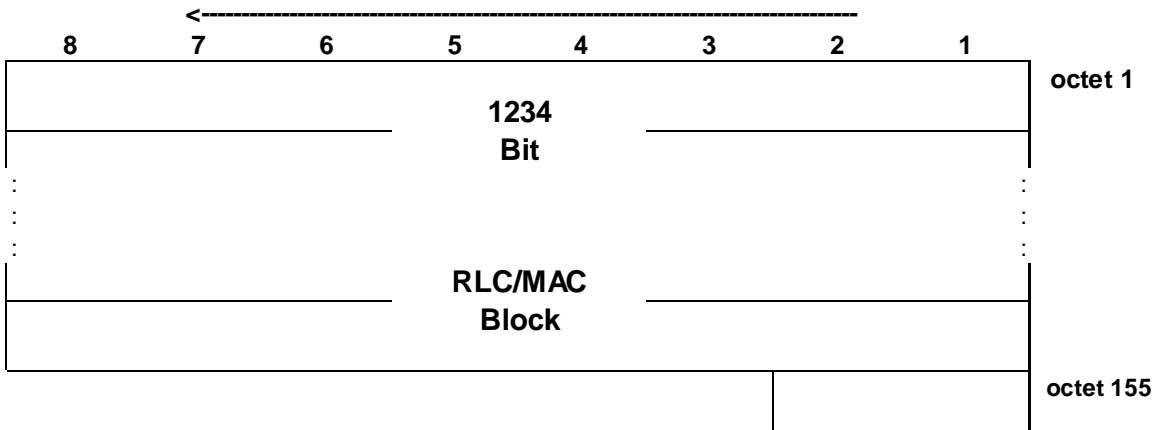
Figure 7.6.13.1: PDTCH block type 13 (MCS-9) uplink format
