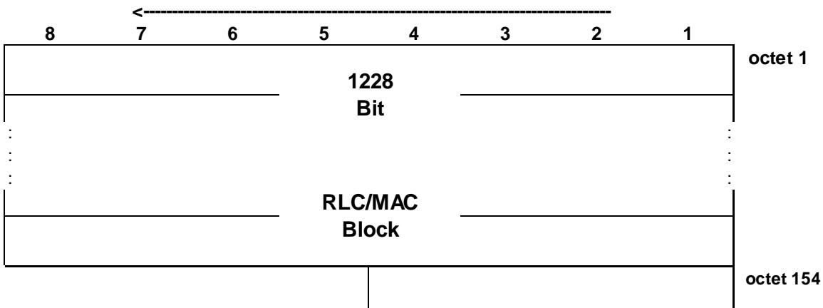
Figure 7.6.13.2: PDTCH block type 13 (MCS-9) downlink format
