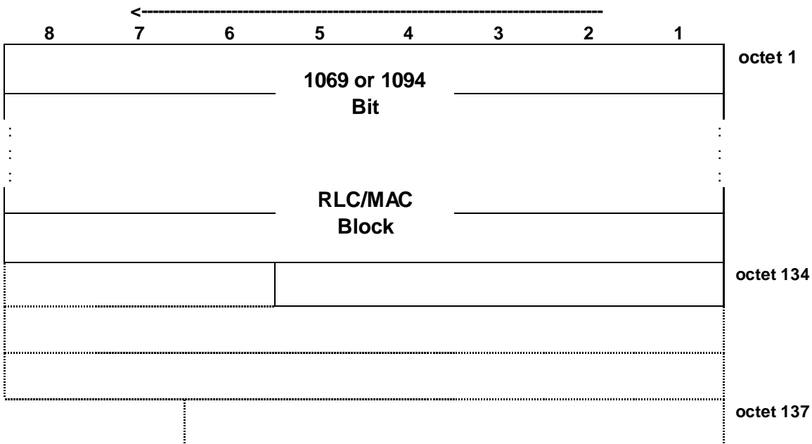
Figure 7.6.15.1: PDTCH block type 15 (UAS-8) format
