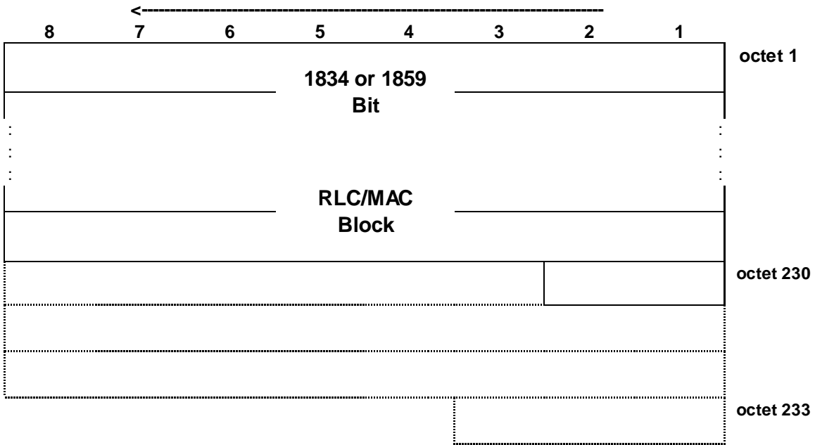
Figure 7.6.24.1: PDTCH block type 24 (UBS-10) format
