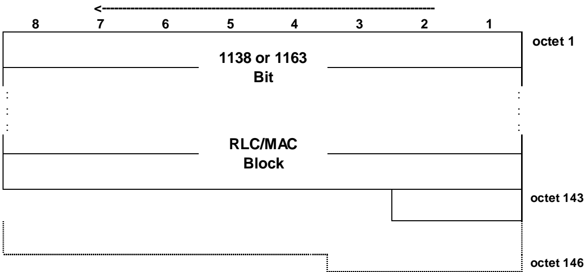
Figure 7.6.12.1: PDTCH block type 12 (MCS-8) uplink format
