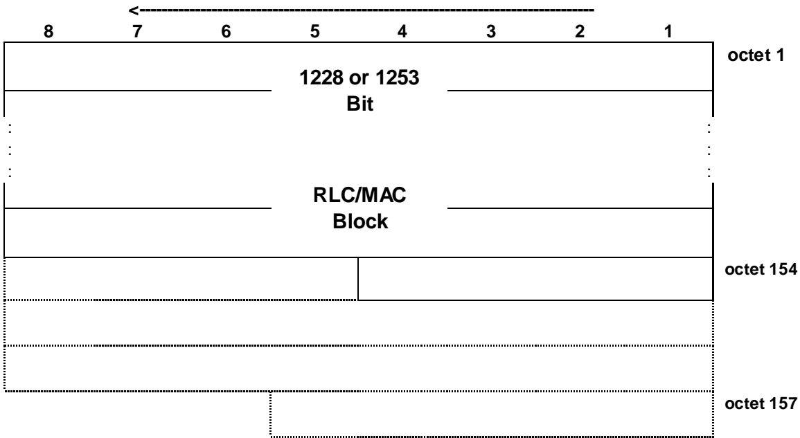
Figure 7.6.22.1: PDTCH block type 22 (UBS-8) format
