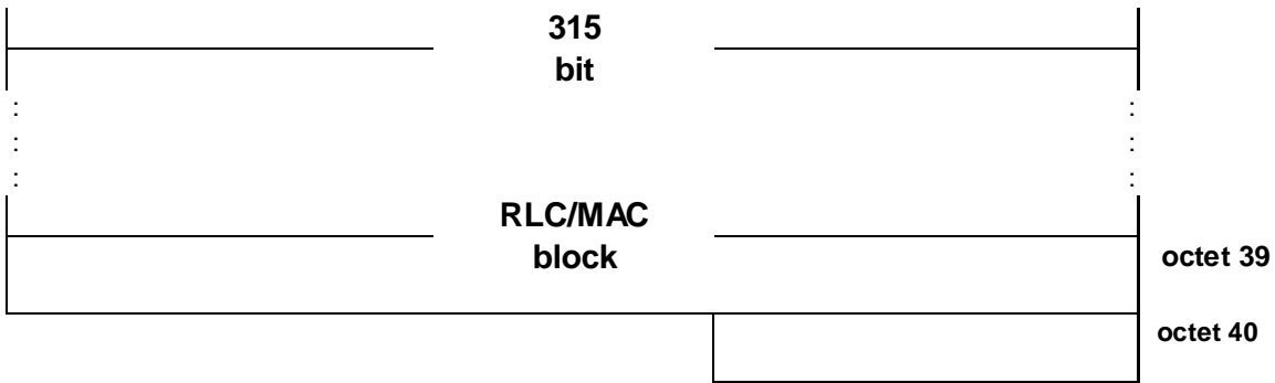
Figure 7.6.3: PDTCH block type 3 (CS-3) format
