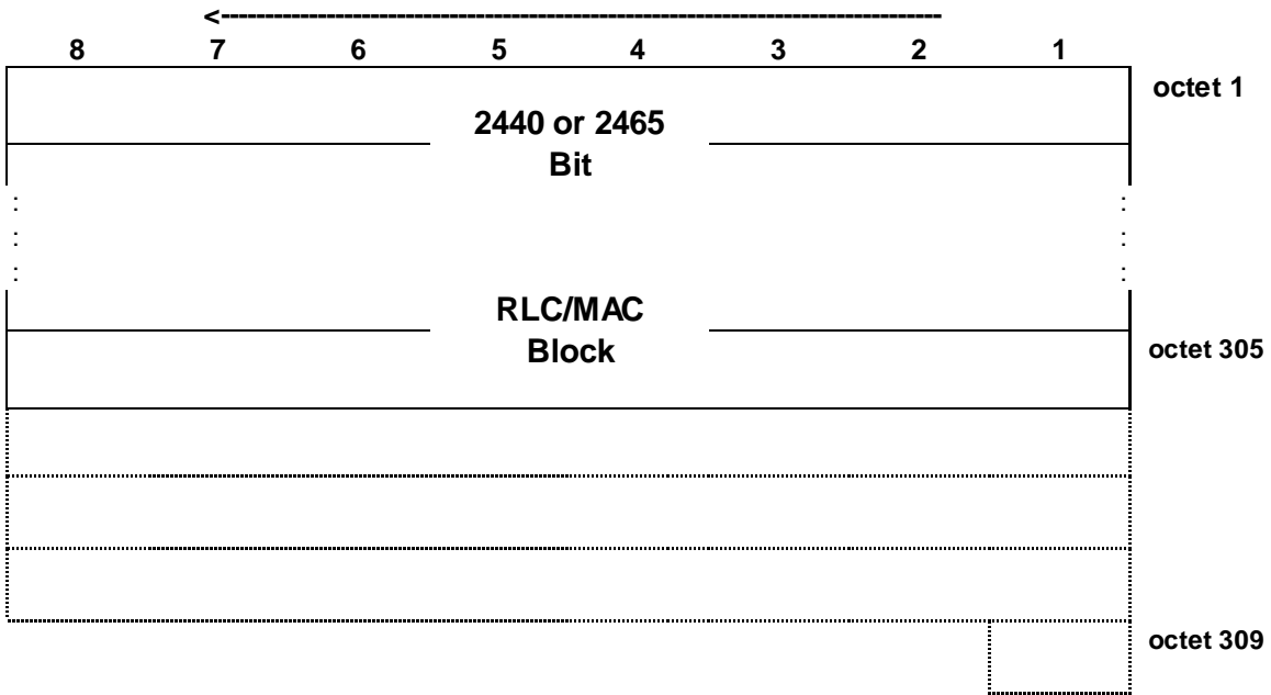
Figure 7.6.26.1: PDTCH block type 26 (UBS-12) format
