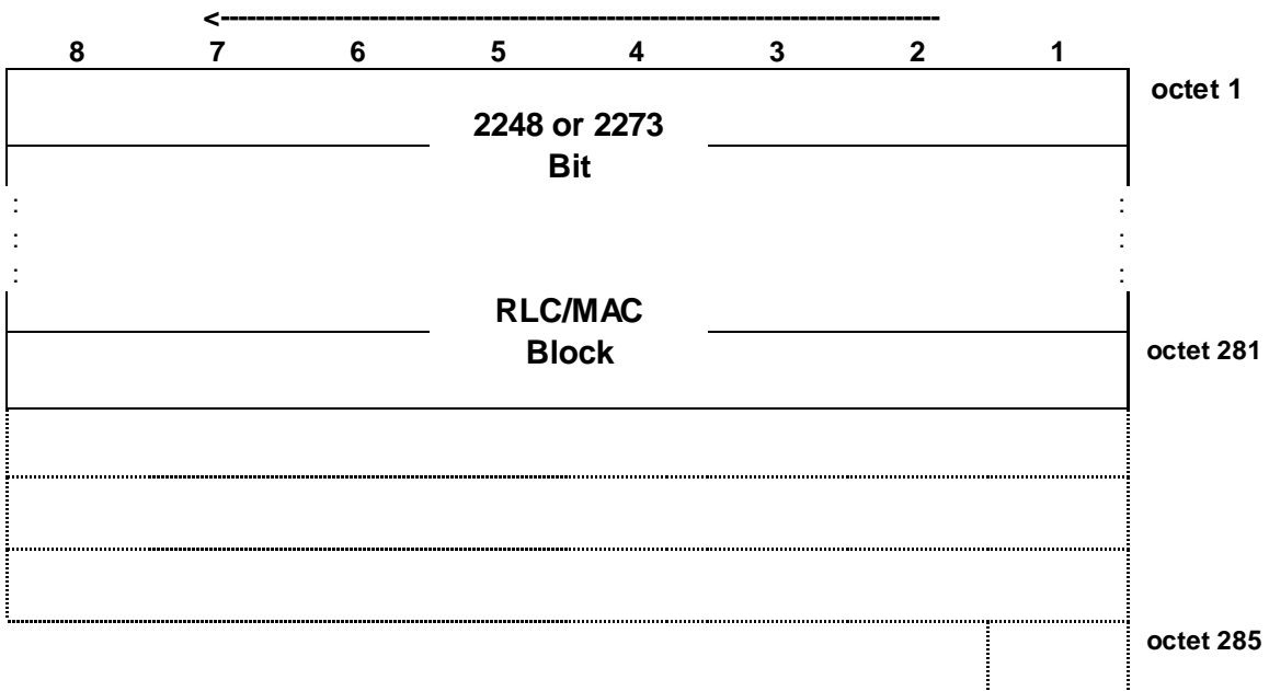
Figure 7.6.25.1: PDTCH block type 25 (UBS-11) format
