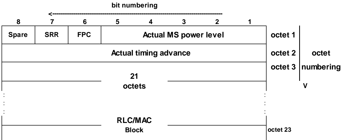
Figure 7.2.2: SACCH uplink block format for MS operating in lu mode
