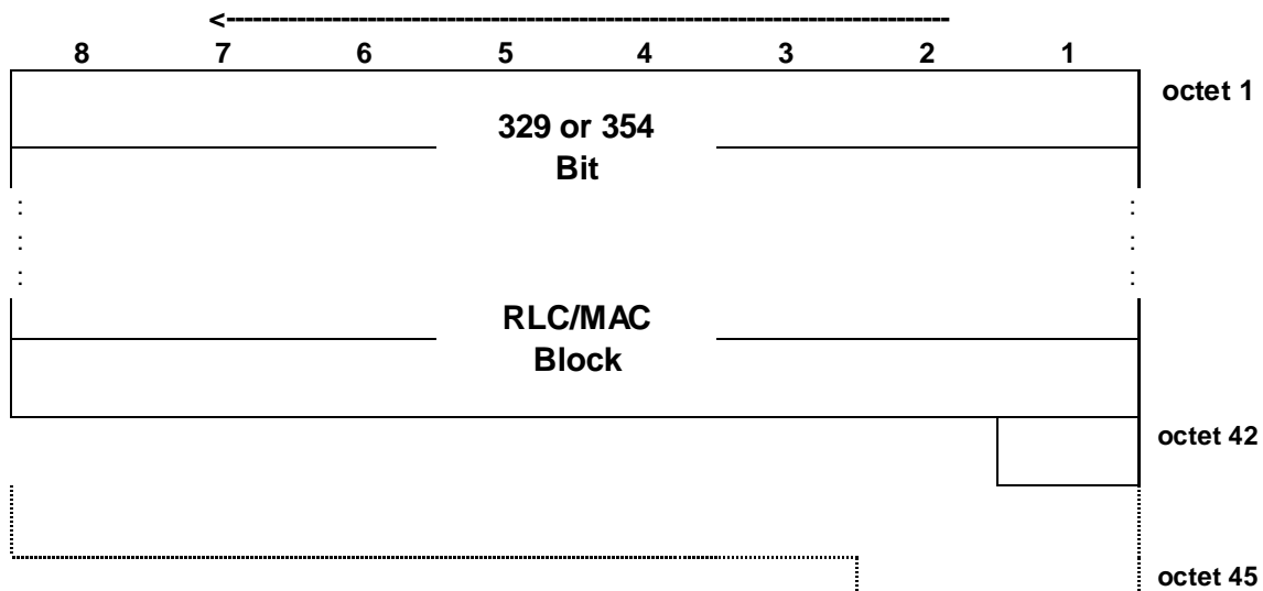
Figure 7.6.7: PDTCH block type 7 (MCS-3) format
