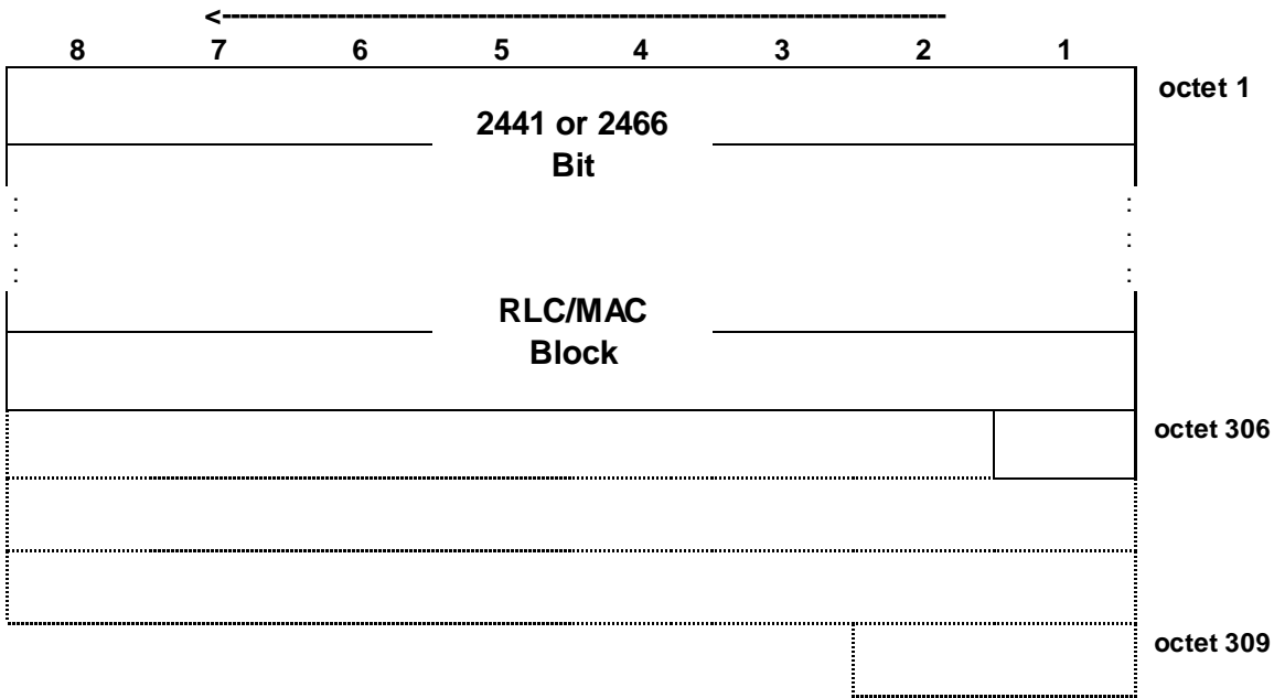
Figure 7.6.42.1: PDTCH block type 42 (DBS-12) format
