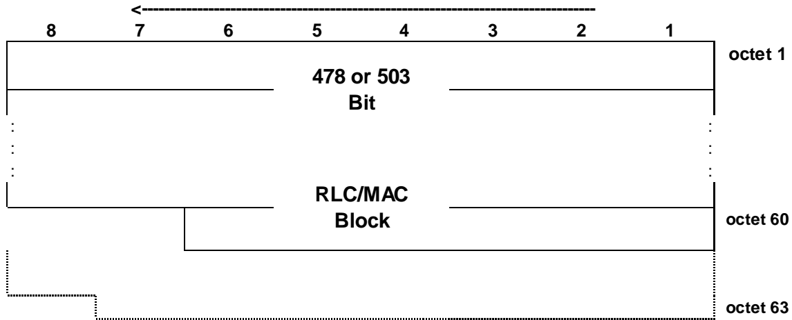
Figure 7.6.9.2: PDTCH block type 9 (MCS-5) downlink format
