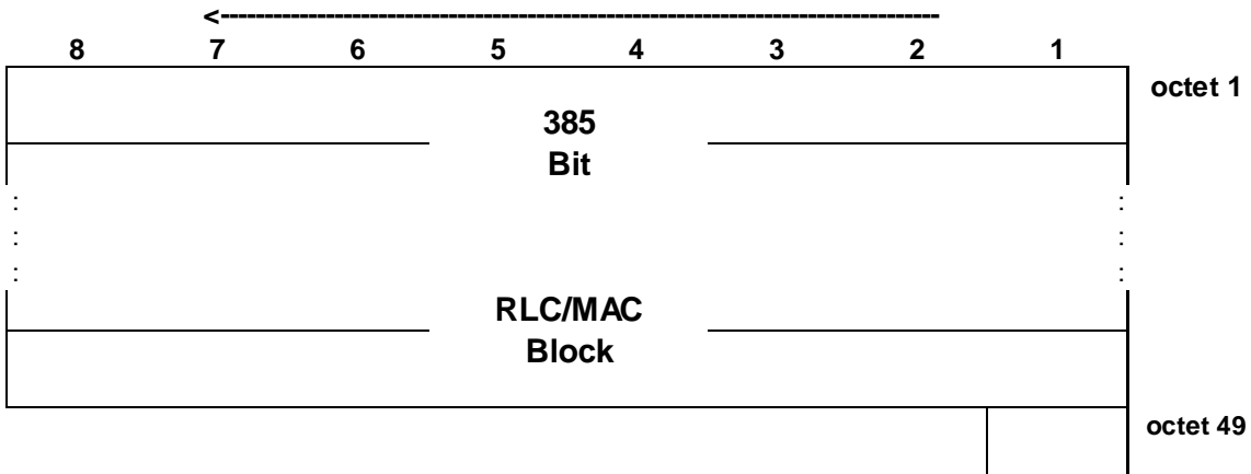
Figure 7.6.8: PDTCH block type 8 (MCS-4) format
