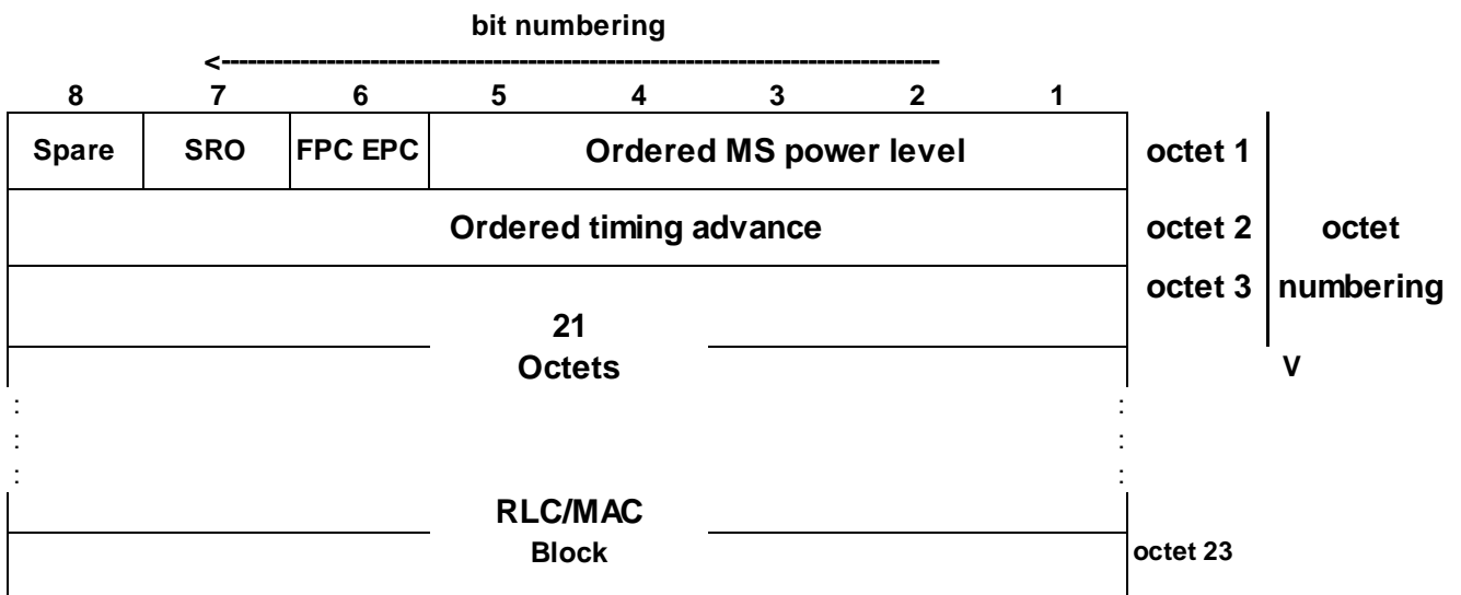
Figure 7.1.2: SACCH downlink block format for MS operating in lu mode
