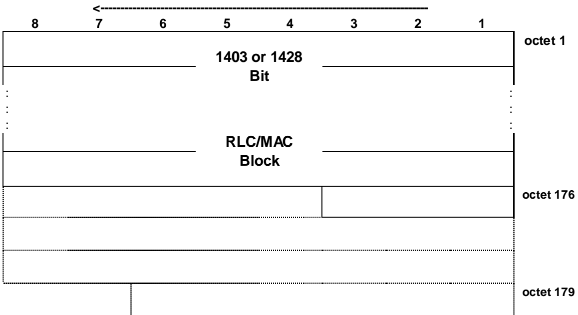
Figure 7.6.39.1: PDTCH block type 39 (DBS-9) format
