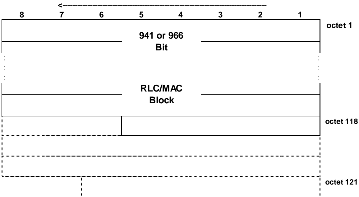
Figure 7.6.37.1: PDTCH block type 37 (DBS-7) format
