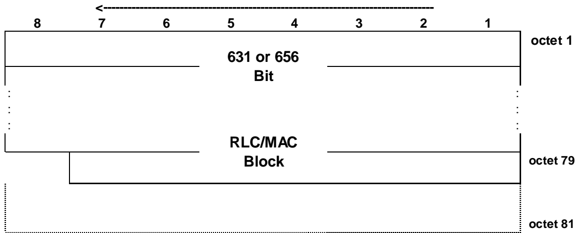
Figure 7.6.10.1: PDTCH block type 10 (MCS-6) uplink format
