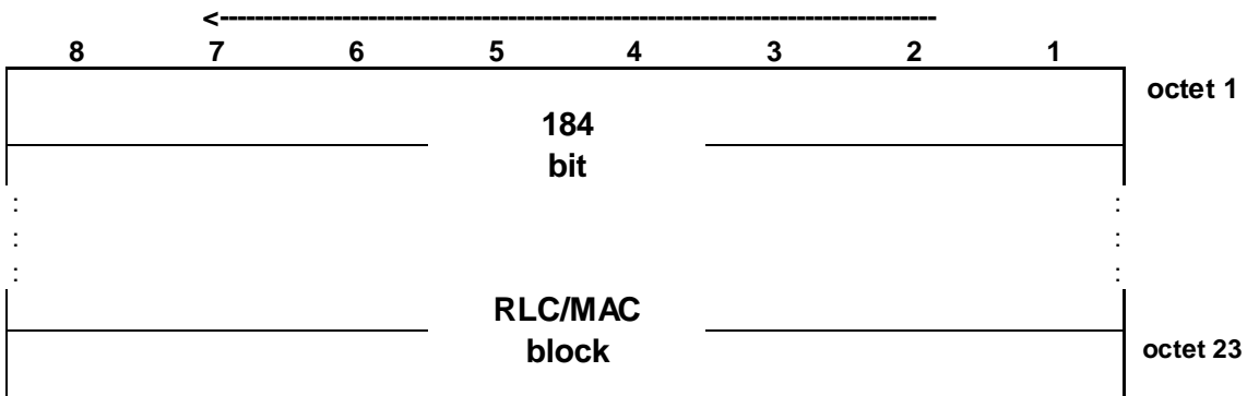
Figure 7.6.1: PDTCH block type 1 (CS-1) format
