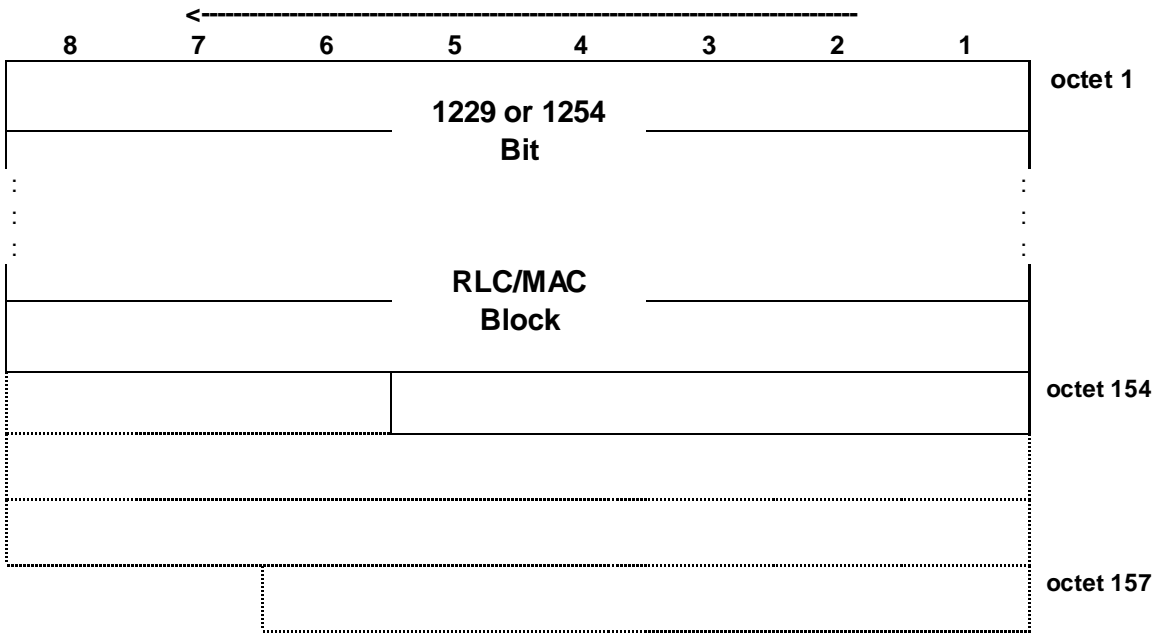
Figure 7.6.16.1: PDTCH block type 16 (UAS-9) format
