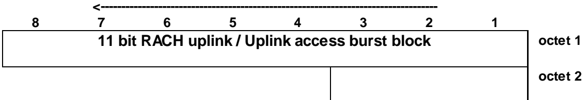
Figure 7.4a.b: 11 bit RACH uplink / Uplink access burst block format
