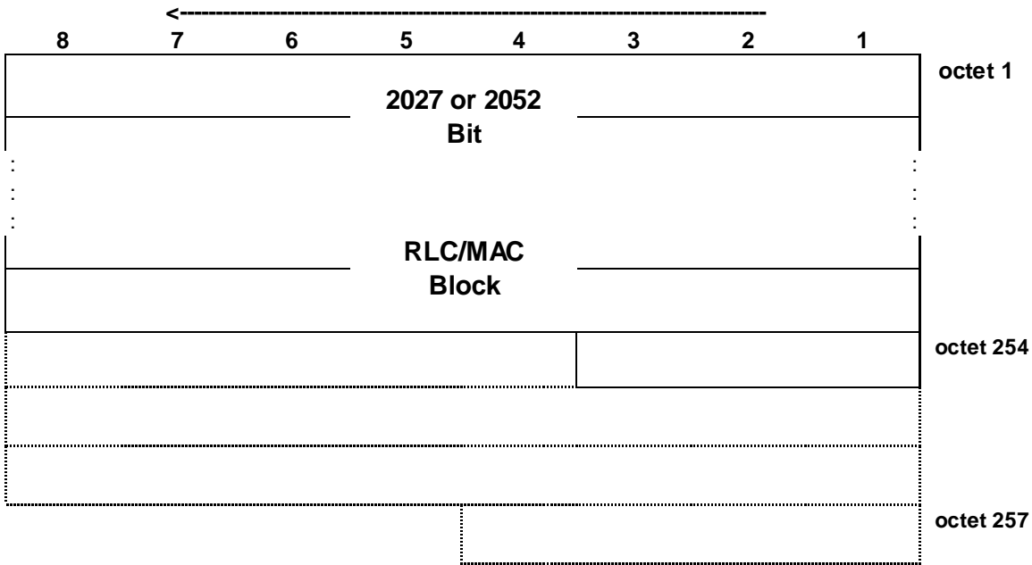
Figure 7.6.34.1: PDTCH block type 34 (DAS-12) format
