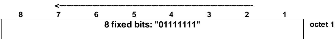
Figure 7.9.a: PTCCH uplink block format
