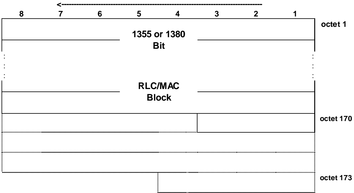
Figure 7.6.32.1: PDTCH block type 32 (DAS-10) format
