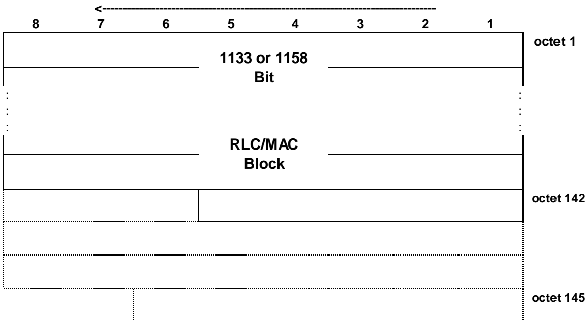
Figure 7.6.31.1: PDTCH block type 31 (DAS-9) format
