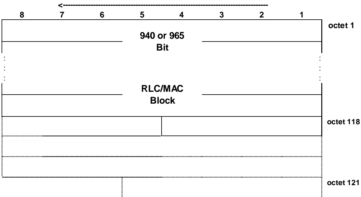
Figure 7.6.21.1: PDTCH block type 21 (UBS-7) format
