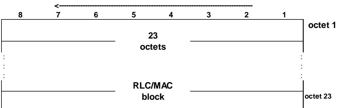
Figure 7.4.2: FACCH/SDCCH uplink block format for MS operating in lu mode
