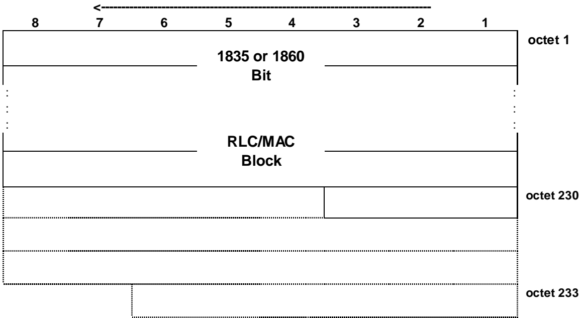
Figure 7.6.40.1: PDTCH block type 40 (DBS-10) format
