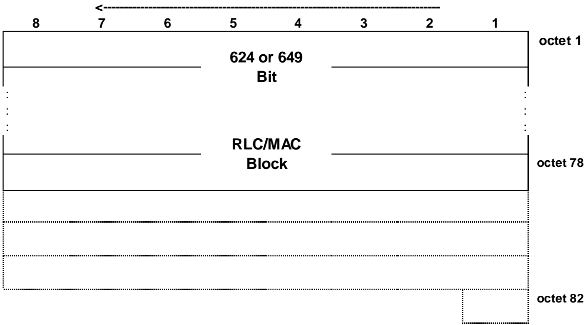
Figure 7.6.36.1: PDTCH block type 36 (DBS-6) format
