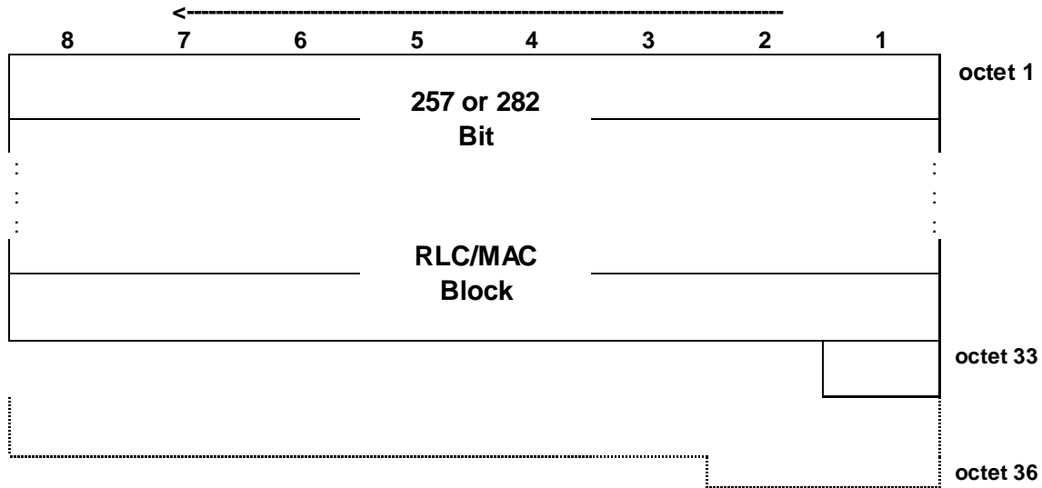
Figure 7.6.6: PDTCH block type 6 (MCS-2) format
