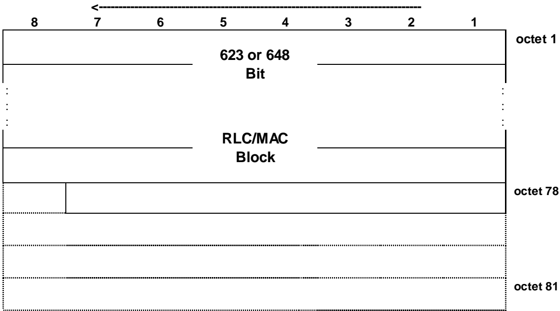
Figure 7.6.20.1: PDTCH block type 20 (UBS-6) format
