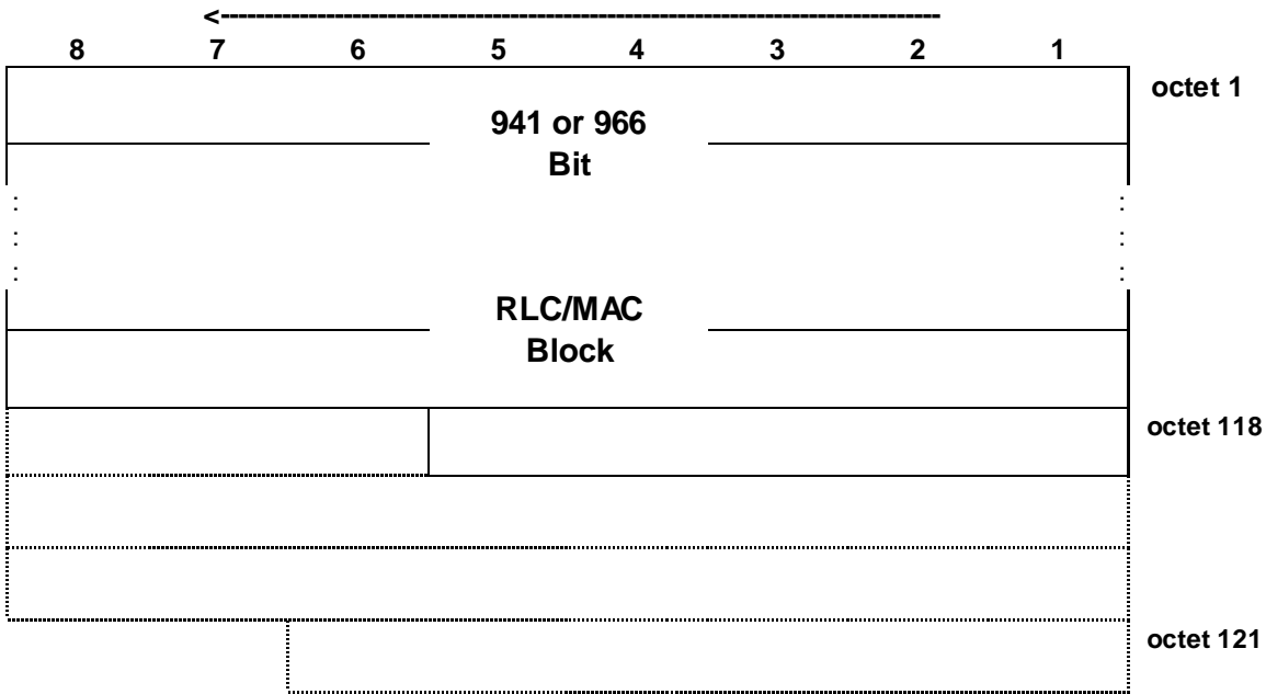
Figure 7.6.30.1: PDTCH block type 30 (DAS-8) format
