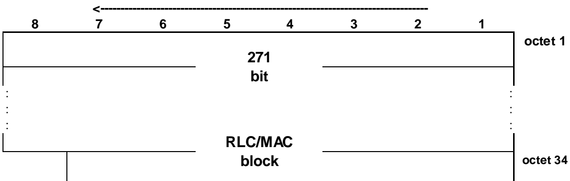
Figure 7.6.2: PDTCH block type 2 (CS-2) format
