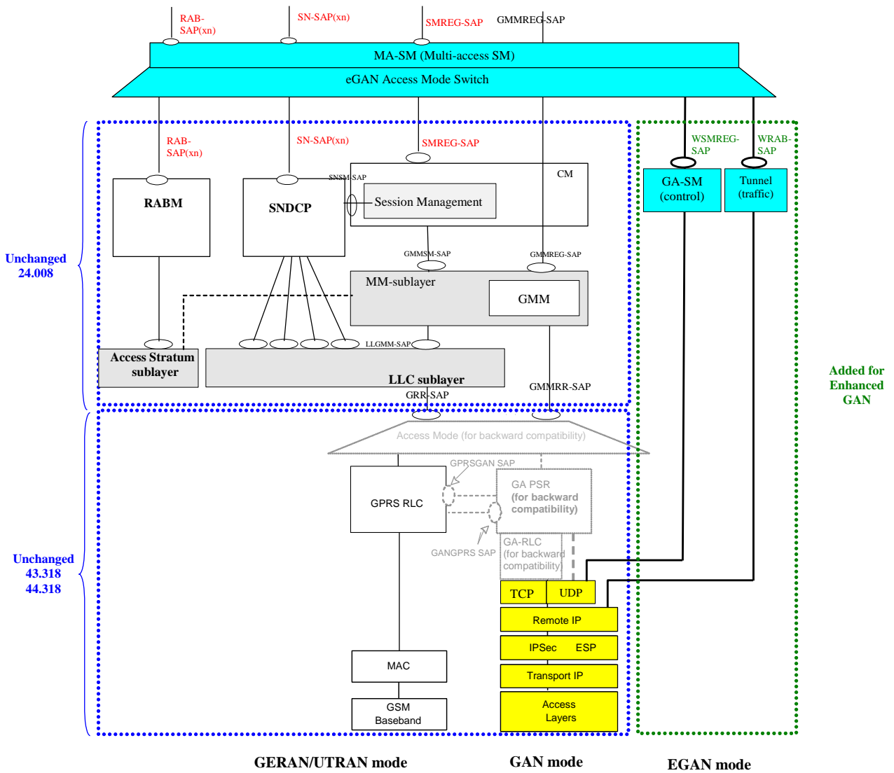
Figure 34: UMTS-GSM-GPRS-GAN terminal
