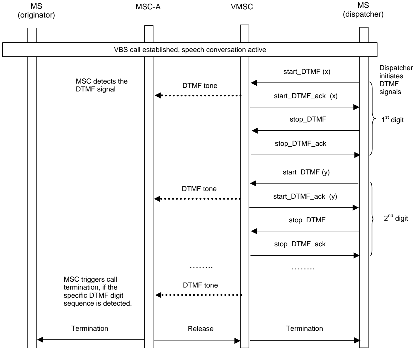
Figure 4c: Signalling required for broadcast call termination by an entitled mobile dispatcher, if the mobile dispatcher is controlled by a visited MSC (could be a relay MSC) of the broadcast call.
