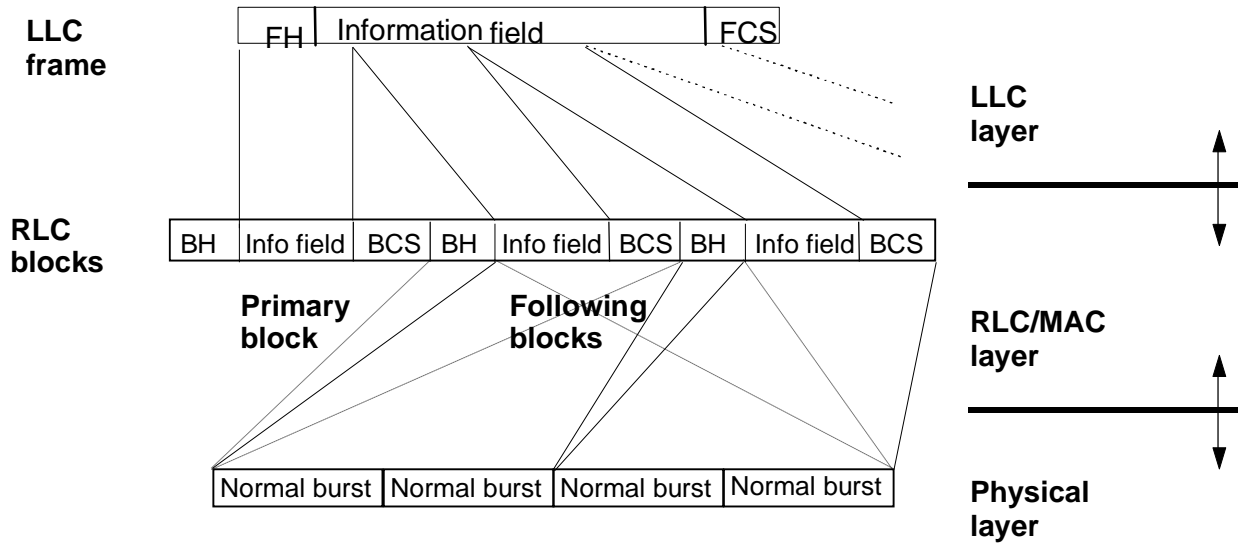
Figure 22: Transmission and reception data flow for EGPRS MCS-9 and MCS-8
