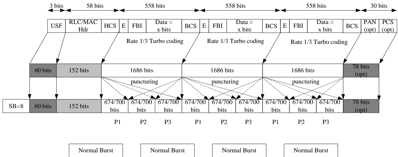
Figure 18e.2: Coding and puncturing for DAS-11; rate 0.84/0.80 32QAM, three RLC blocks per radio block
