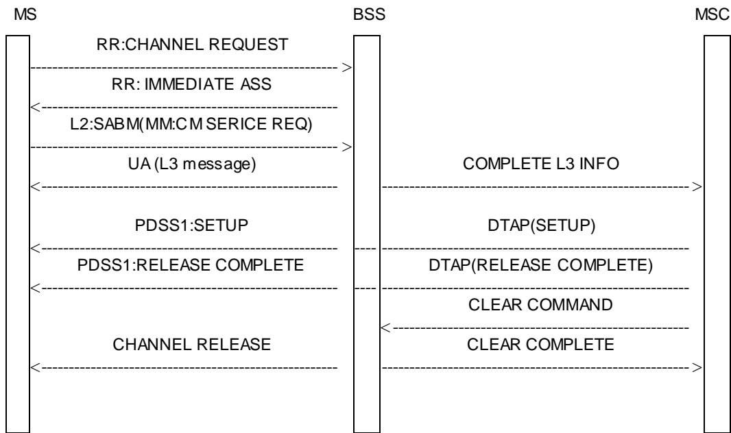
Figure 5: Signalling flow for PDSS1 (rejection of service after setup)
