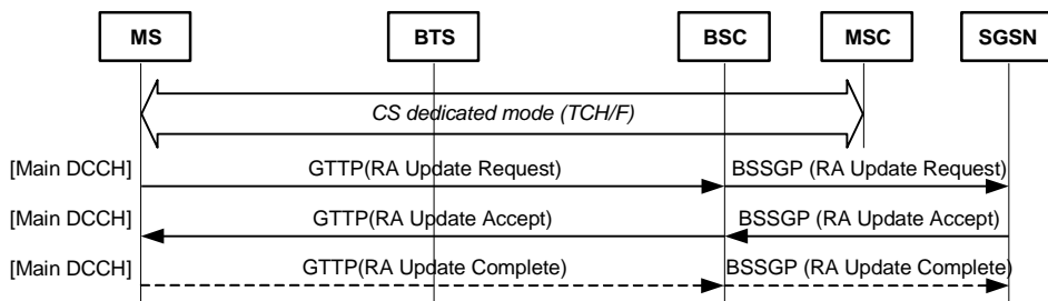
Figure 14: Routeing Area Update procedure in dedicated mode, packet idle mode and Ready state; performed on the main DCCH
