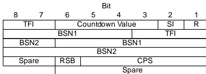
Figure B.6: Uplink RLC Data Block Header for MCS-7, MCS-8 and MCS-9
