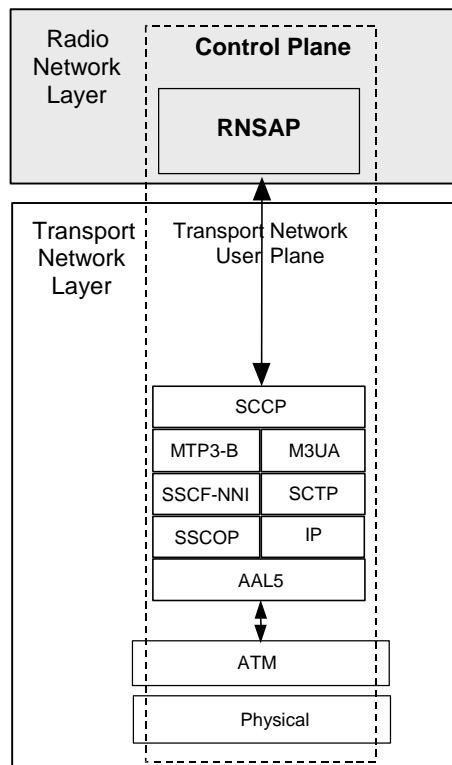
Figure 9: Iur-g Protocol Architecture
