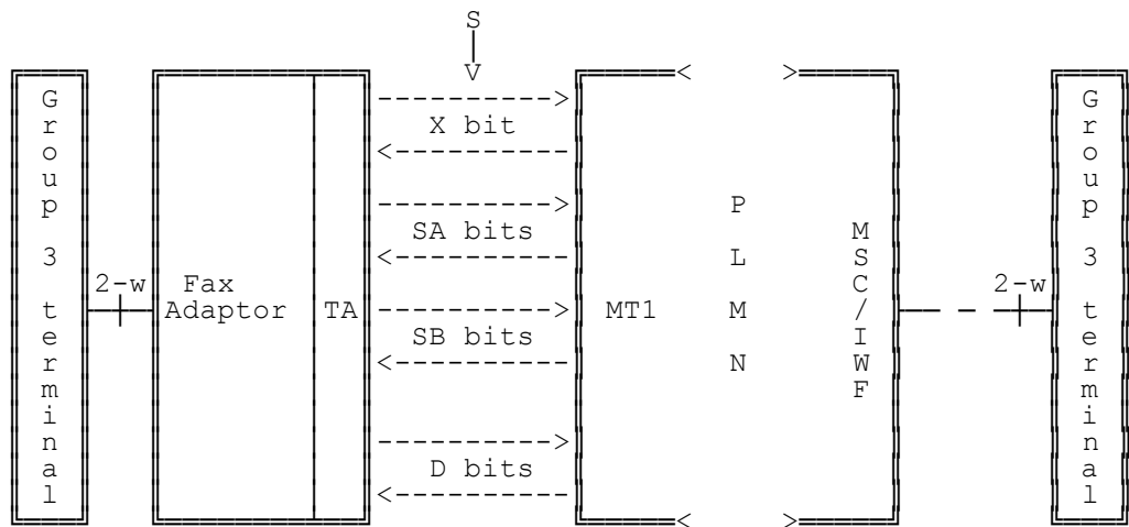
Figure 4b/43.046: Optional Teleservice connection
