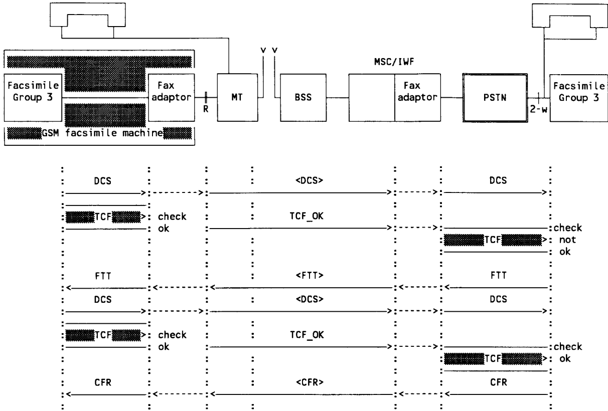
Figure B.11/43.046: Mobile originated facsimile transmission - error recovery (example)
