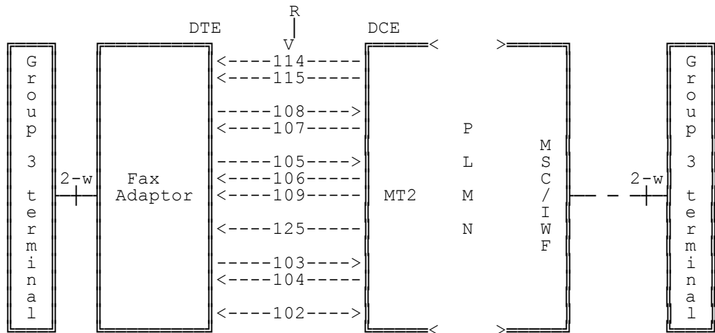
Figure 4a/43.046: Standard Teleservice connection
