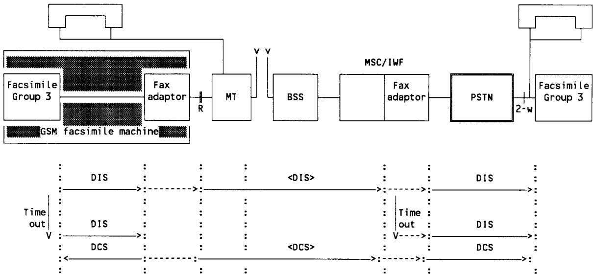
Figure B.10/43.046: Mobile terminated facsimile transmission - error recovery (example)
