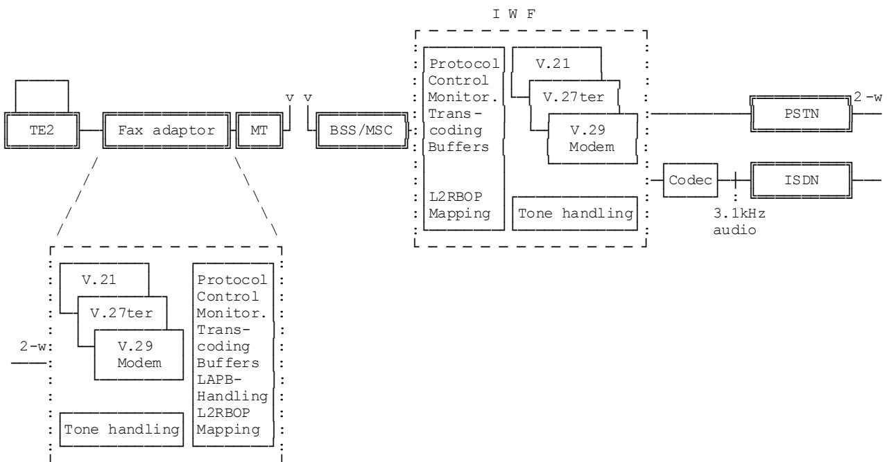
Figure 7/43.046: Network interworking
