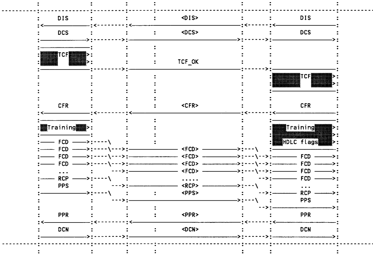
Figure B.8/43.046: Mobile originated facsimile transmission (error correction mode)
