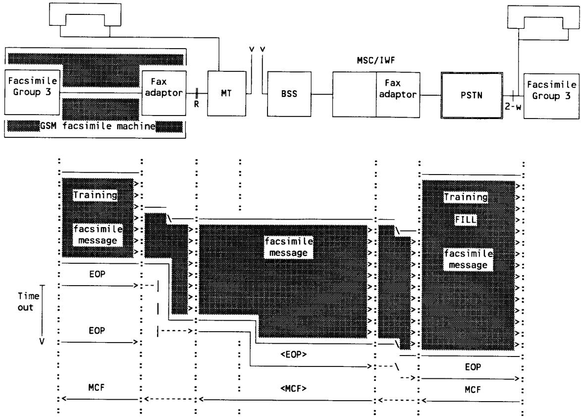
Figure B.13/43.046: Mobile originated facsimile transmission - error recovery (example)
