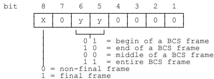
Figure A.2/43.046: Element discriminator of a BCS element
