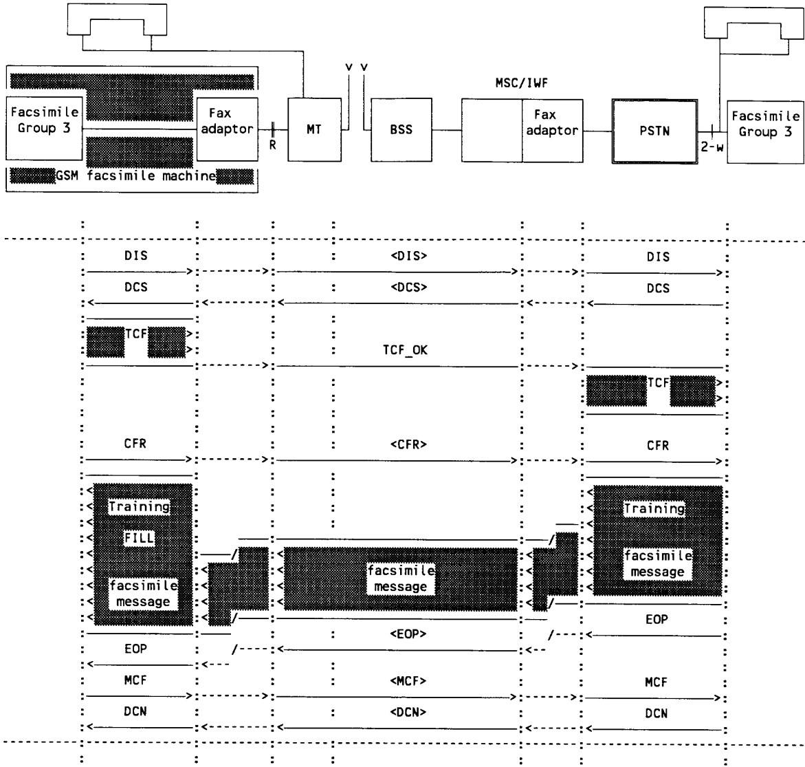
Figure B.7/43.046: Mobile terminated facsimile transmission
