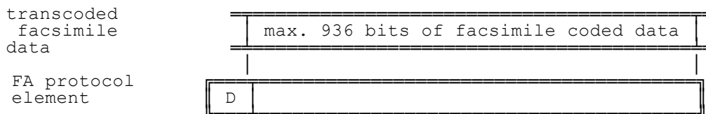
Figure A.11/43.046: Information field content of a normal fax data element
