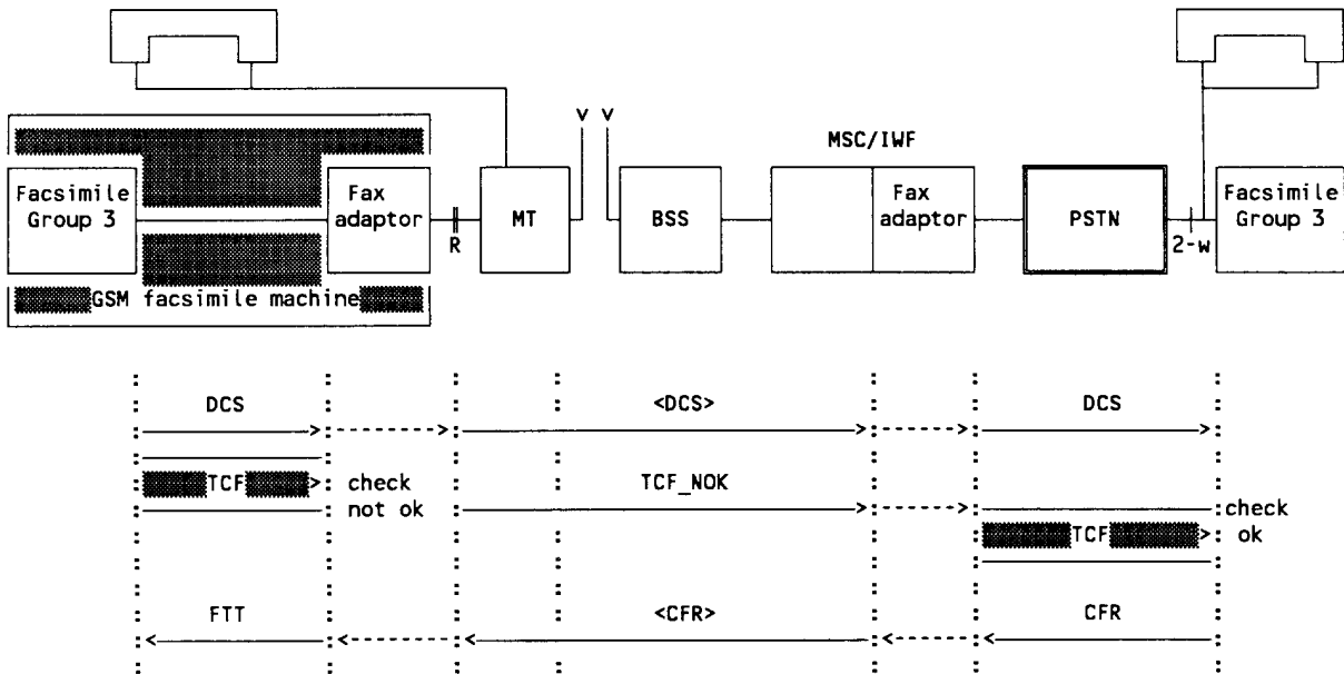
Figure B.12/43.046: Mobile originated facsimile transmission - error recovery (example)
