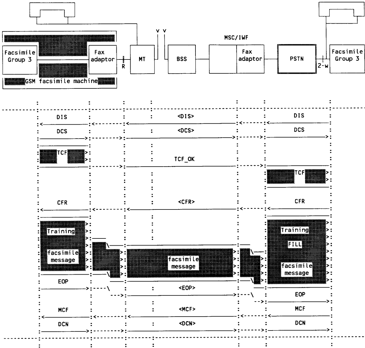
Figure B.6/43.046: Mobile originated facsimile transmission
