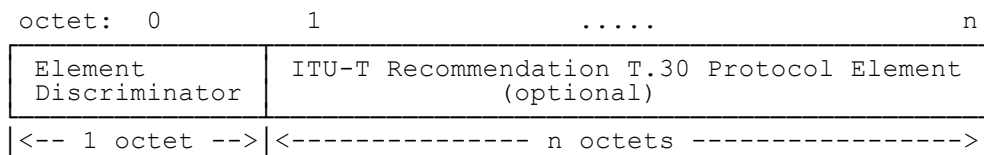
Figure A.1/43.046: Principle FA protocol element structure
