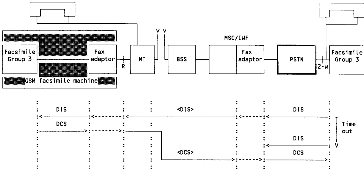
Figure B.9/43.046: Mobile originated facsimile transmission - error recovery (example)
