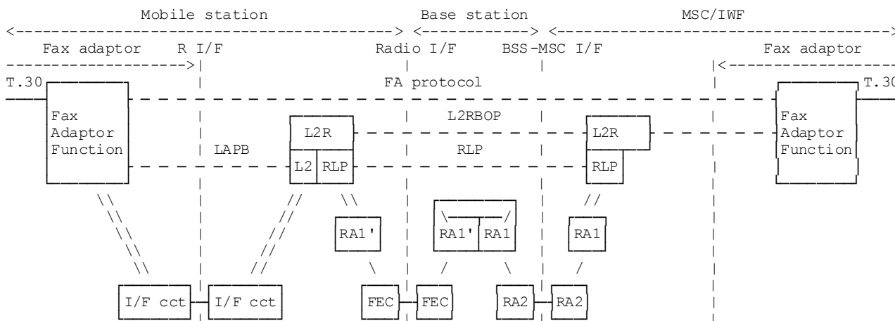
Figure 5/43.046: Protocol model for non-transparent support
