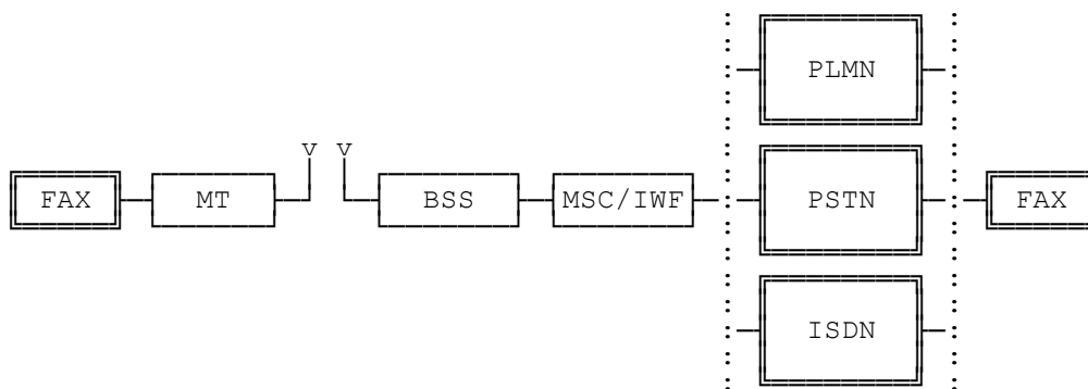
Figure 1/43.046: Network architecture
