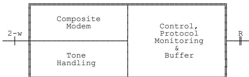
Figure 3/43.046: Fax adaptor scheme
