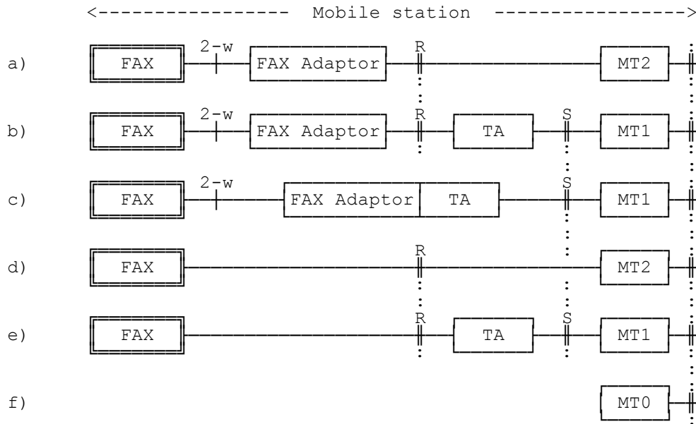
Figure 2/43.046: Reference configurations
