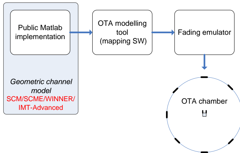
Figure 6.3.1.2.1-1: Modelling process
