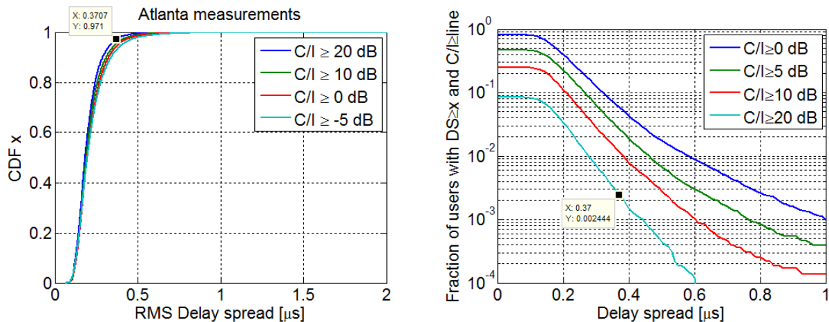
Figure 5.5.4.4-4: Measured results from Atlanta, GA
