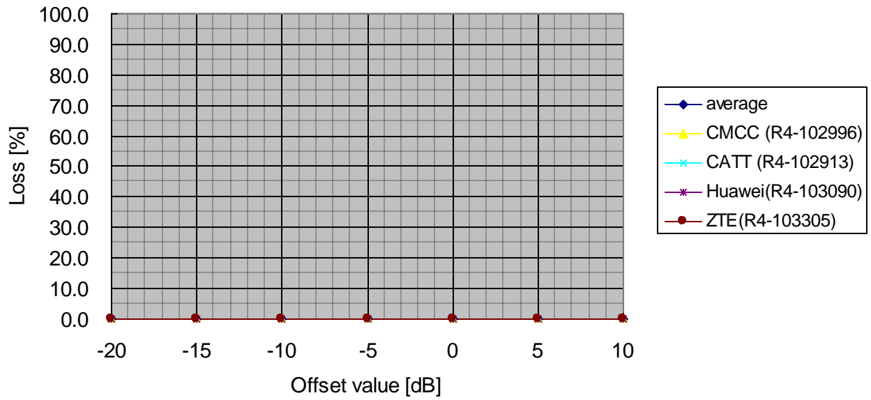
Figure 12.27 average 1.6 MHz UTRA uplink capacity loss (TPC set 1)
