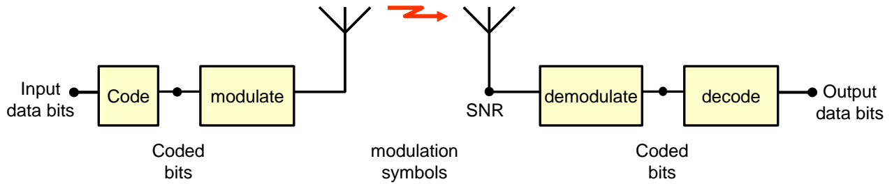
Figure A.3 Coding and Modulation for Transmission of data over a radio link
