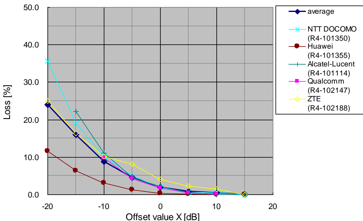
Figure 12.23 average 5 MHz UTRA downlink capacity loss
