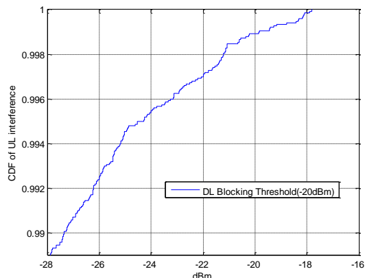
Figure 6.2.3.2-2 CDF of UL interference (Zoom in view)
