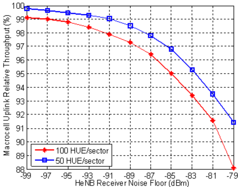
Figure 6.2.1.1.2-1 Relative uplink throughput loss versus noise floor
