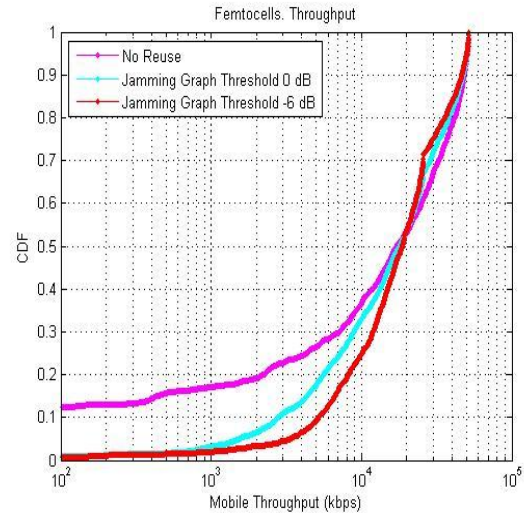
(b) Mobile throughput
