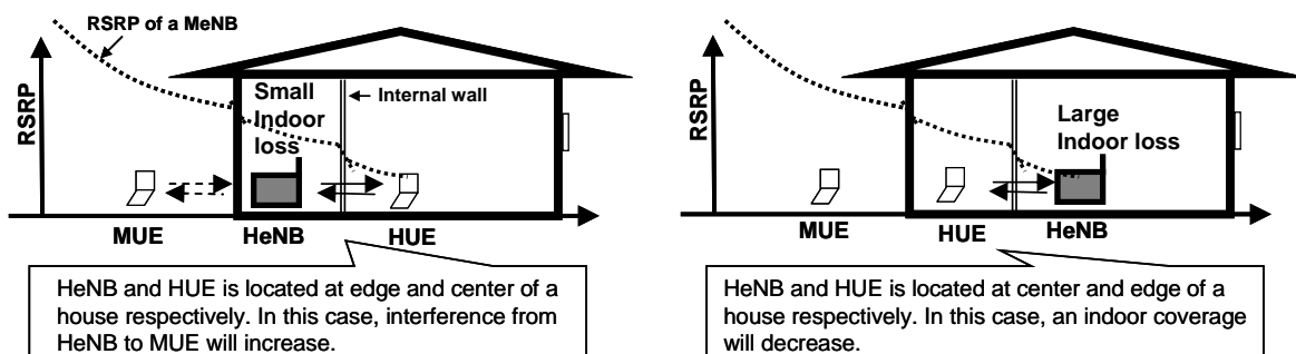
Figure 7.2.3.1-1 Scenarios where HeNB transmit power are not appropriately set.
