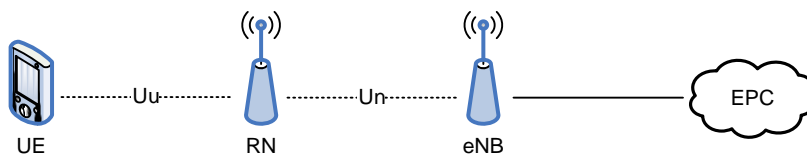
Figure 9.1-1: Relays
