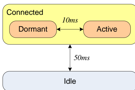
Figure 10.1-1: C-Plane Latency
