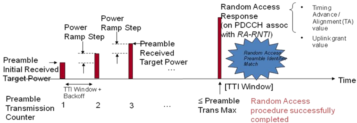
Figure 4.7.4.1.1-1: RACH Procedure
