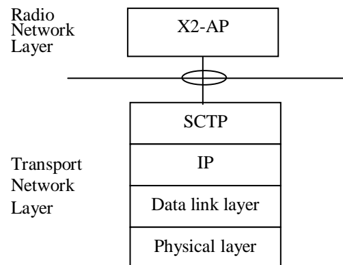
Figure 4.1: X2 signalling bearer protocol stack
