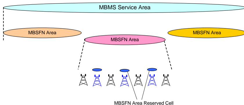
Figure 15-1: MBMS Definitions
