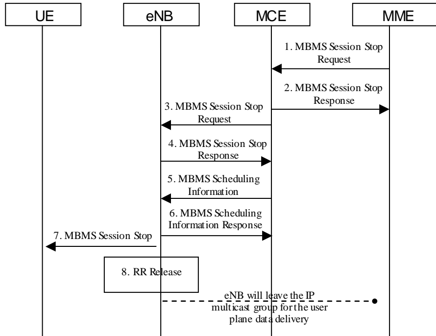
Figure 15.7.1.2-1. Session Stop procedure
