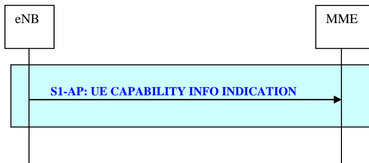
Figure 19.2.2.20-1: UE Capability Info Indication procedure
