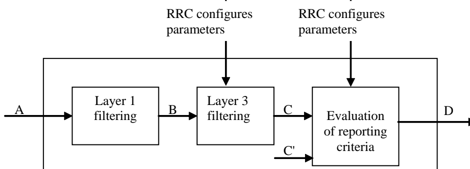
Figure 10.6-1: Measurement model
