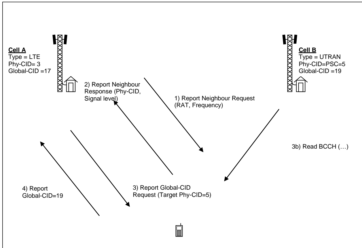
Figure 22.3.4-1: Automatic Neighbour Relation Function in case of UTRAN detected cell
