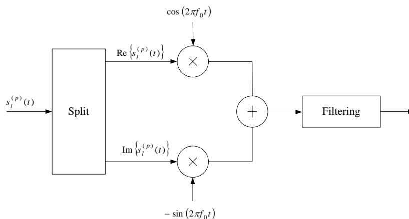
Figure 6.13-1: Downlink modulation
