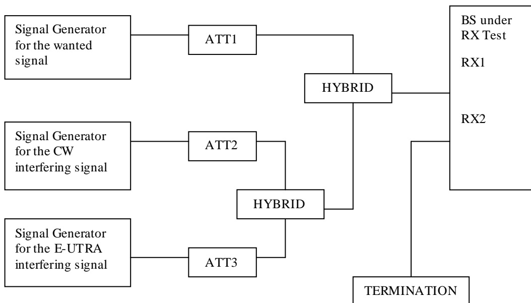
Figure 1.2-7: Measuring system Set-up for intermodulation characteristics
