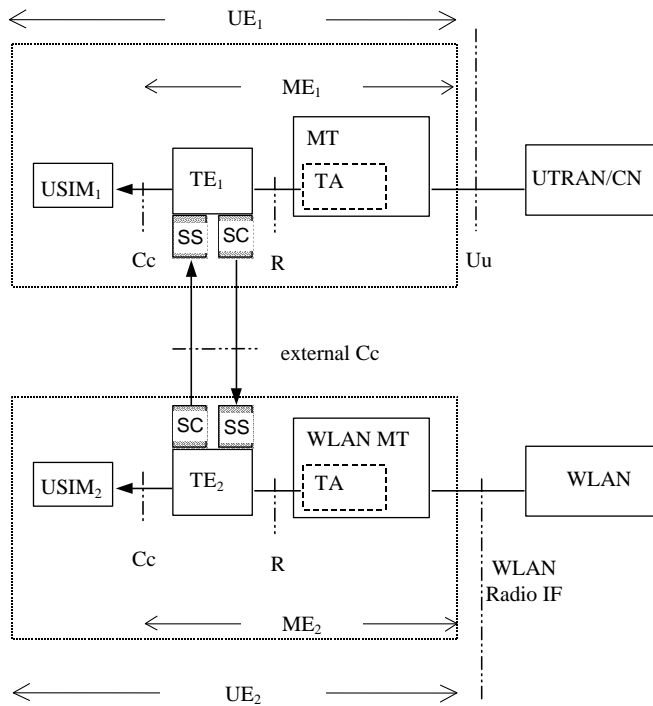
Figure 2: Security Architecture Reference Model
