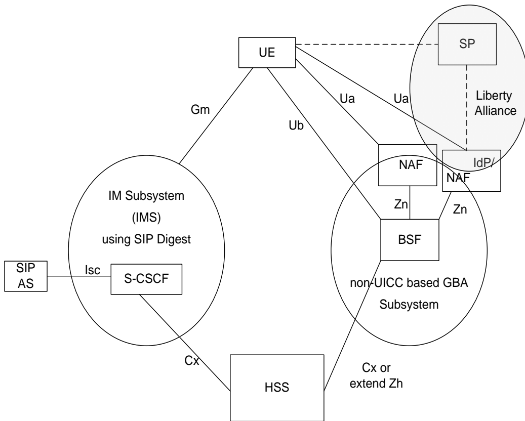
Figure 7.2-3 interworking with Liberty Alliance
