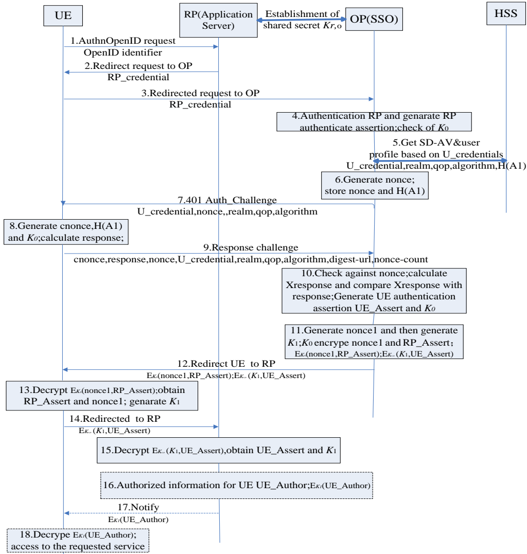
Figure 7.3-65 authentication process of interworking of the SIP Digest-based SSOSDALS with the OpenID that co-hosts IdP (SSO Server) and OP
