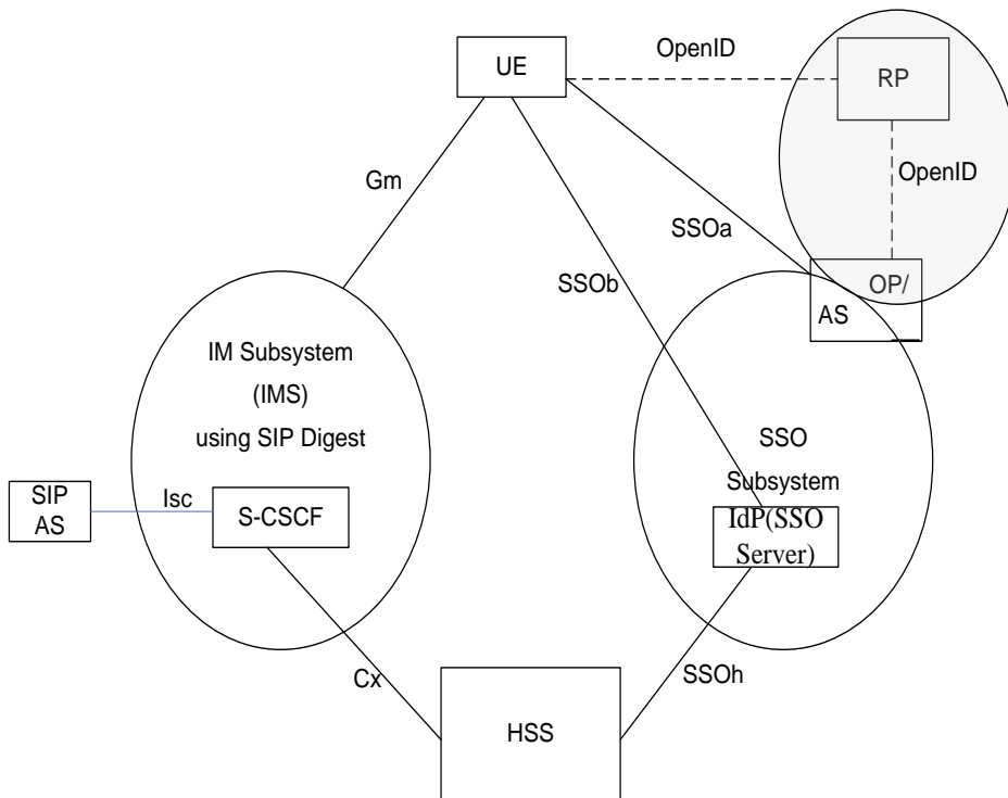
Figure 7.3-2: Architecture for interworking with OpenID that co-hosts AS and OP
