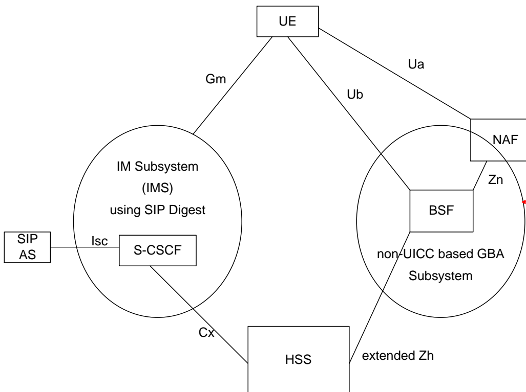
Figure 7.2-1 Architecture of GBA_Digest
