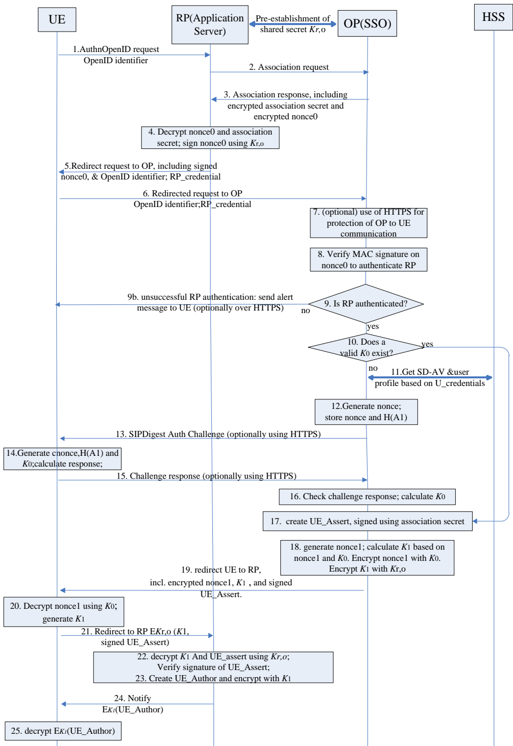
Figure 7.3-78 authentication in the interworking of the SIP Digest-based SSO-SDALS with the OpenID RP (SSO Server) and OP co-hosting, with RP authentication
