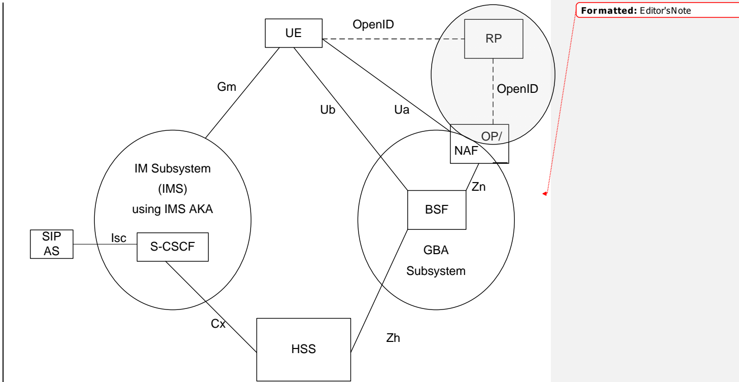
Figure 5.1-4: Relation of GBA with the Common IMS and interworking with OpenID
