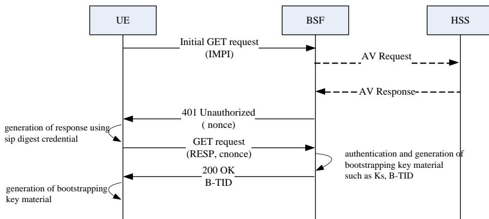
Figure 7.2-2 GBA_Digest bootstrapping procedure
