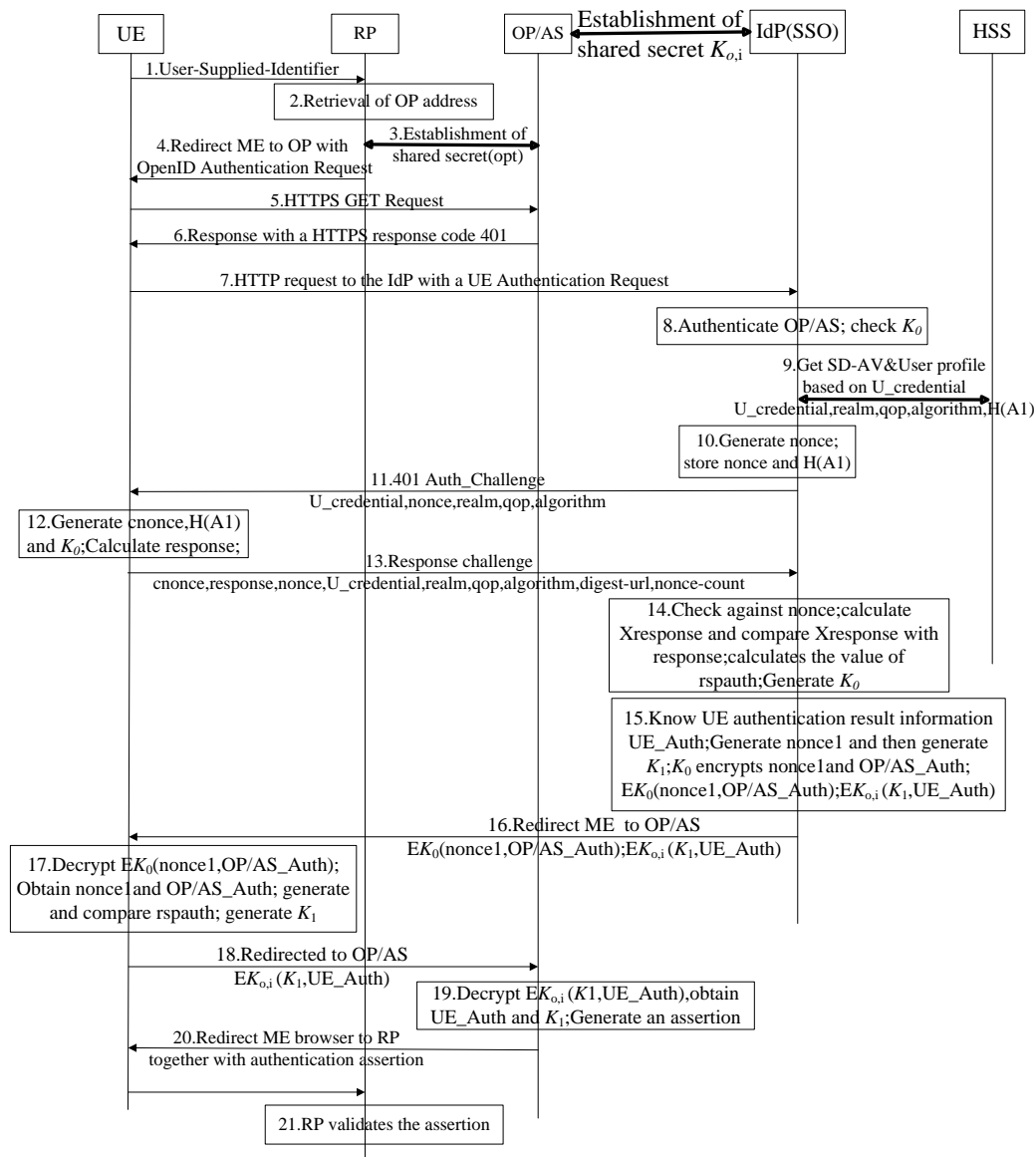
Figure 7.3-76 Interworking of SDALS message flow with OpenID that co-hosts AS and OP
