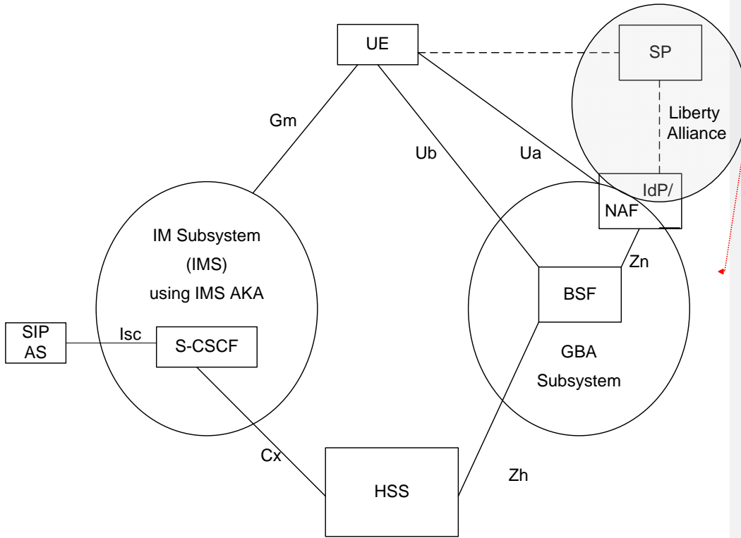
Figure 5.1-2: Relation of GBA with the Common IMS and interworking with Liberty Alliance collocating IdP and NAF
