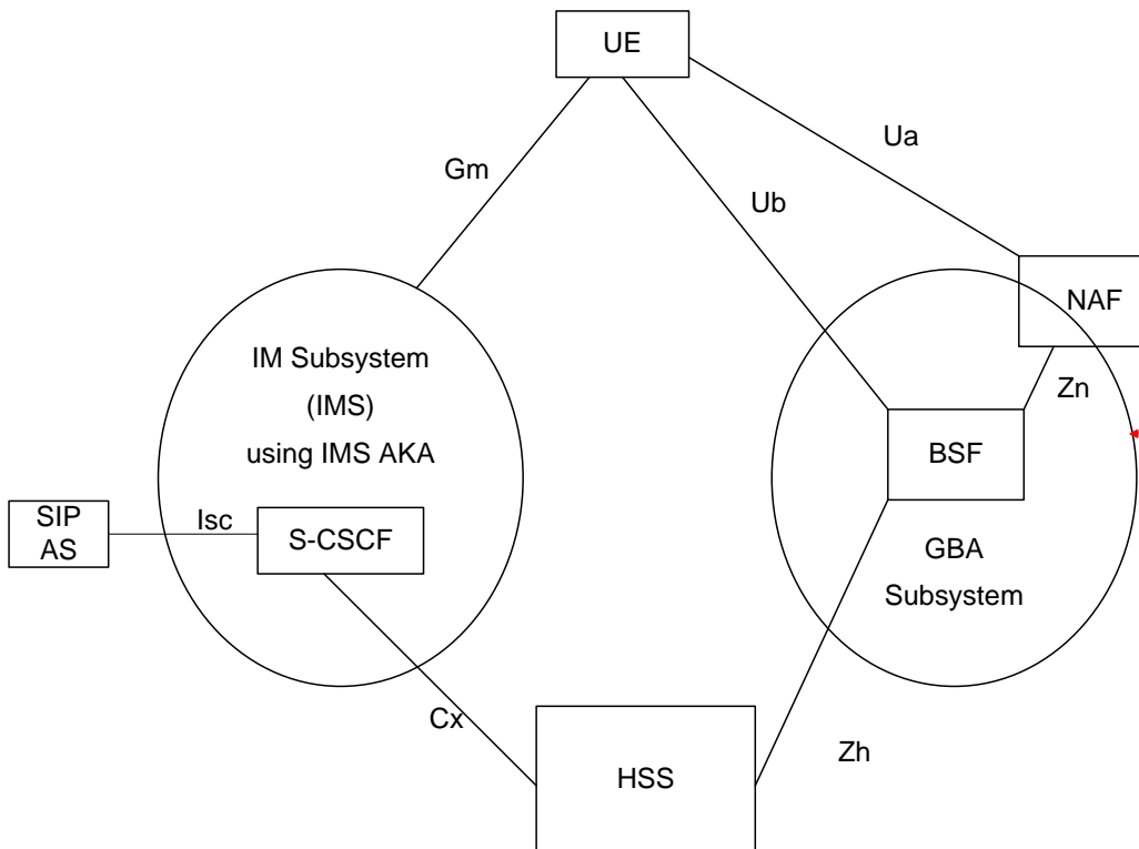
Figure 5.1-1: Relation of GBA with the Common IMS
