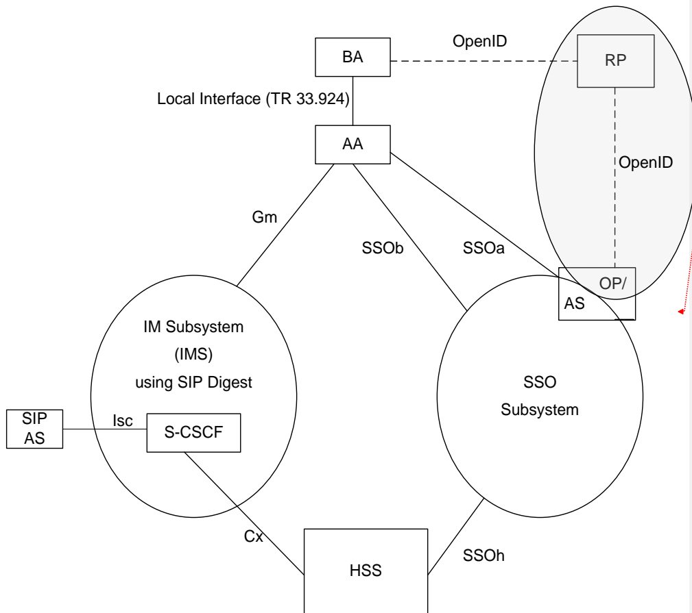
Figure 5.5-2: Relation of SIP Digest-based SSO with the Common IMS and interworking with OpenID for the split terminal scenarios
