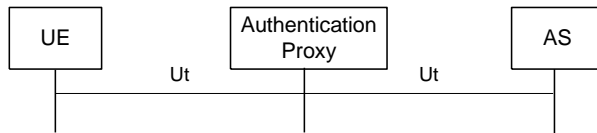
Figure 5.3-2: Authentication proxy in the Ut interface path
