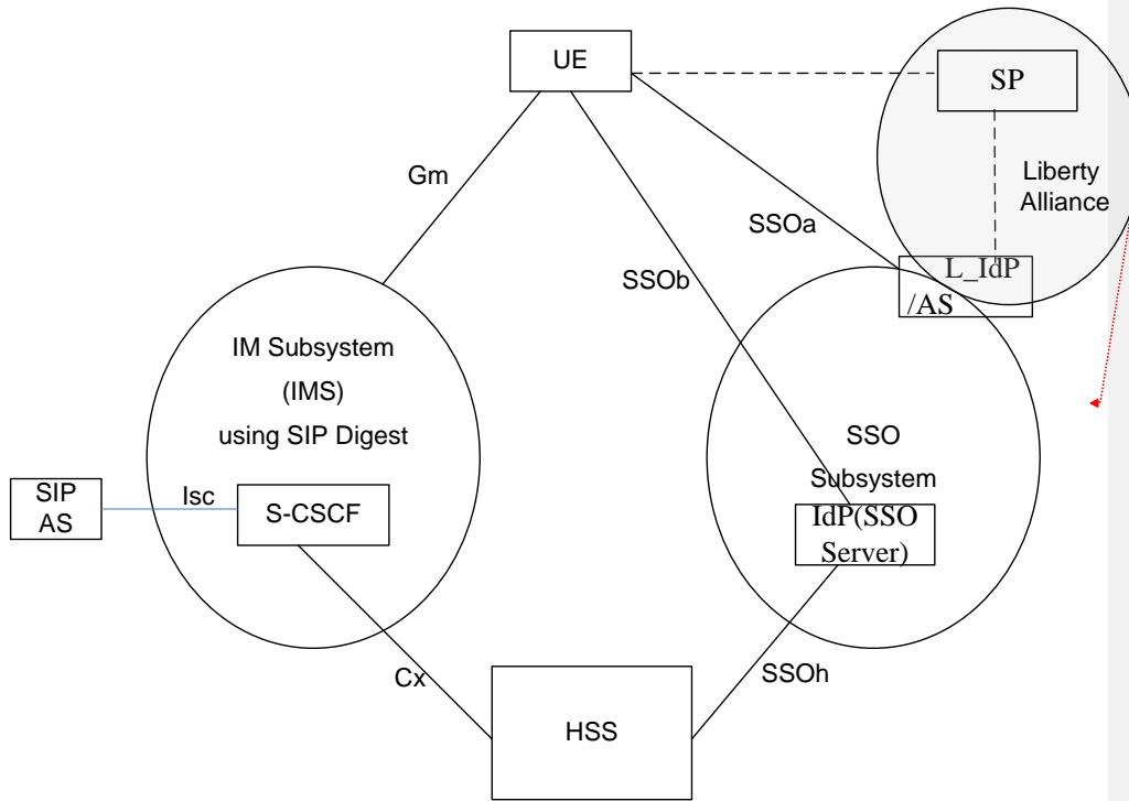
Figure 7.3-3: Architecture for interworking with Liberty Alliance that co-hosts AS and IdP (Liberty Alliance)
