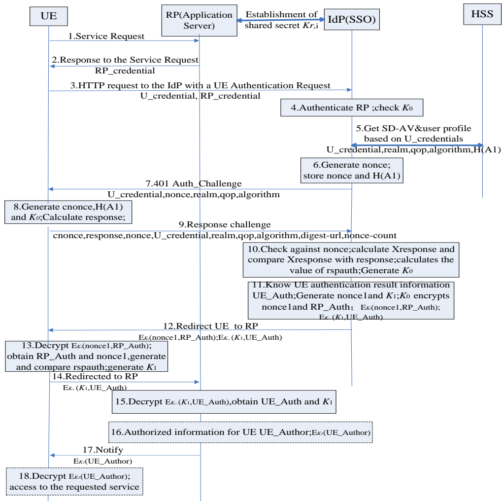
Figure 7.3-45 authentication process of SIP Digest-based SSO with the Common IMSSDALS Procedure
