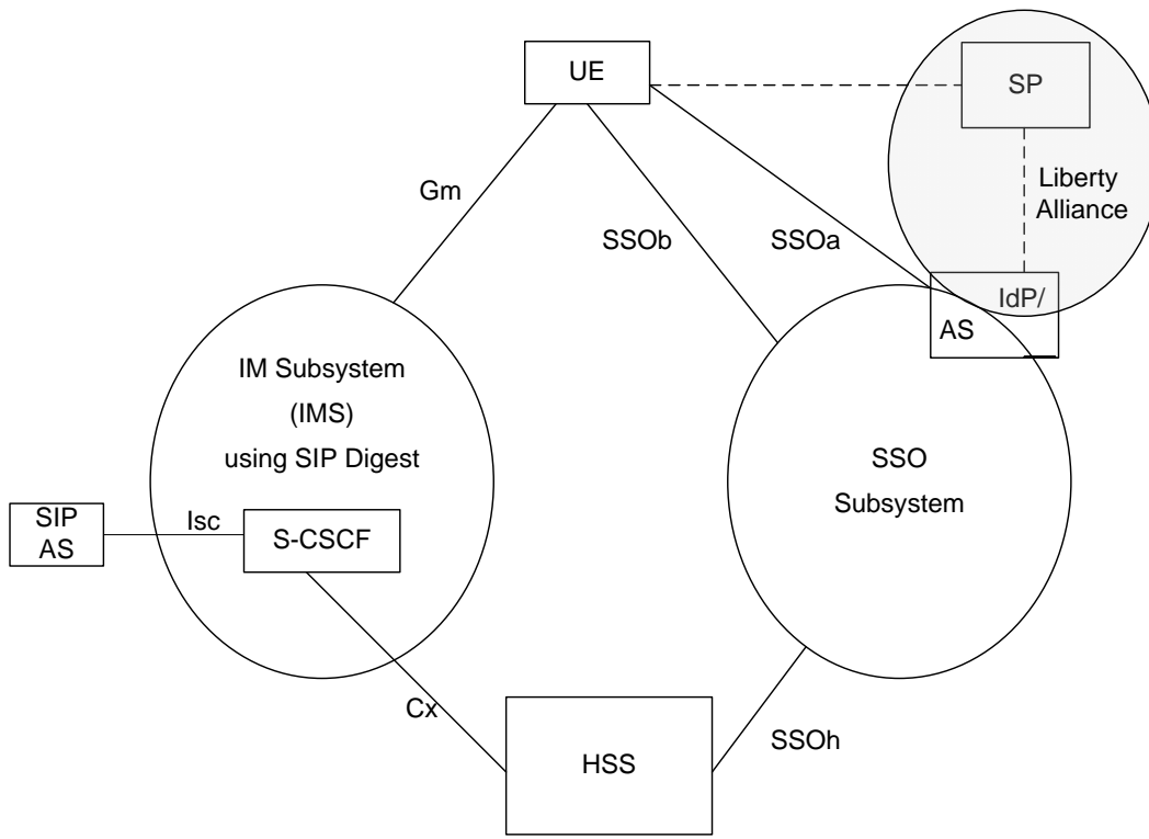
Figure 5.4-1: Relation of SIP Digest-based SSO with the Common IMS and interworking with Liberty Alliance
