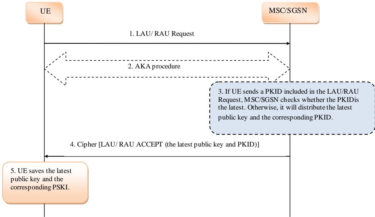
Figure 7.3.4.2.1: Distribution of public key information in GSM/GPRS
