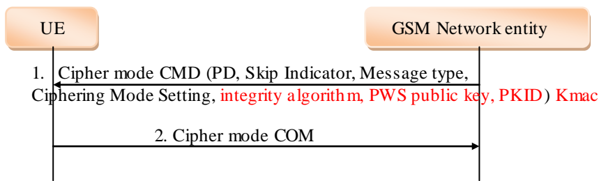
Figure 7.3.4.3.1: Distribution of public key information in GSM
