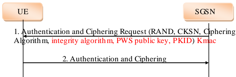
Figure 7.3.4.3.2: Distribution of public key information in GPRS
