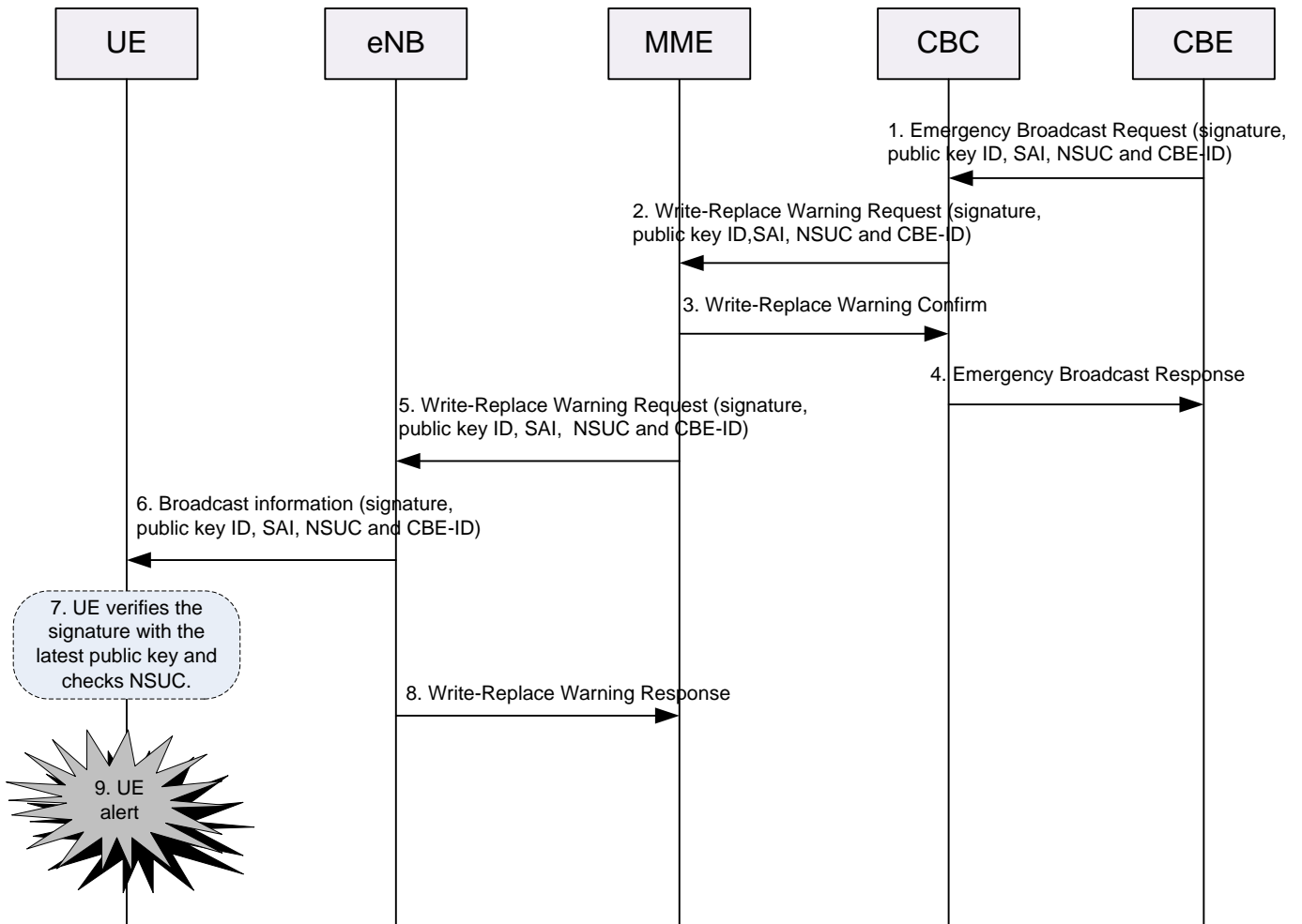
Figure 7.3.3.1 PWS Warning Notification procedure for LTE system
