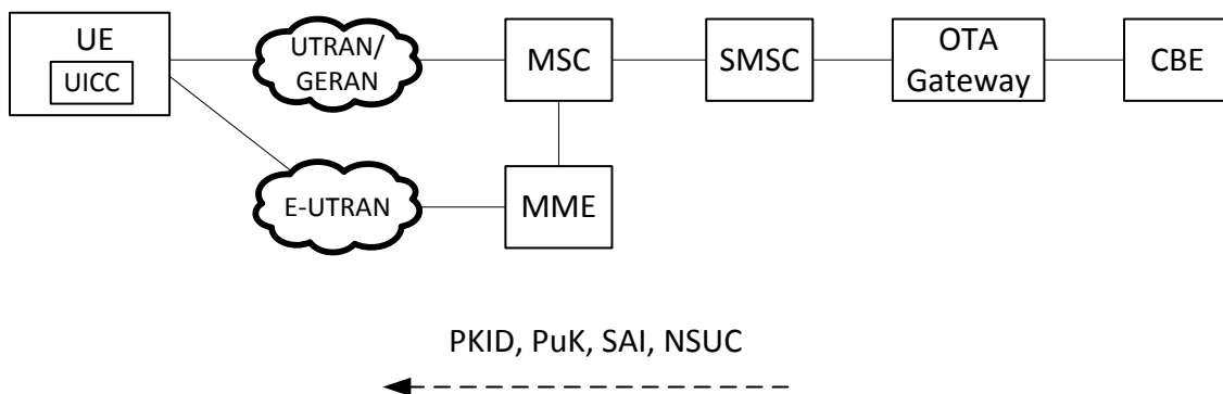
Figure 7.8.2 UICC OTA delivery of PWS key using SMS as transport bearer
