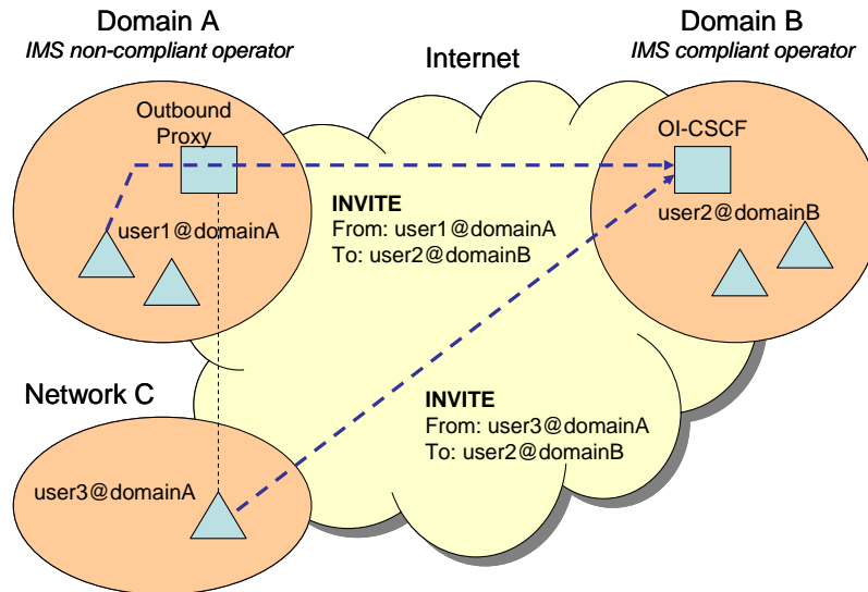
Figure 5.3-2: Non-IMS interconnection network architecture
