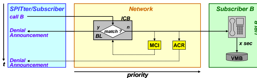
Figure 7.3-2: Simple Black List with Anonymous Call Rejection
