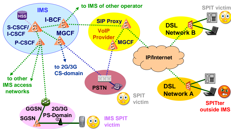
Figure 5.2-2: SPIT/UC source outside IMS
