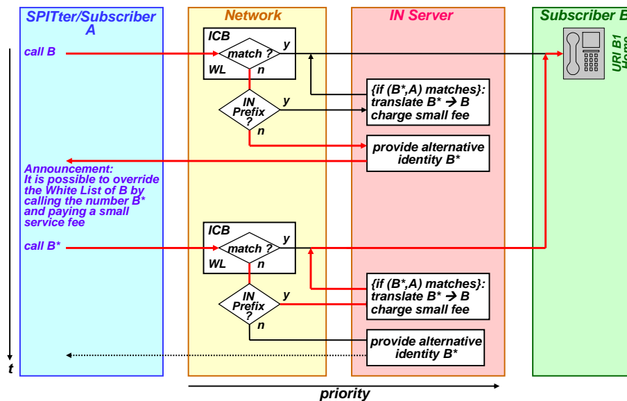
Figure 7.3-6: White List Consent Achievement by IN Server
