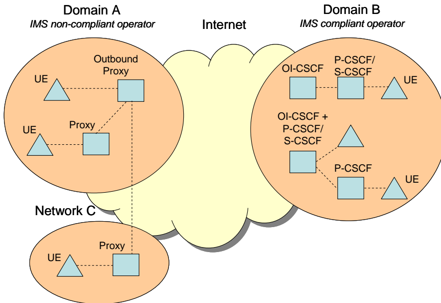
Figure 7.5-1: Non-IMS interconnection general architecture
