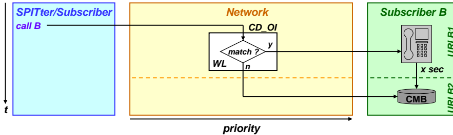
Figure 7.3-3: WhiteList with Consent Mailbox
