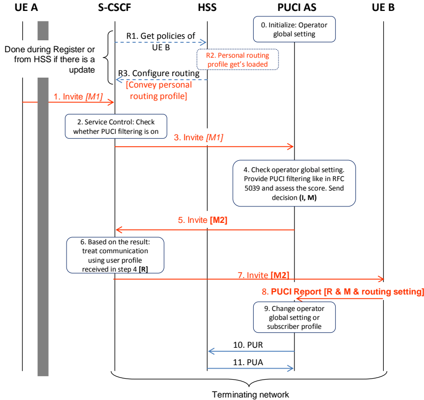
Figure 7.2-5: Simple PUCI service invocation.
