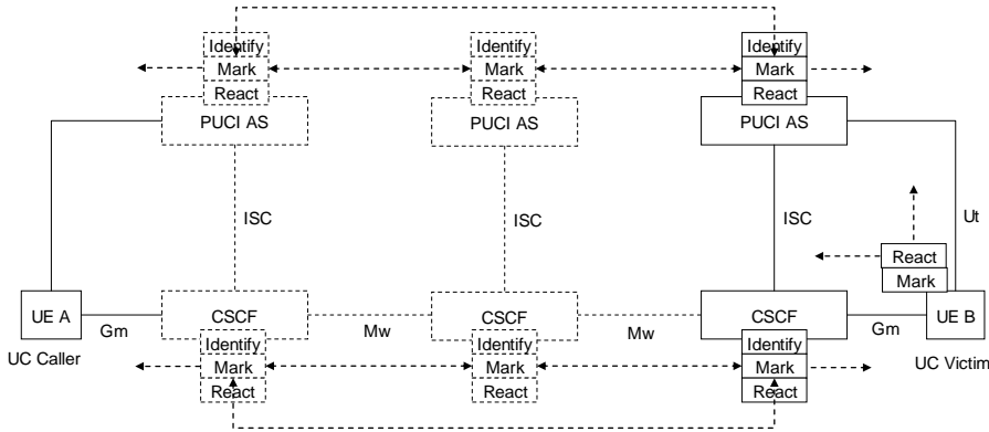
Figure 7.2-3: Requirements represented in figure.
