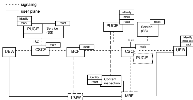
Figure 9.1-1: Mapping of PUCI functionality to IMS architecture.
