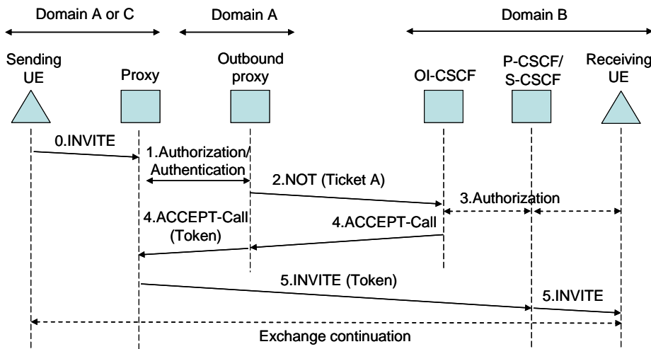
Figure 7.5-3: Protocol exchange when a shared secret is available between domains
