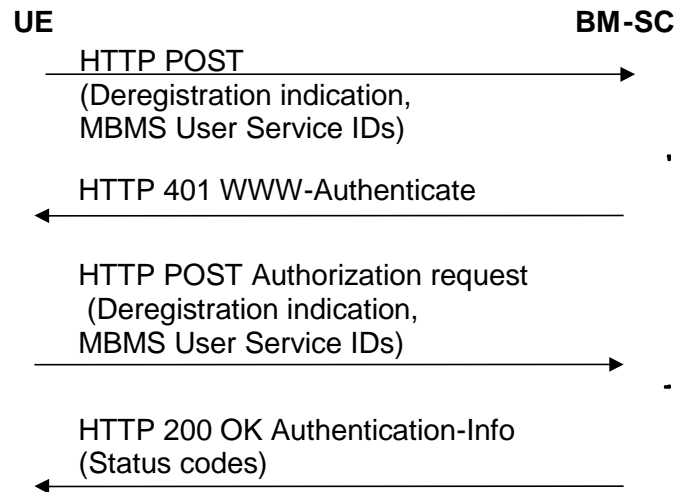
Figure 6.0B: MBMS User Service Deregistration procedure
