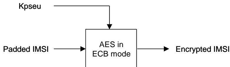
Figure 8: Encrypted IMSI generation
