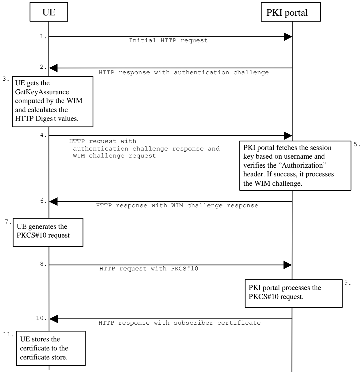
Figure 2: Certificate request using PKCS#10 with HTTP Digest Authentication
