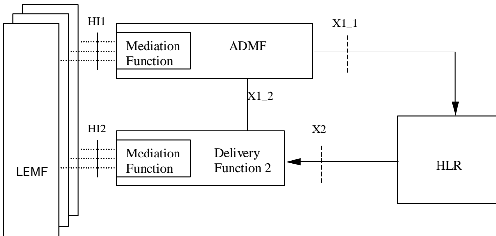
Figure 1c: HLR Intercept configuration
