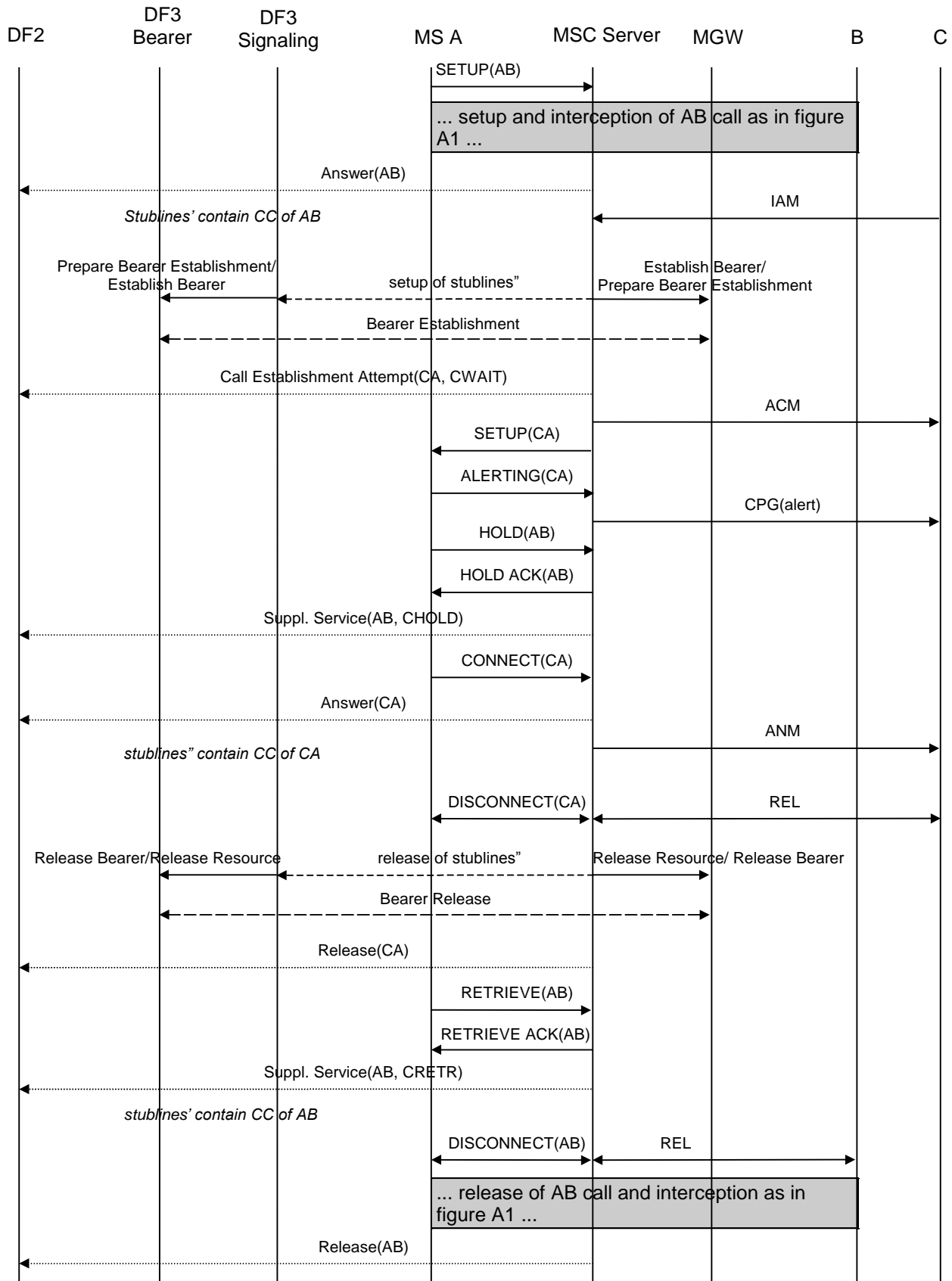
Figure A.4: Interception of call hold / call waiting - stblines per target call
