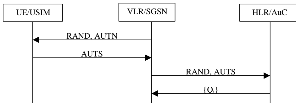
Figure 12: Resynchronisation mechanism
