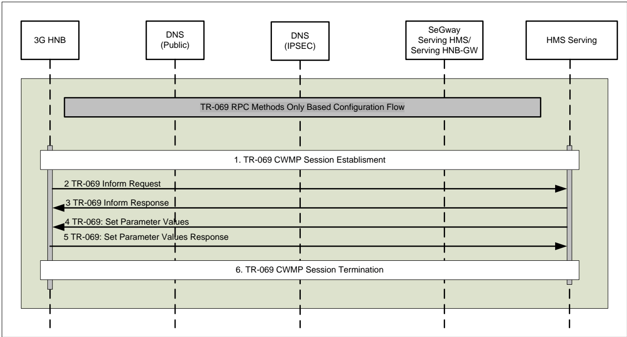
Figure 6: TR-069 RPC Methods Only Based Configuration Flow
