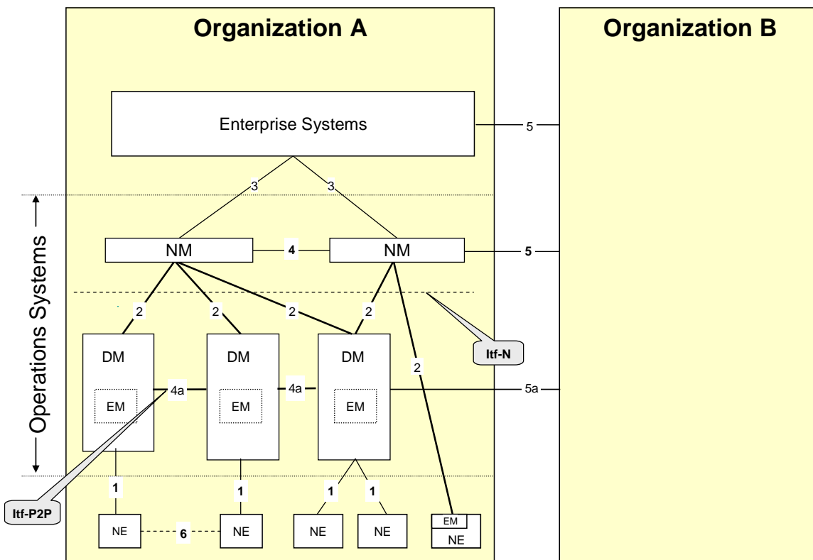
Figure 14: Management reference model
