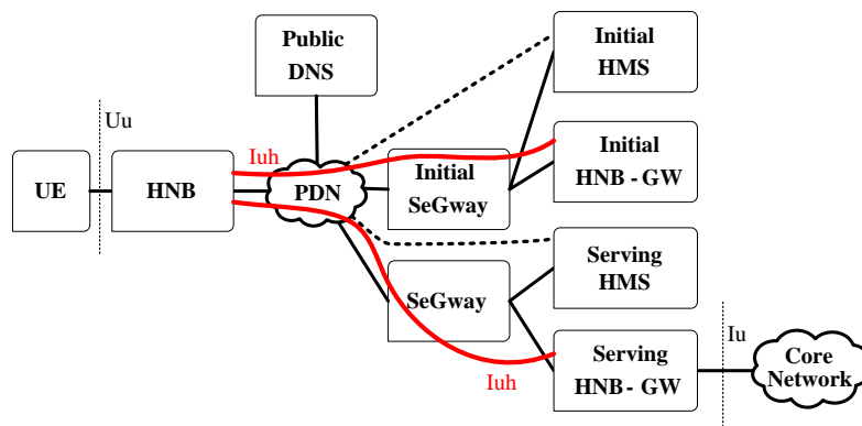
Figure 4: Iuh reference model
