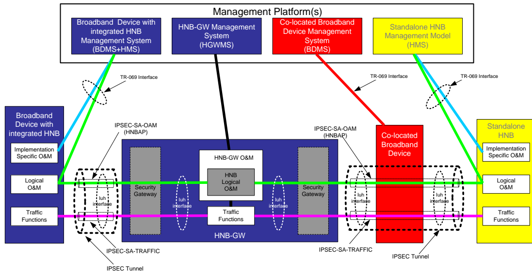
Figure 1: HNB/HNB-GW architecture with OAM interfaces
