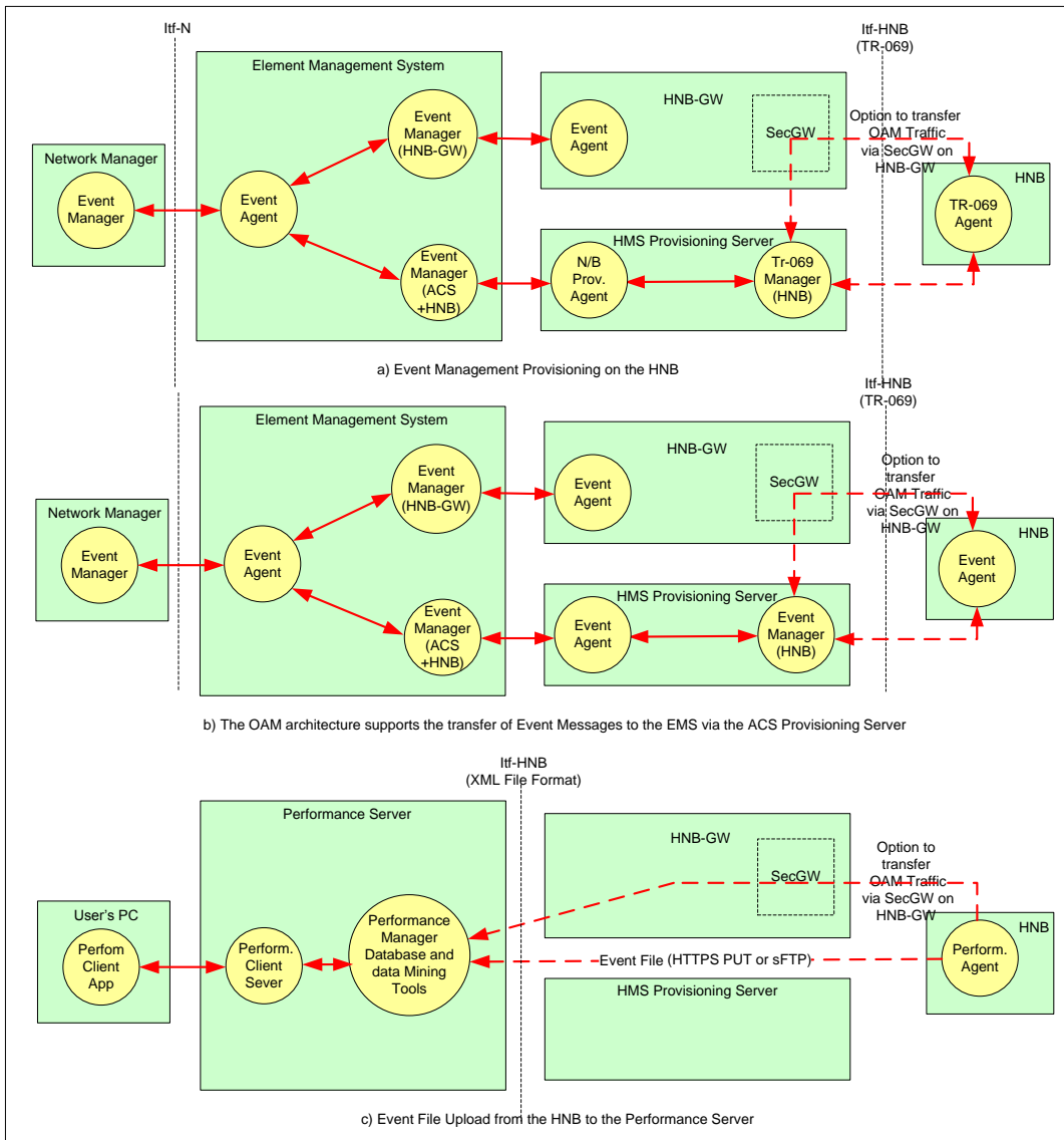
Figure 13: HNB/HNB-GW Fault Management
