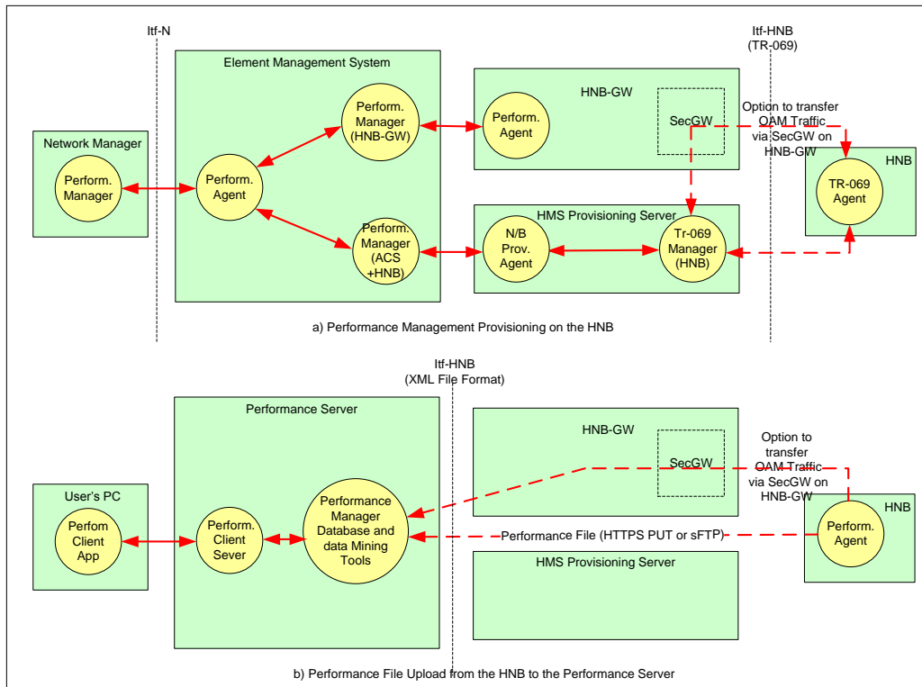
Figure 12: HNB/HNB-GW Performance Management
