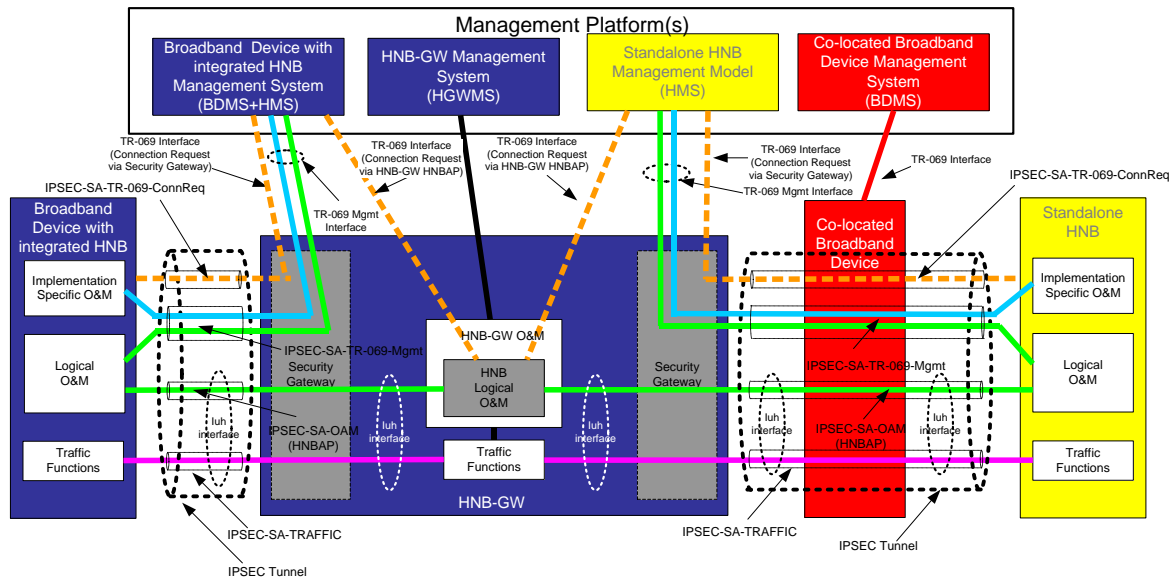
Figure 2: HNB/HNB-GW architecture with OAM interfaces via IPSEC Tunnel
