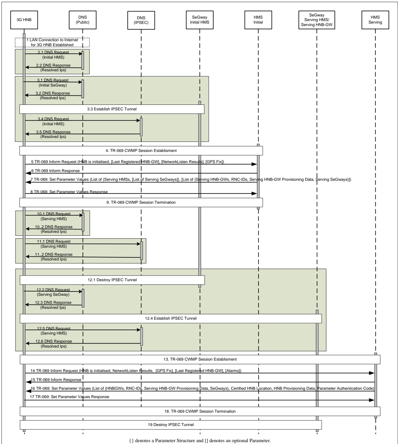
Figure 9: HNB-GW Discovery Procedure
