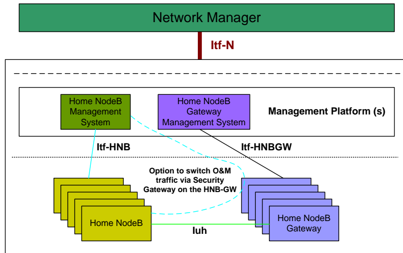
Figure 3: 3GPP HNB Radio Network Management Interfaces
