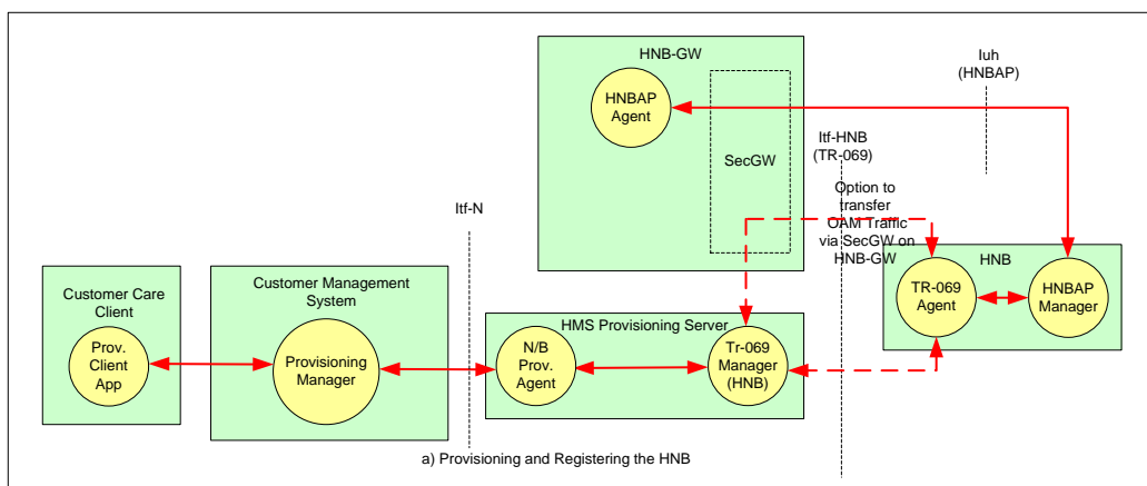
Figure 8: HNB/HNB-GW Configuration Management
