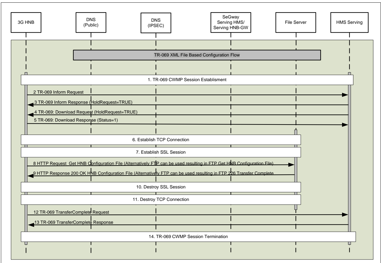
Figure 7: TR-069 XML File Based Configuration Flow
