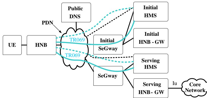
Figure 5: TR069 based provisioning
