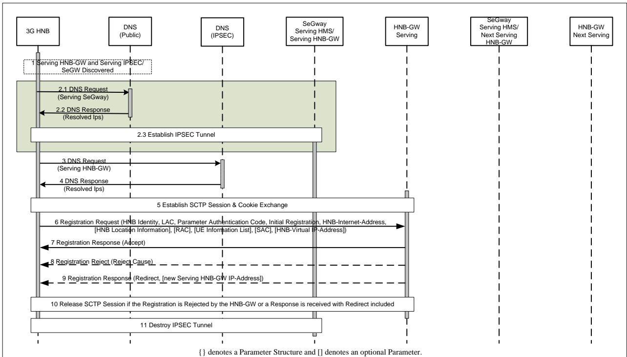
Figure 10: HNB Registration Procedure
