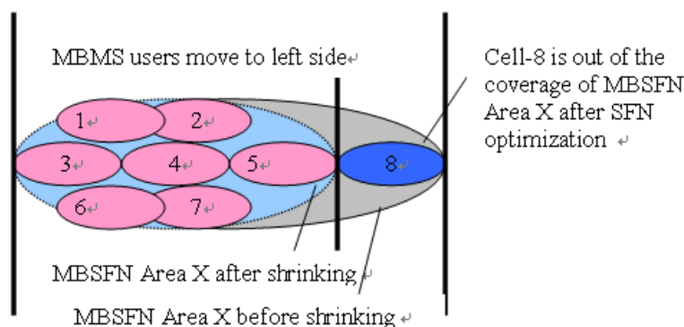
Figure 1: An example of MBSFN Area optimization.
