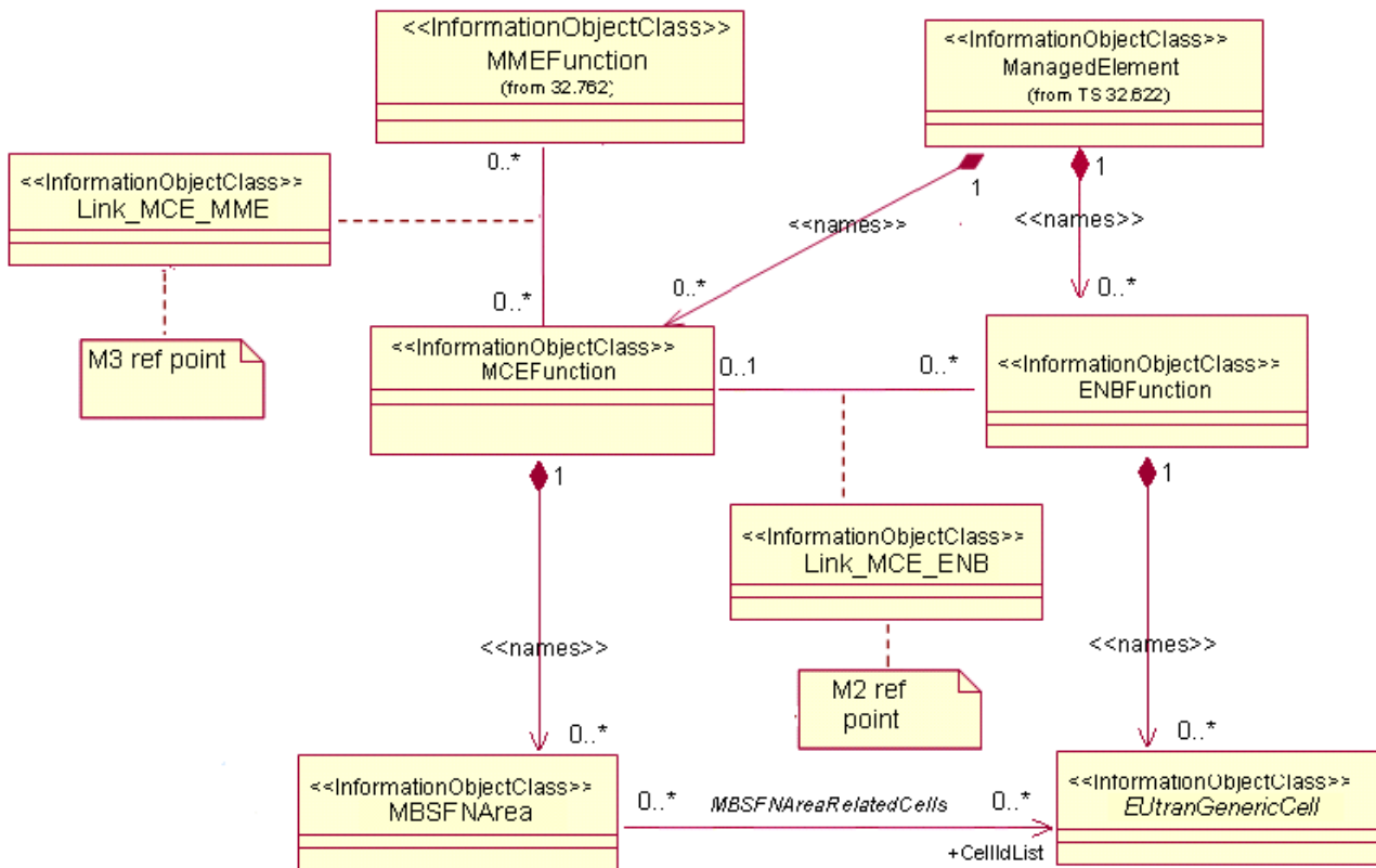
Figure 6.2.1.6: MBMS view of E-UTRAN NRM 2
