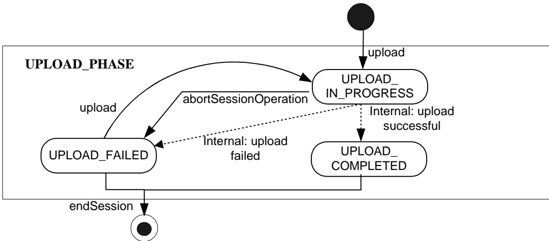
Figure 9.2.1: Substate Machine - UPLOAD_PHASE
