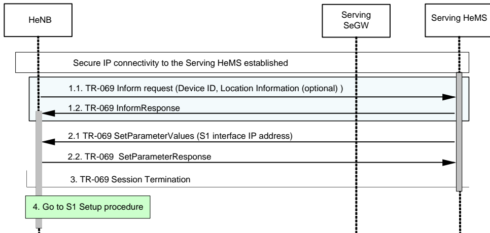
Figure 5-2: Procedure for HeNB registration with Serving HeMS
