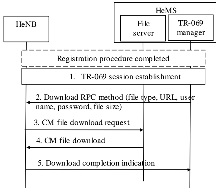
Figure 5-3 HeNB configuration using file download procedure
