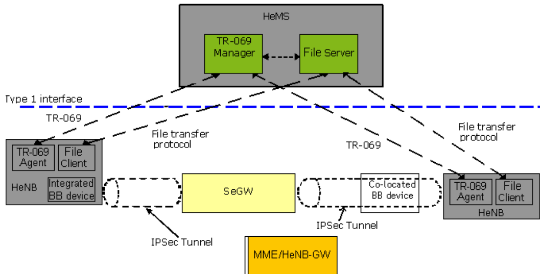
Figure 0-1: HeNB Management Architecture
