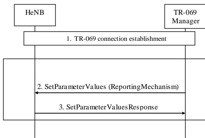
Figure 5-6 : Alarm Reporting Mechanism Configuration
