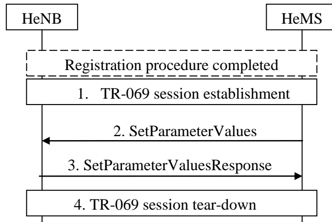
Figure 5-4 HeNB configuration procedure using RPC SetParameterValues method
