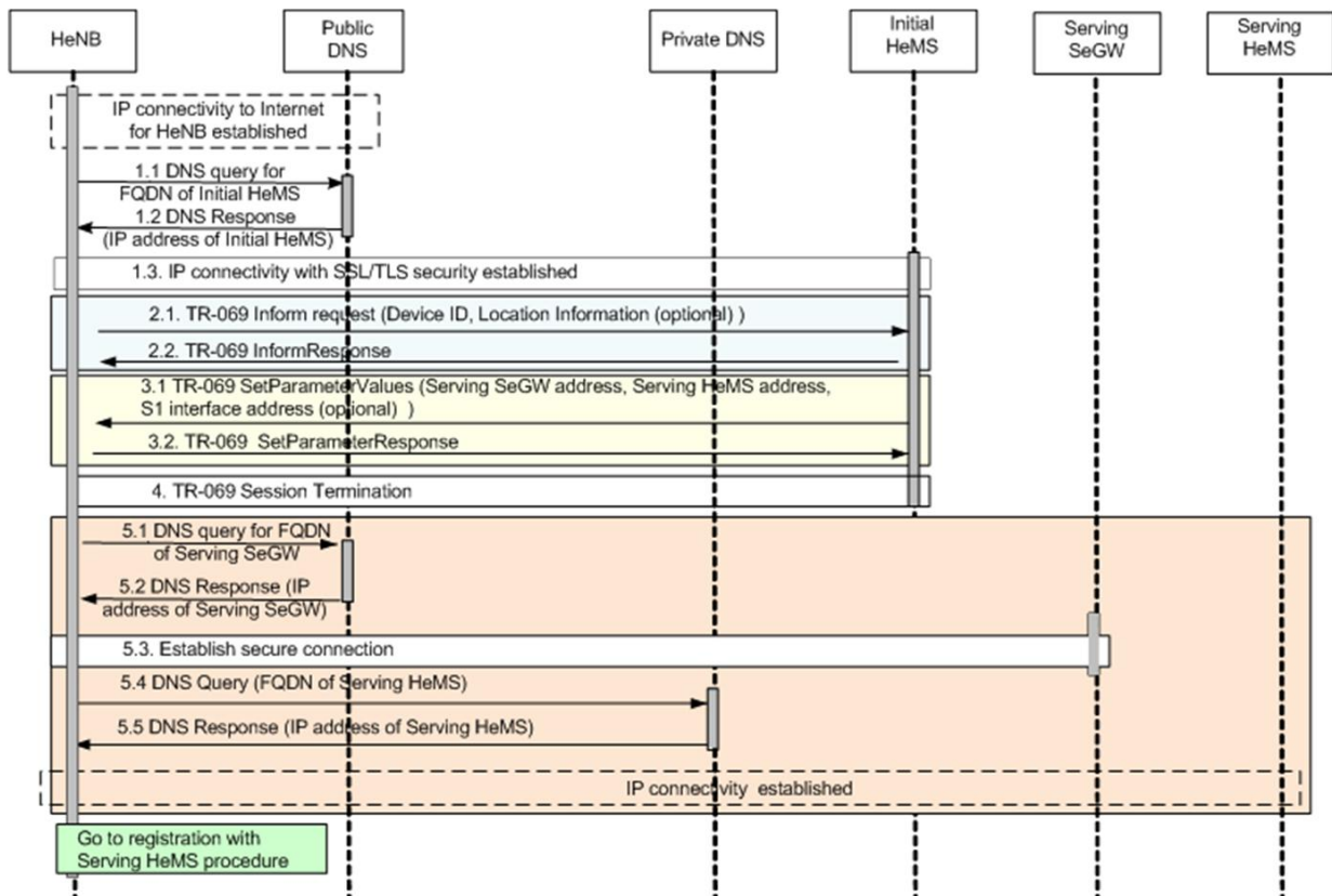
Figure 5-1 Serving HeMS Discovery via Initial HeMS accessible on the public internet
