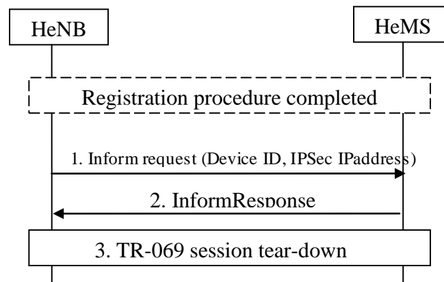
Figure 5-5 IP address change notification procedure
