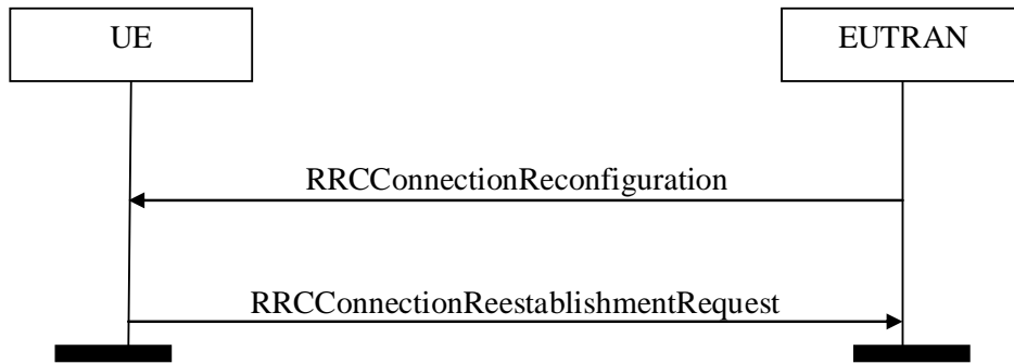
Figure12: RRC connection reconfiguration, failure
