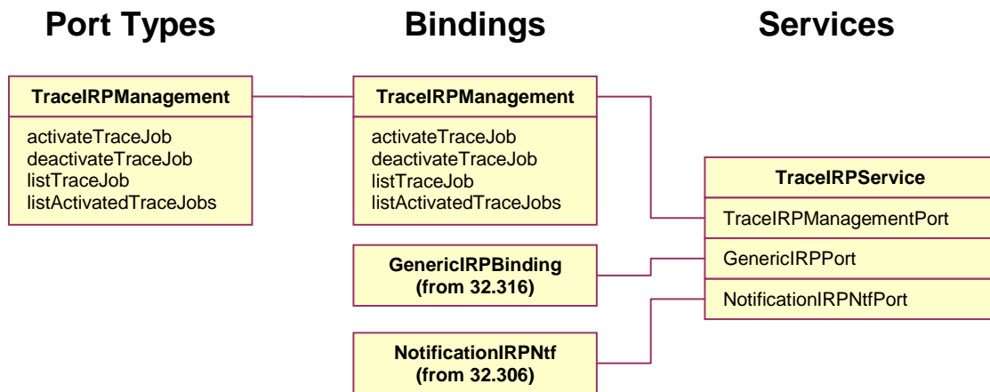
Figure C.3.2: Trace Management IRP SOAP Solution Set WSDL structure
